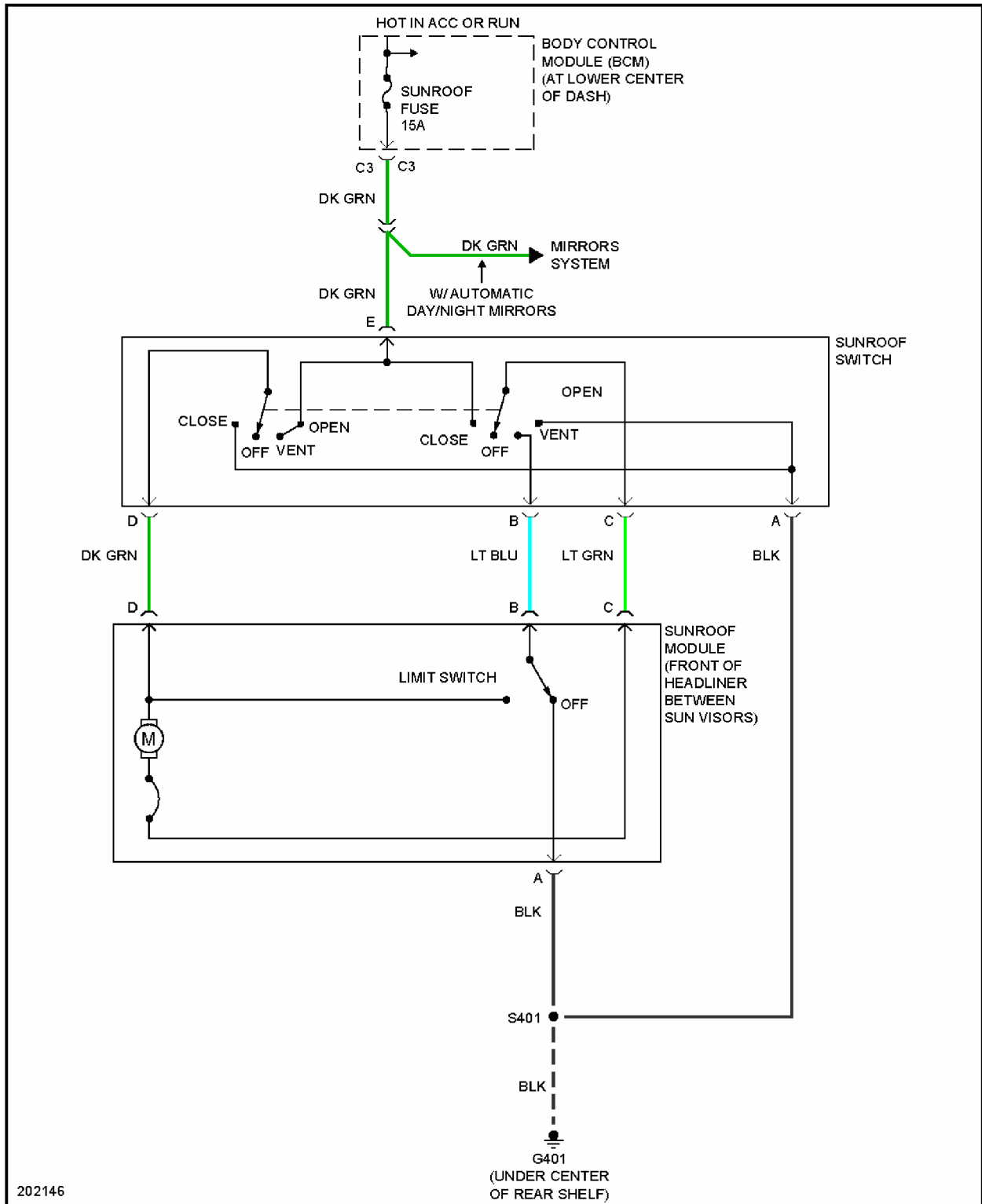
Fig. 47: Power Top/Sunroof Circuit
