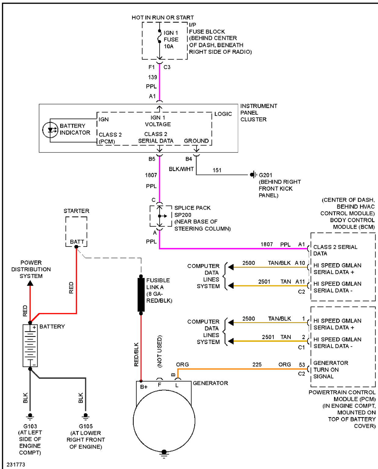
Fig. 42: Charging Circuit
