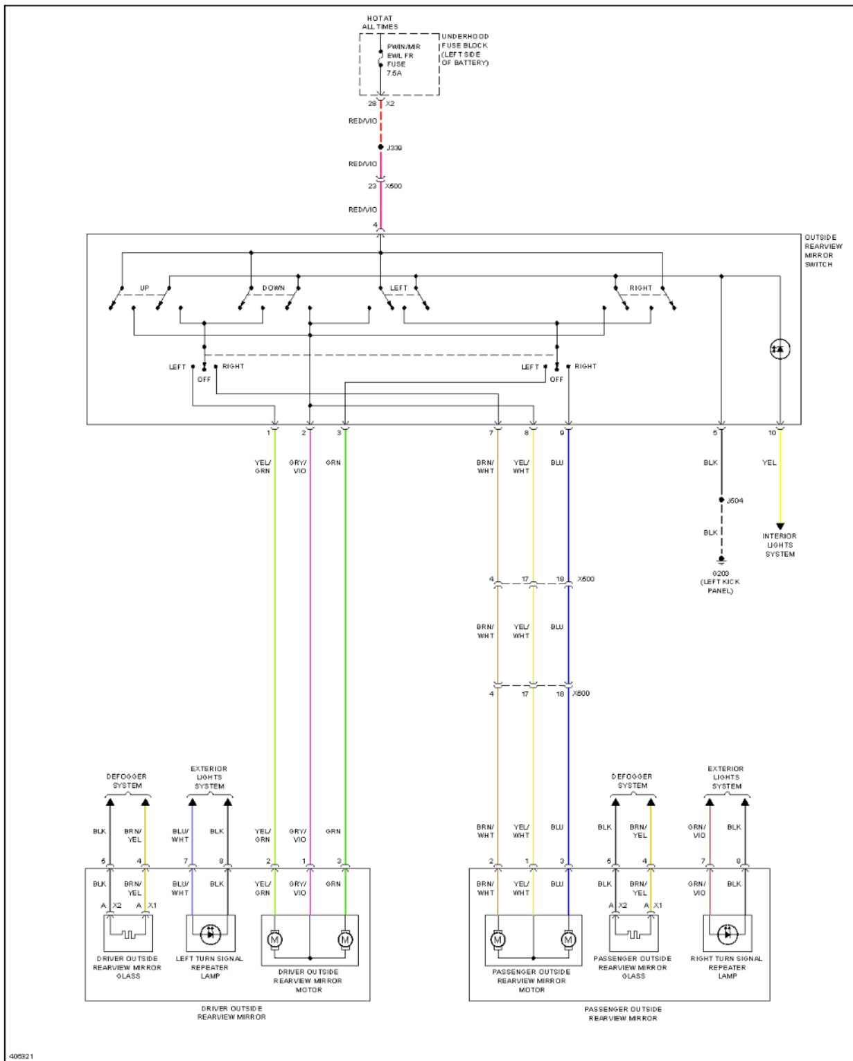
Fig. 101: Power Mirrors Circuit
