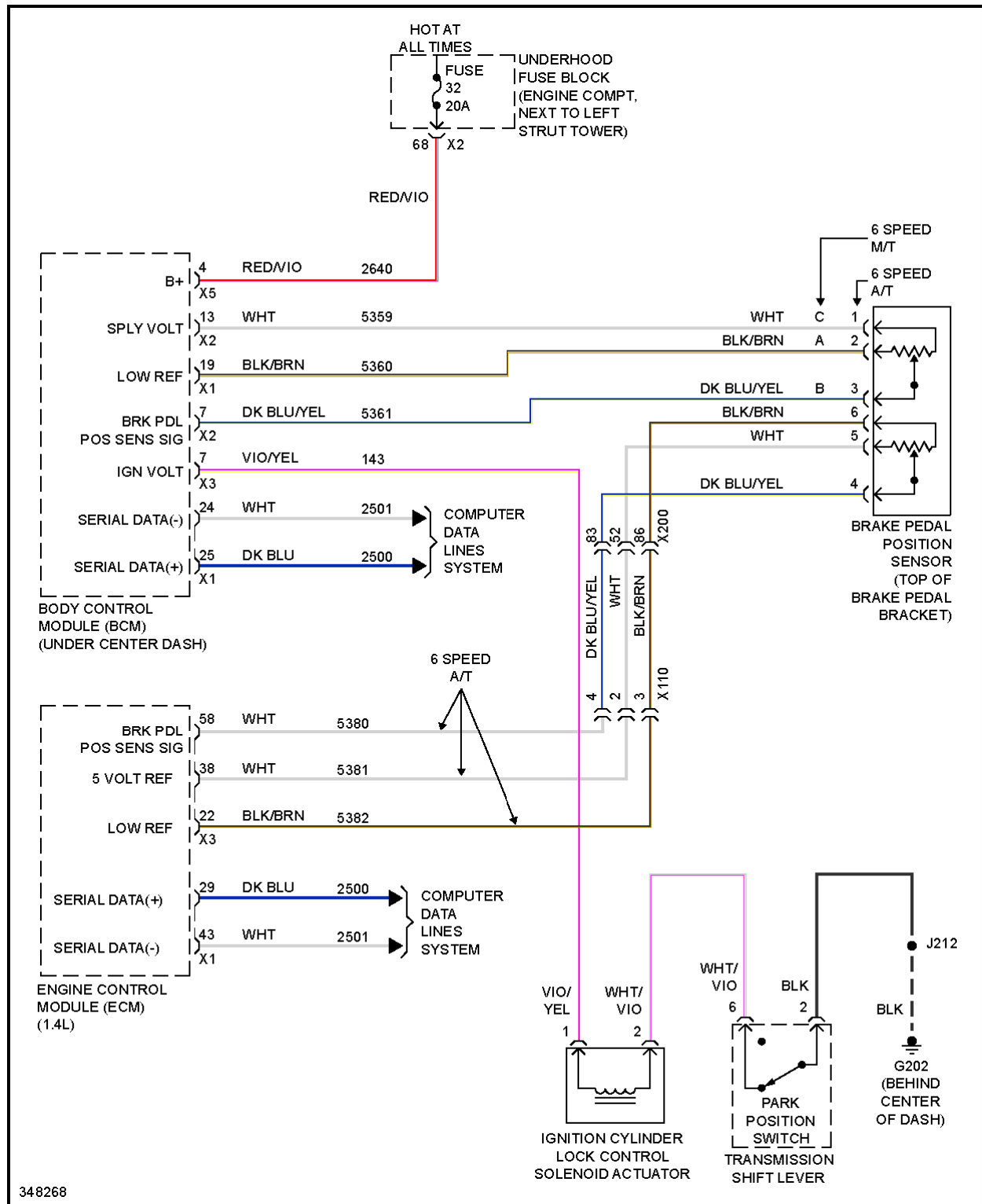
Fig. 66: Ignition Lock Solenoid Circuit
