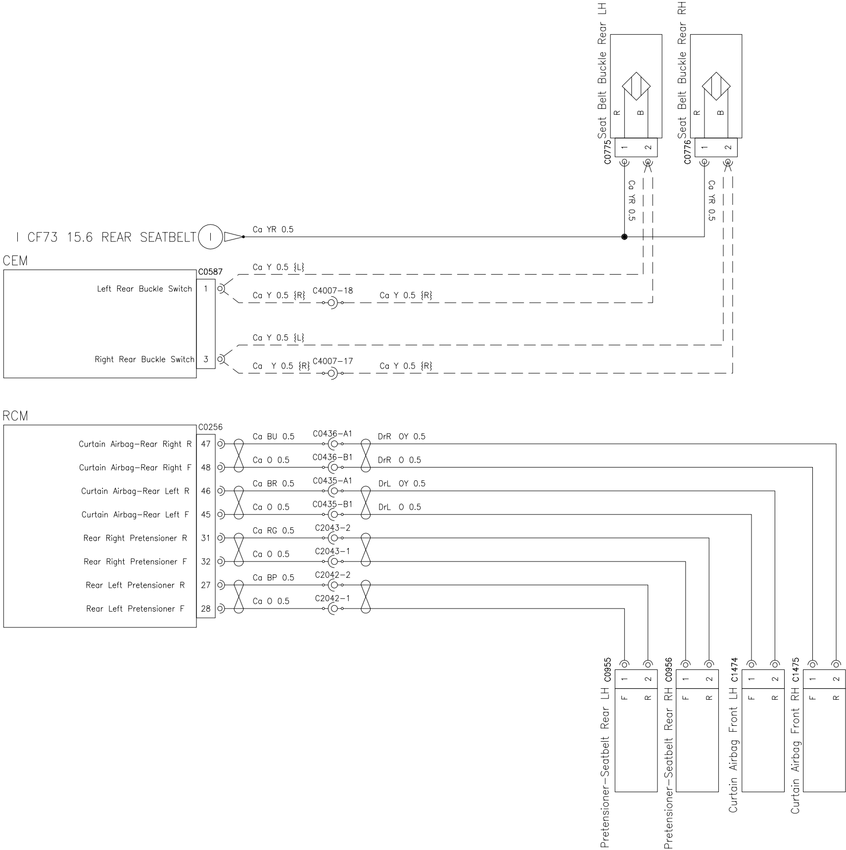
Supplementary Restraint System Rear Occupants - Sensors, Airbags and Actuators
