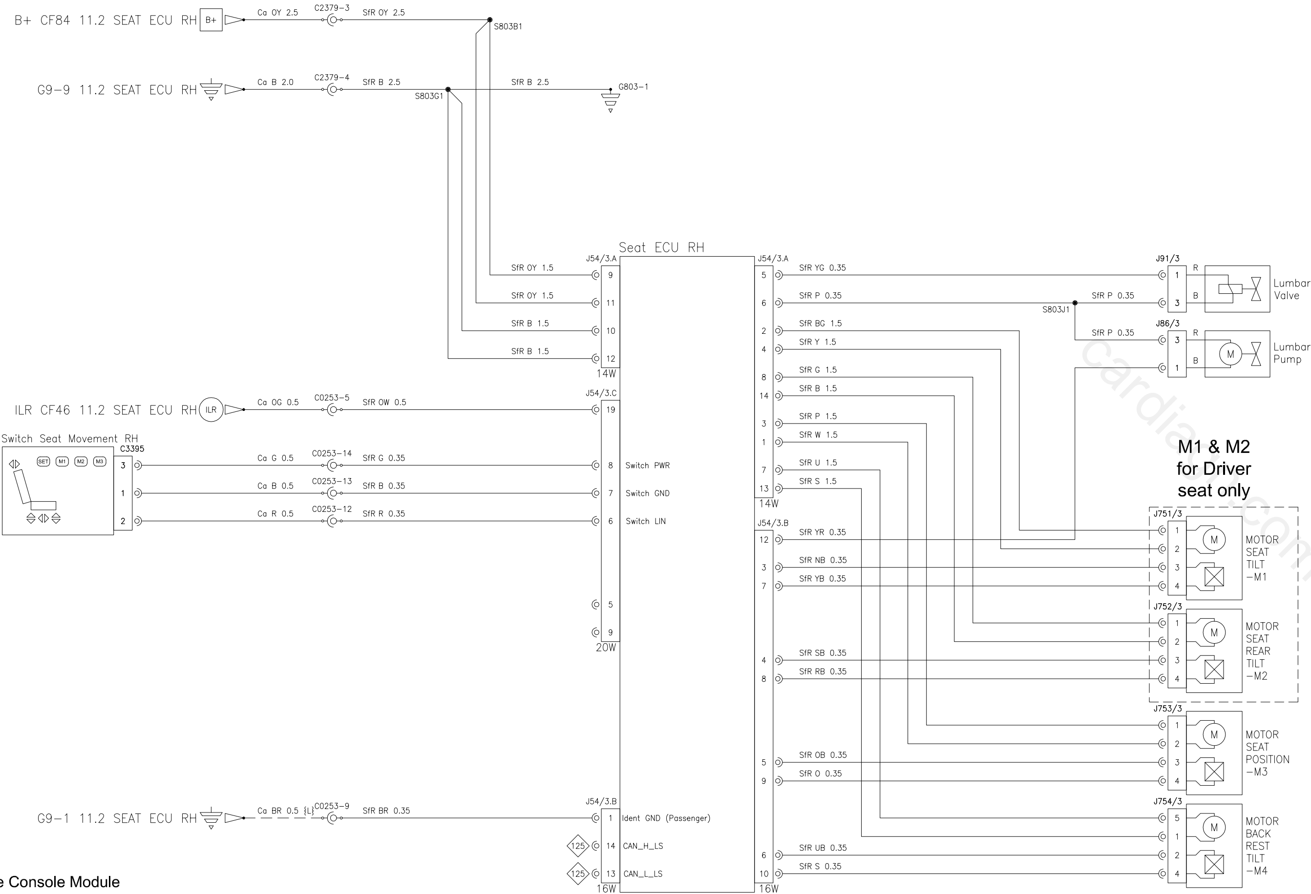
Seat Adjustment Front Right
