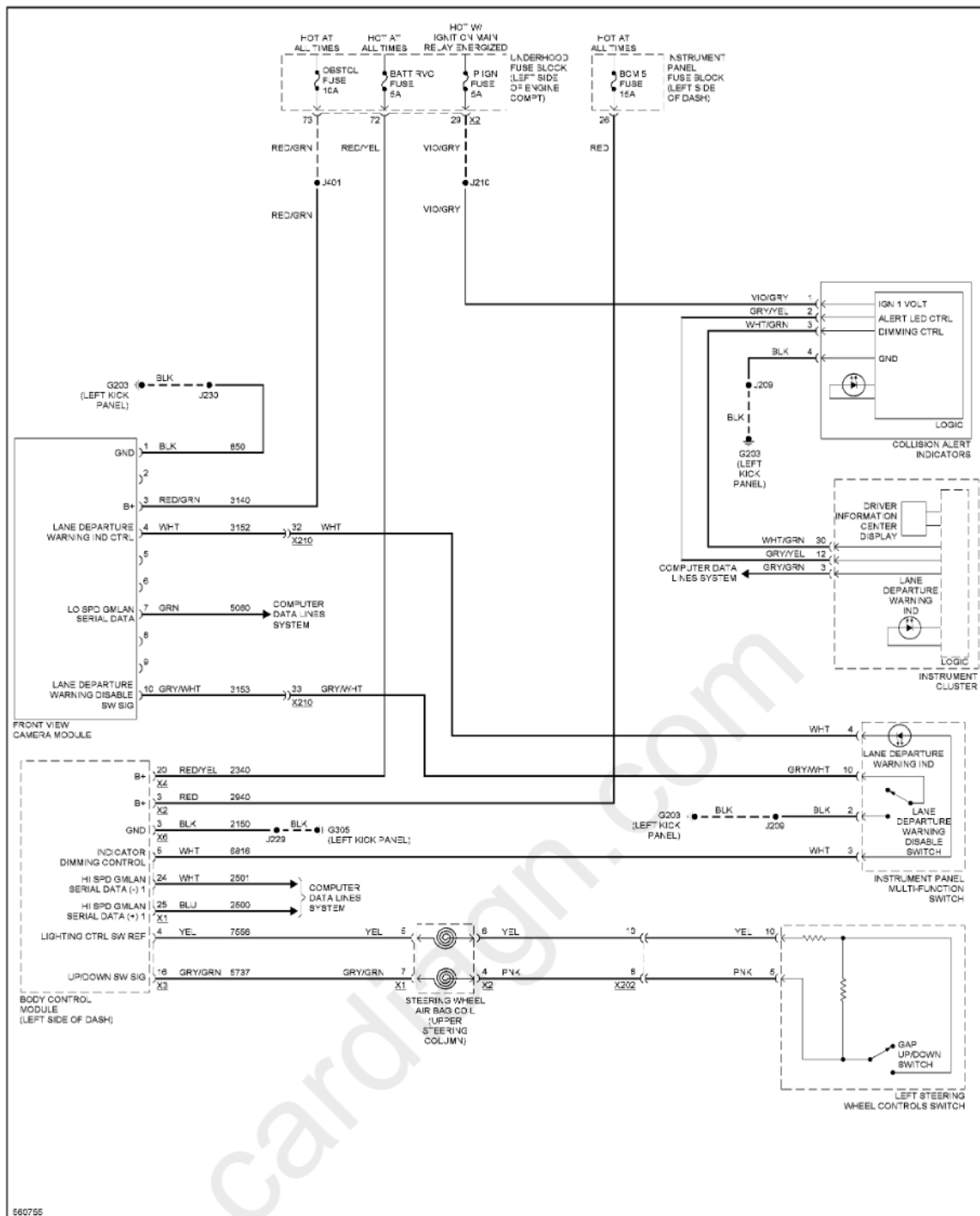
Fig. 76: Lane Departure Warning Circuit
