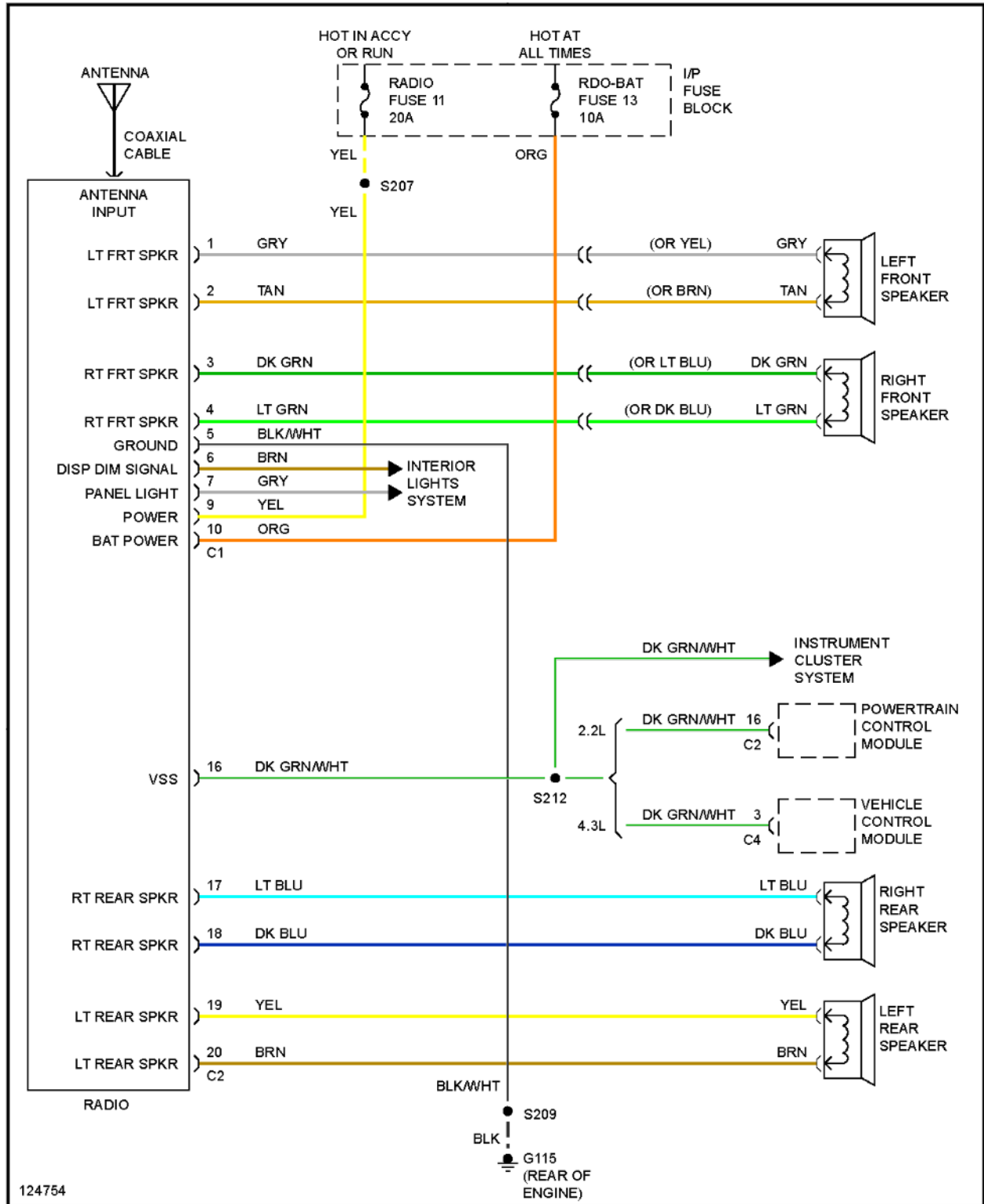
Fig. 30: 4-Speaker System Circuit
