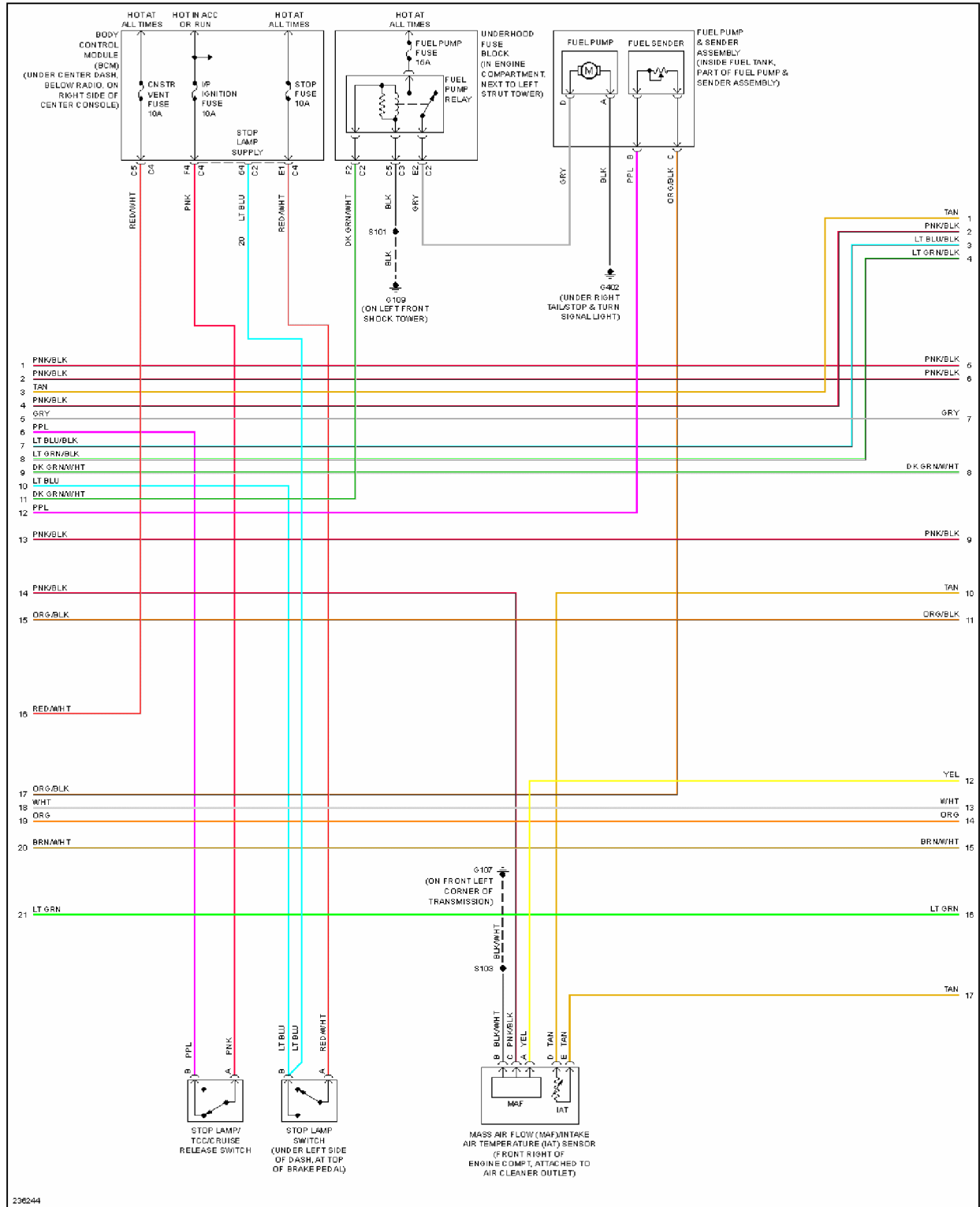
Fig. 18: 2.2L VIN F, Engine Performance Circuit (3 of 4)
