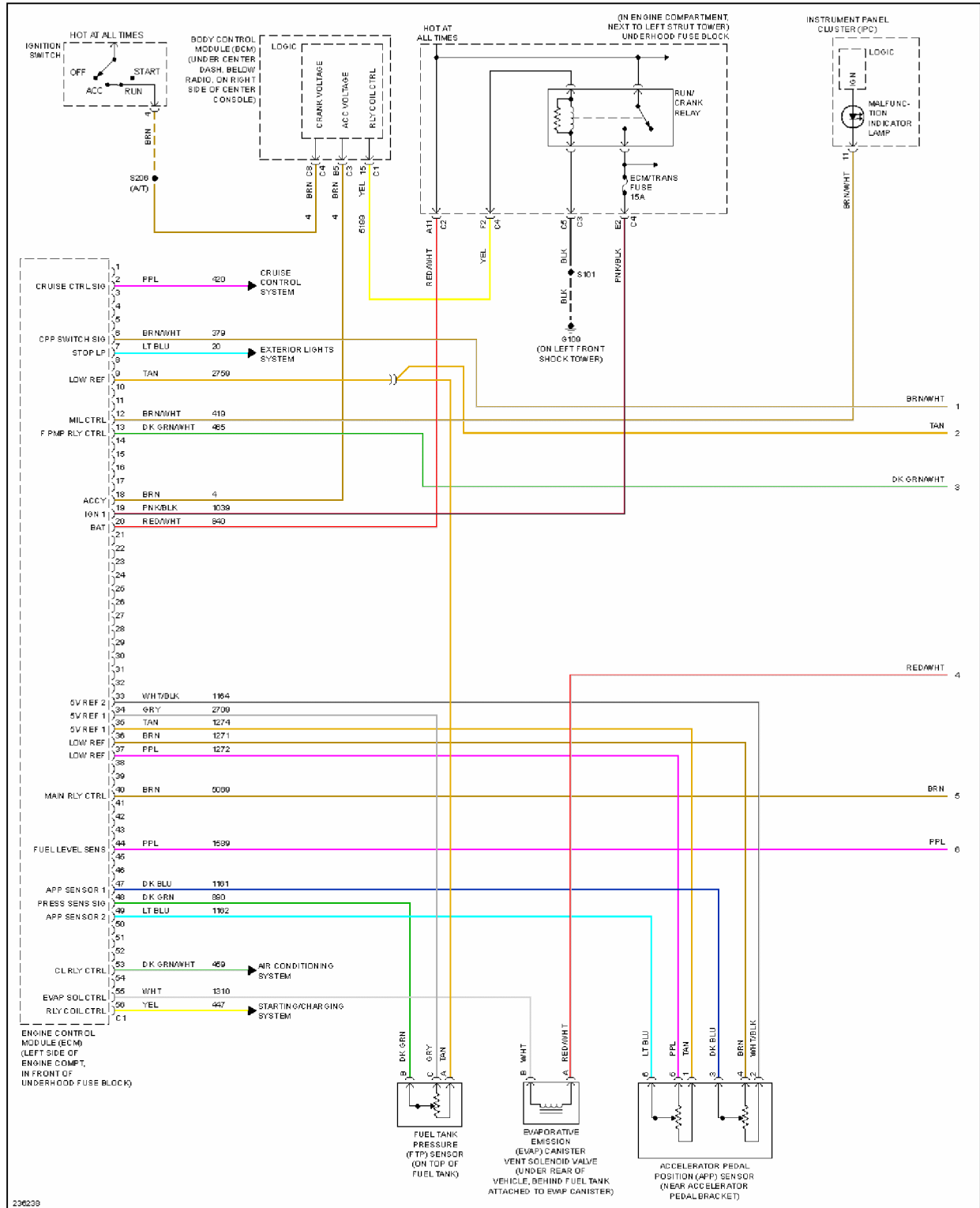
Fig. 20: 2.4L VIN B, Engine Performance Circuit (1 of 4)
