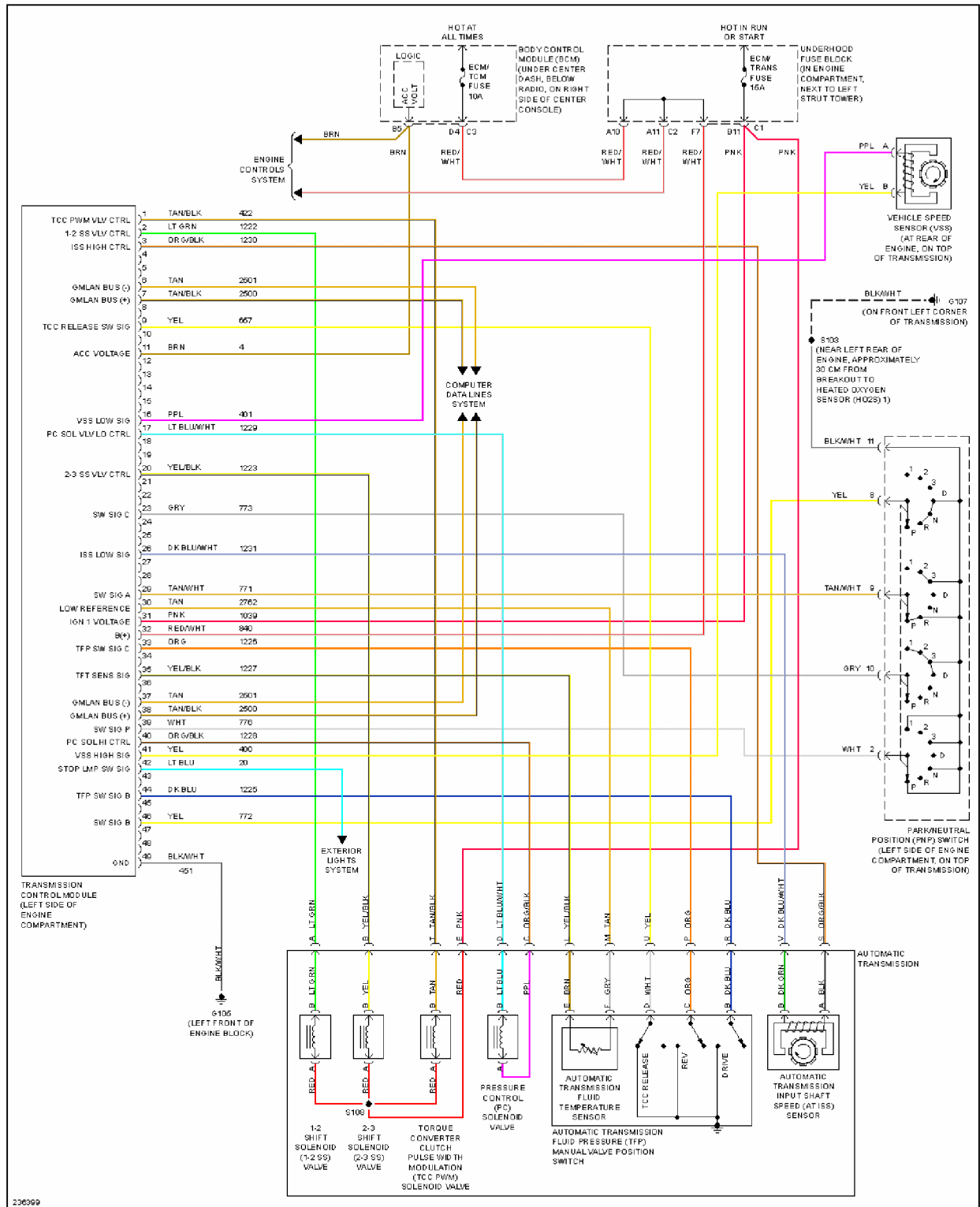
Fig. 53: A/T Circuit
