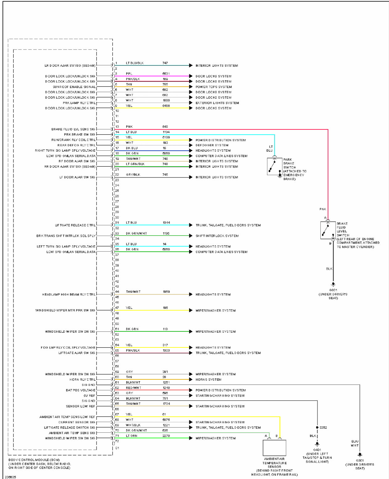
Fig. 7: Body Control Modules Circuit (1 of 4)
