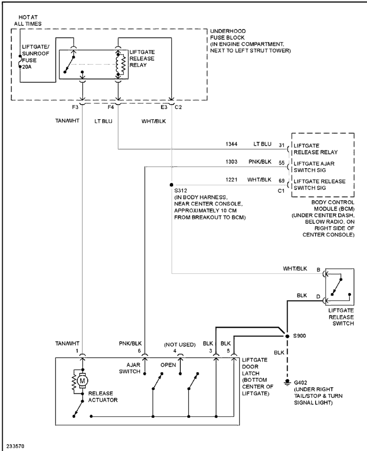
Fig. 55: Liftgate Release Circuit
