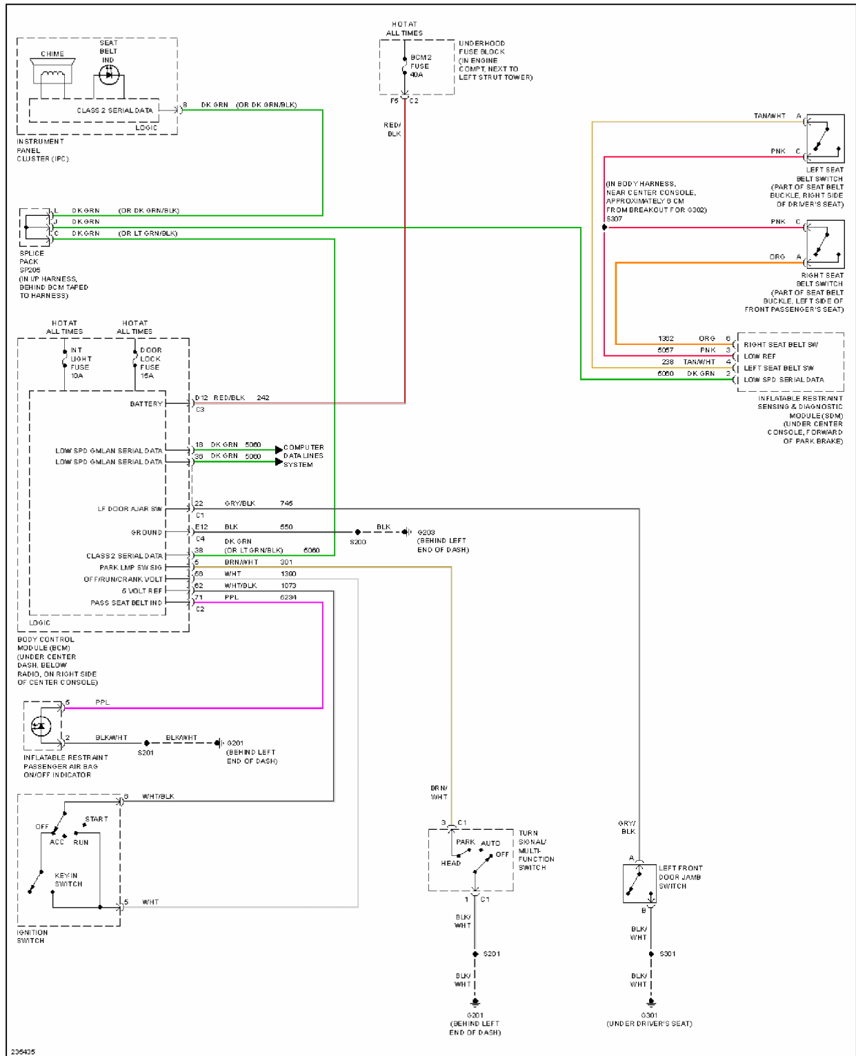
Fig. 56: Warning Systems Circuit
