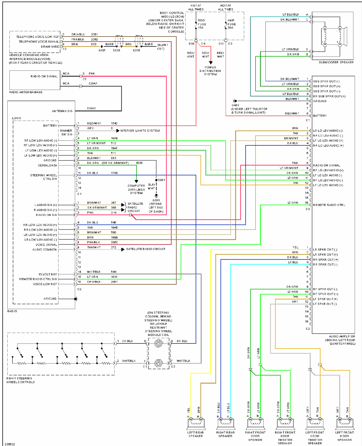
Fig. 45: Radio Circuit, W/ Amplifier
