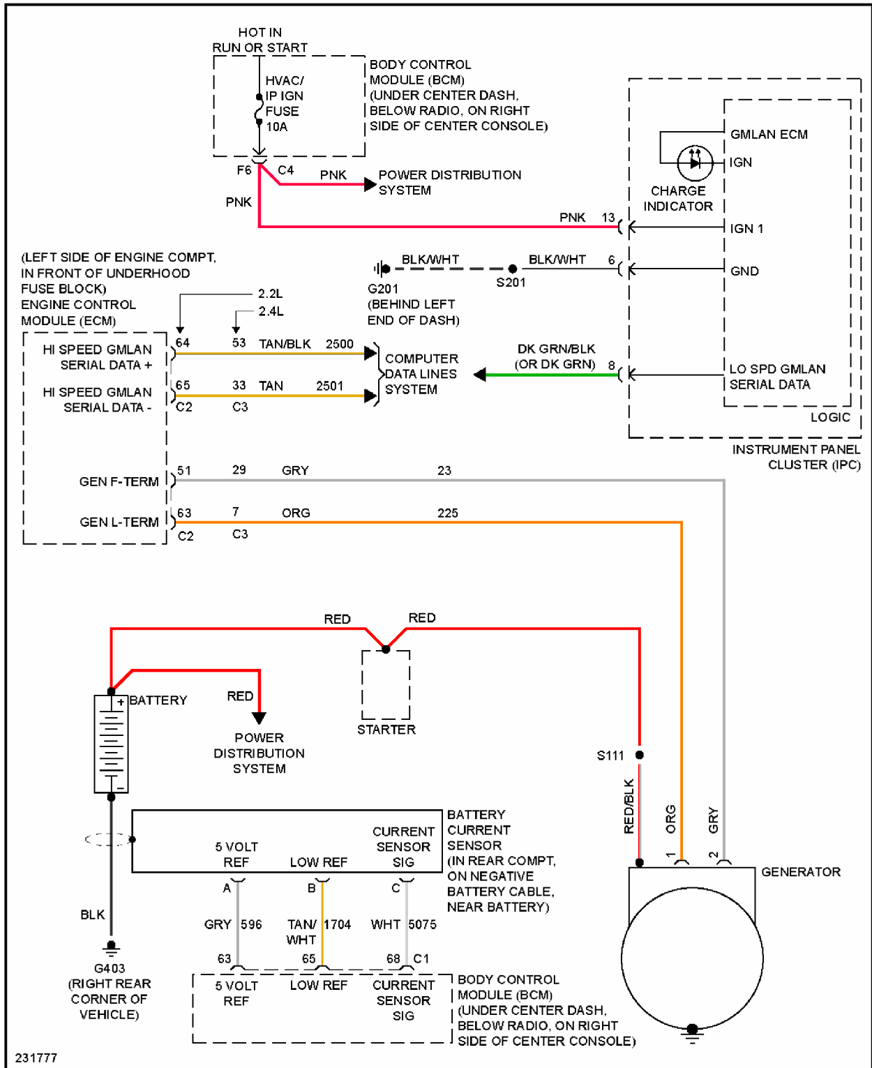
Fig. 49: Charging Circuit
