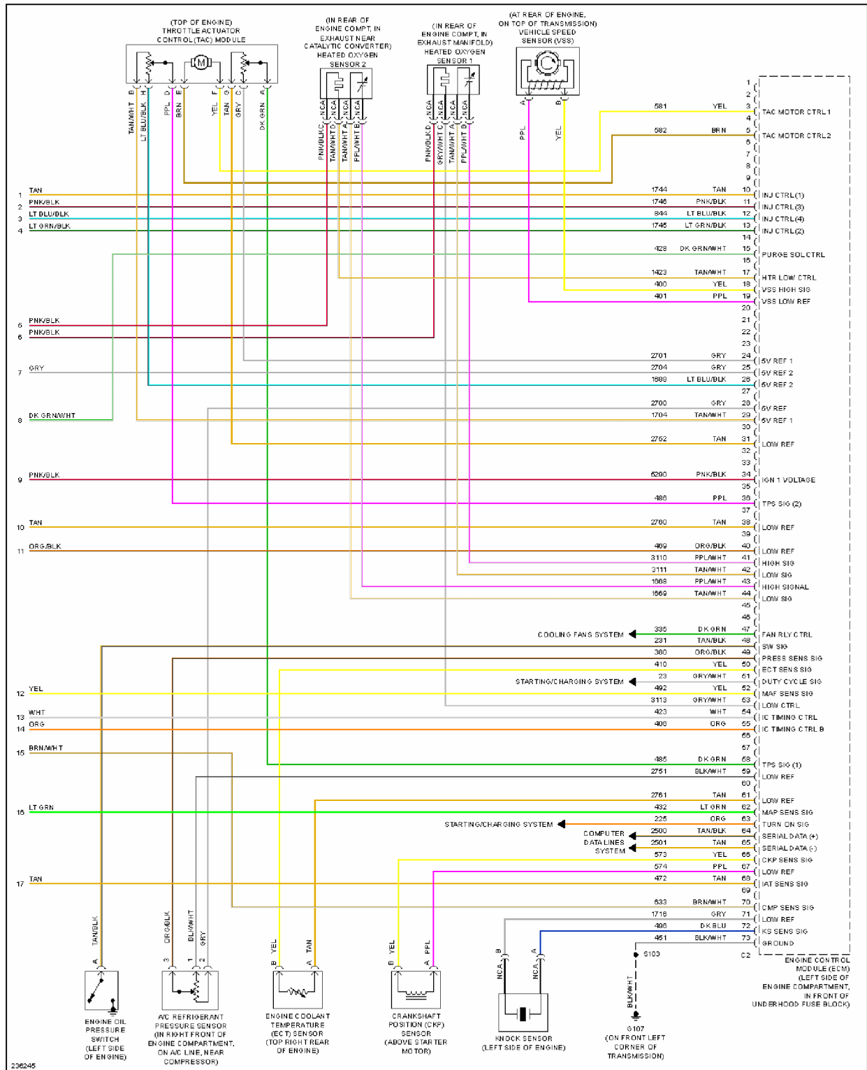
Fig. 19: 2.2L VIN F, Engine Performance Circuit (4 of 4)
