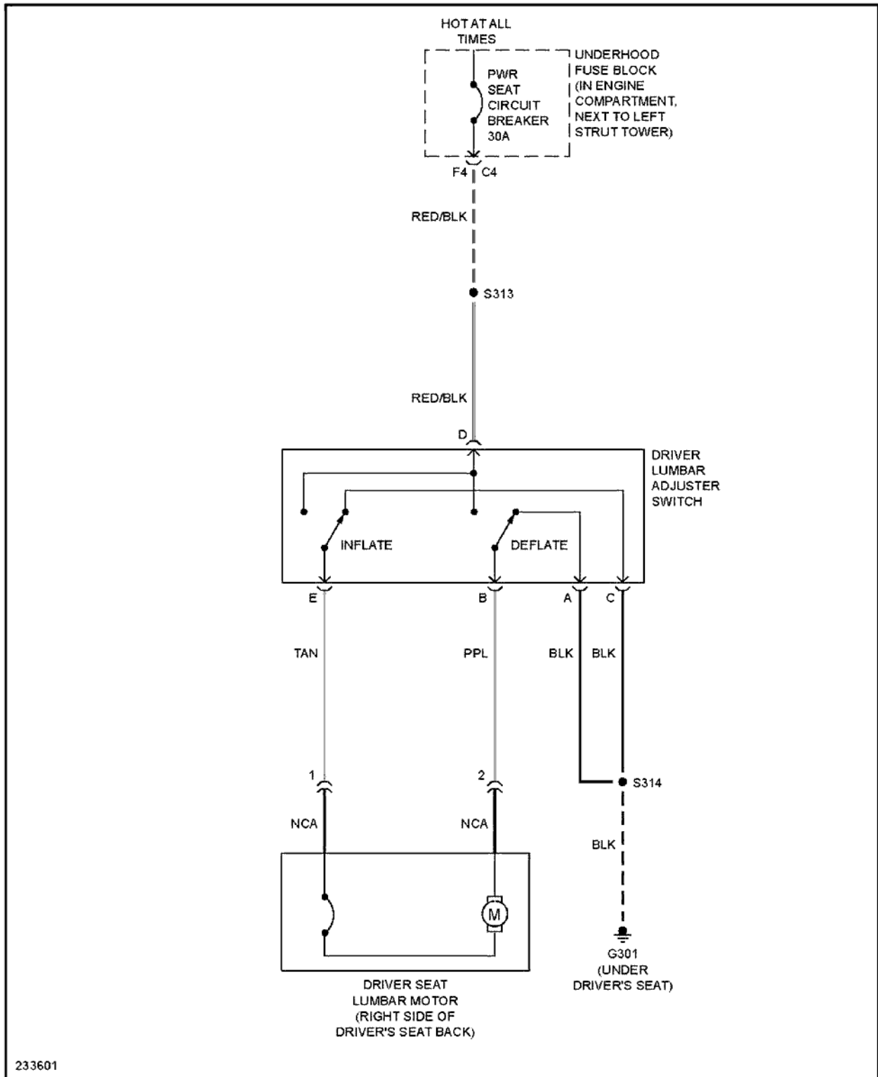
Fig. 41: Driver's Lumbar Circuit
