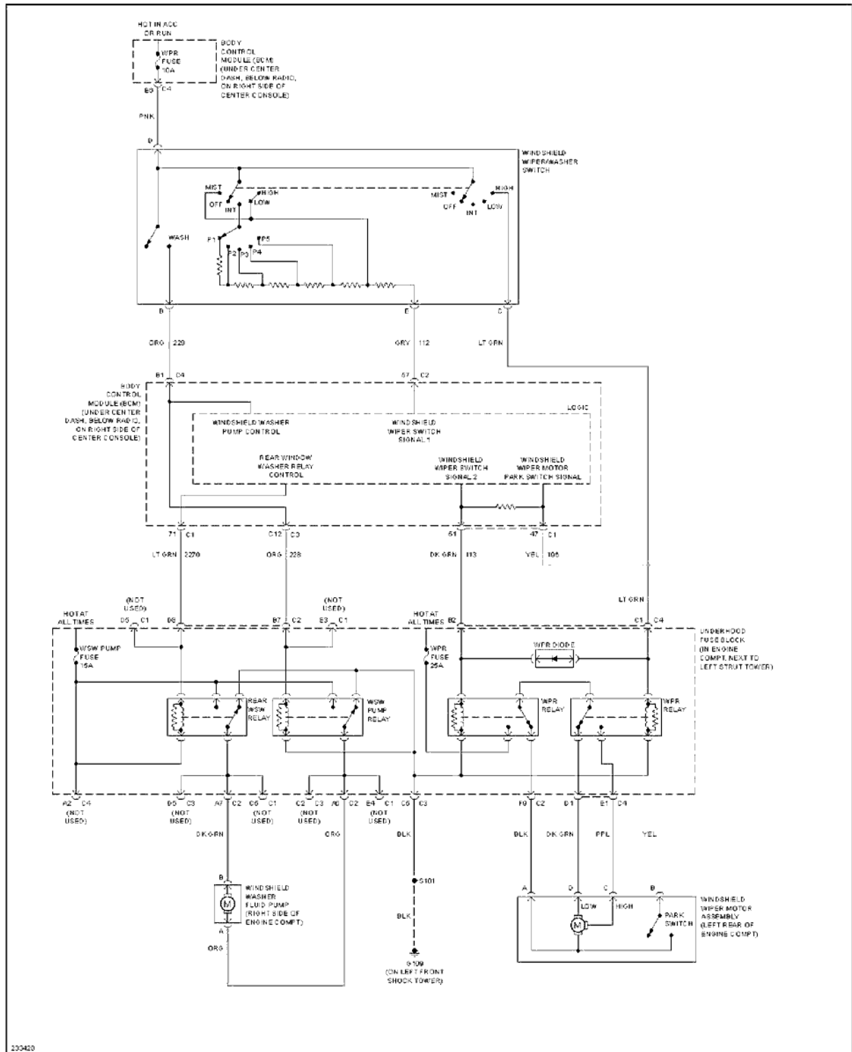
Fig. 57: Front Wiper/Washer Circuit
