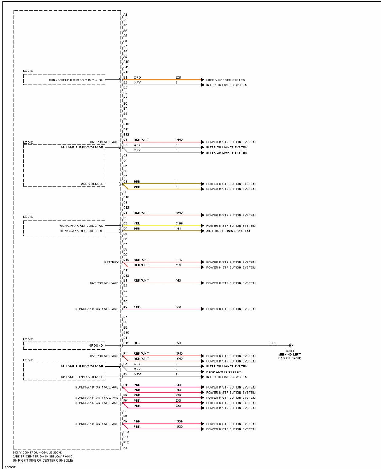
Fig. 9: Body Control Modules Circuit (3 of 4)
