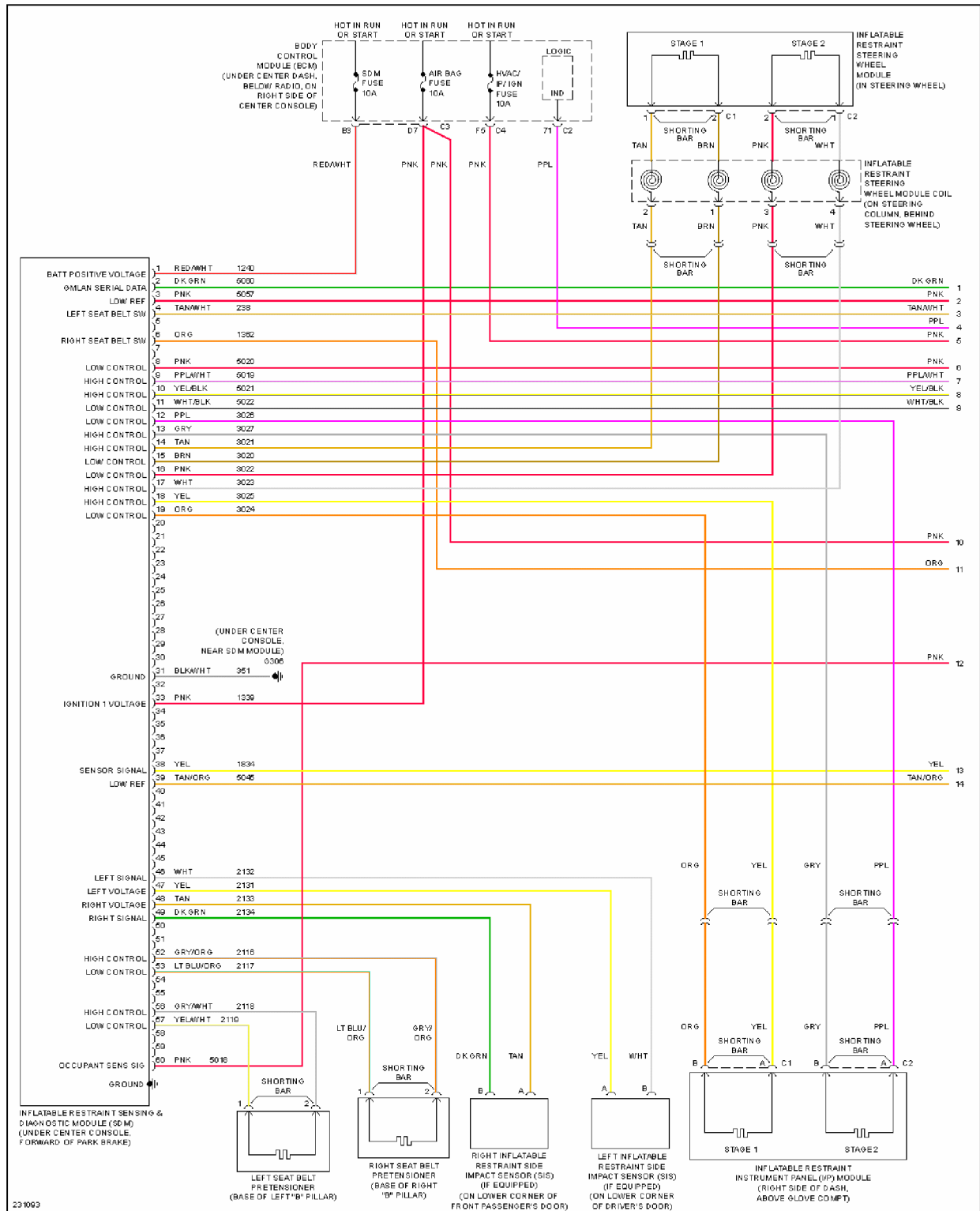
Fig. 51: Supplemental Restraints Circuit (1 of 2)
