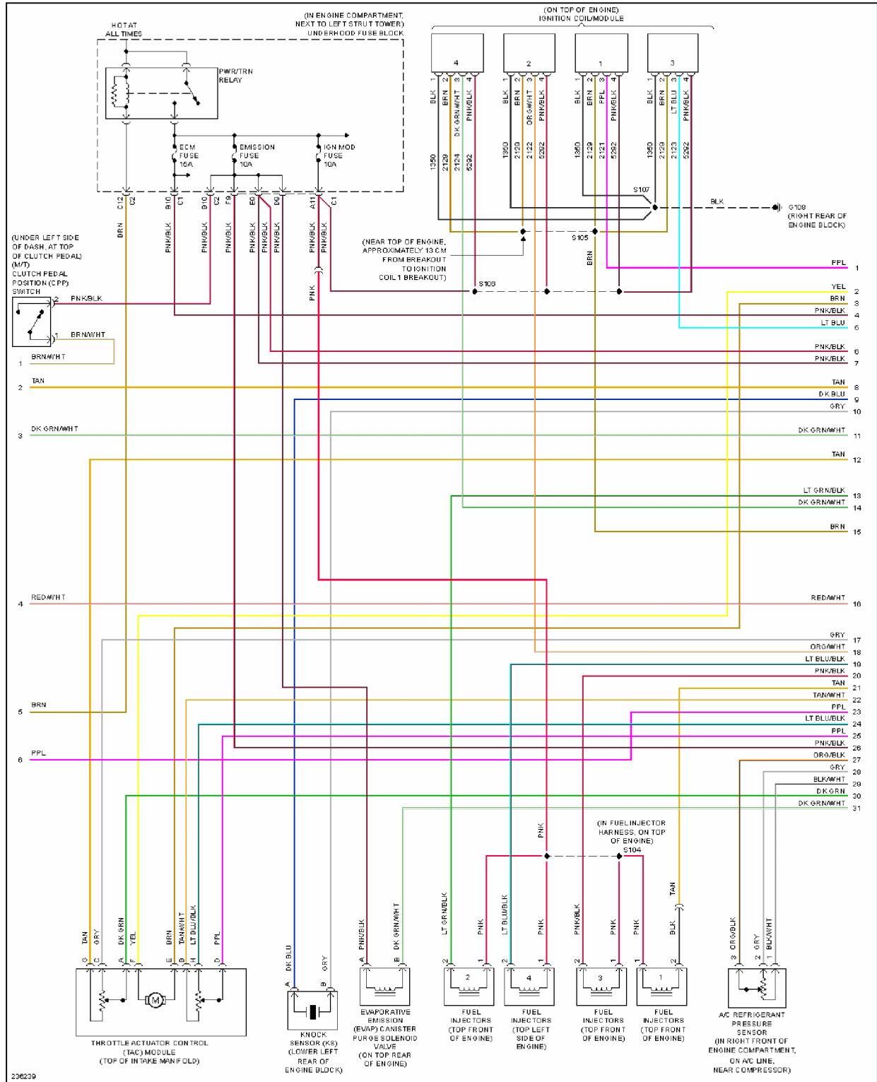
Fig. 21: 2.4L VIN B, Engine Performance Circuit (2 of 4)
