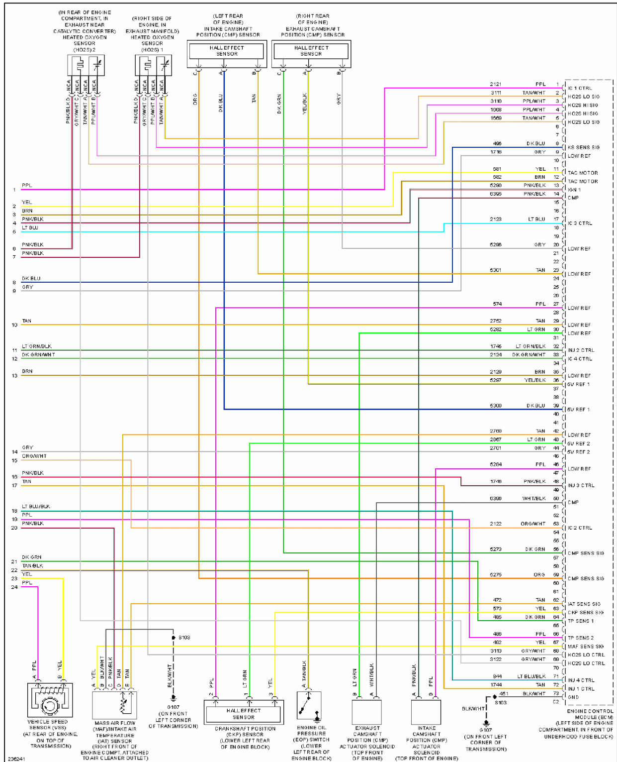
Fig. 23: 2.4L VIN B, Engine Performance Circuit (4 of 4)
