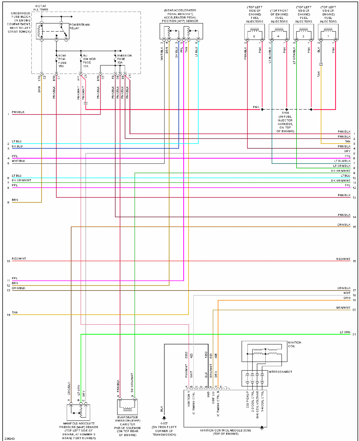
Fig. 17: 2.2L VIN F, Engine Performance Circuit (2 of 4)
