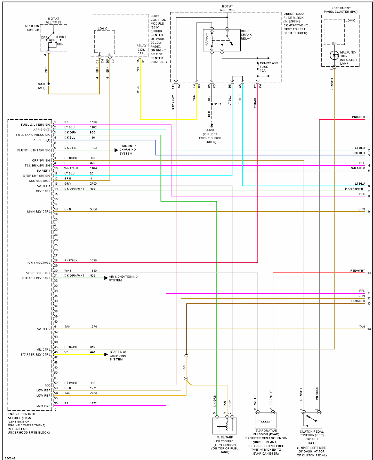
Fig. 16: 2.2L VIN F, Engine Performance Circuit (1 of 4)
