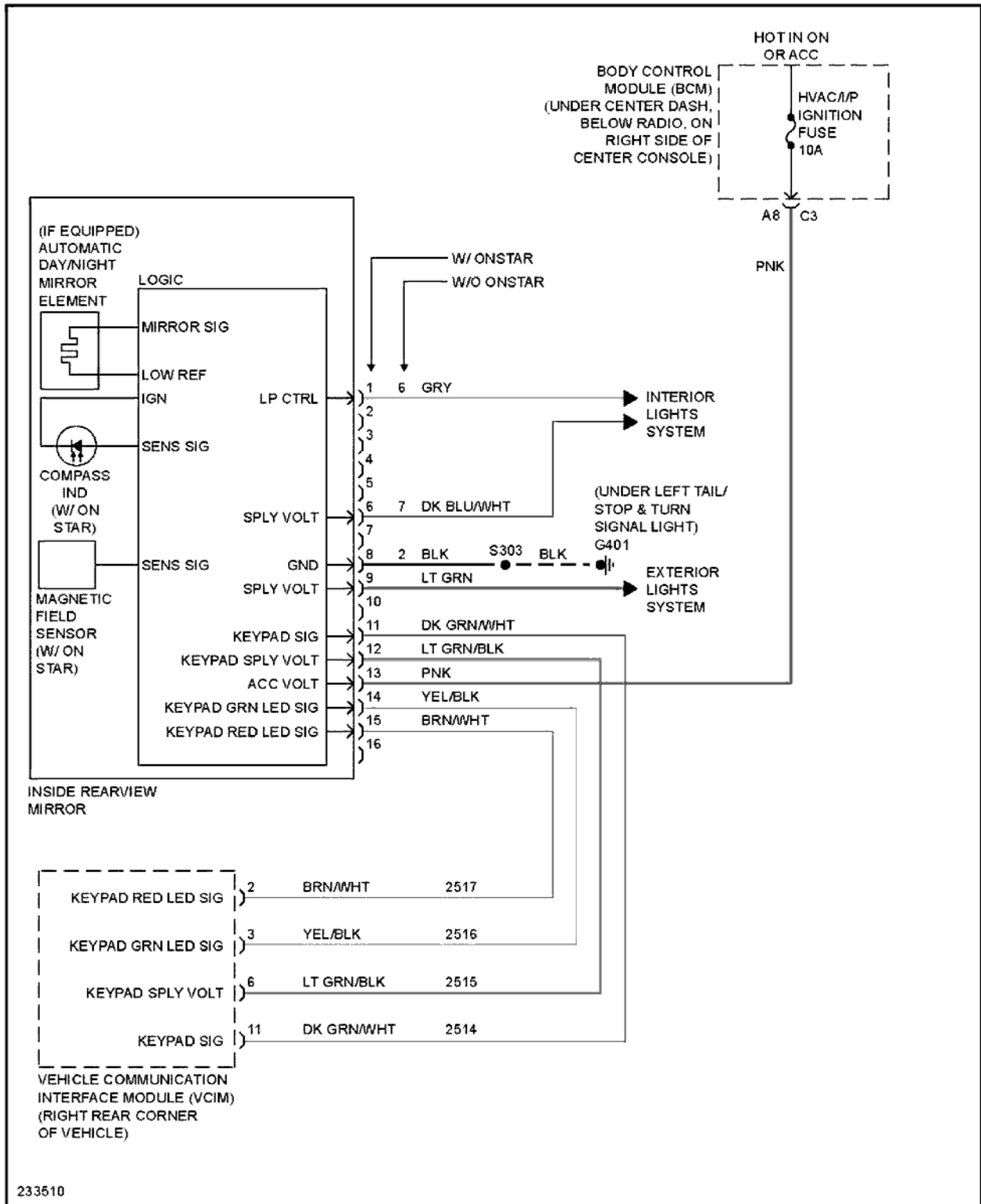
Fig. 38: Automatic Day/Night Mirror Circuit
