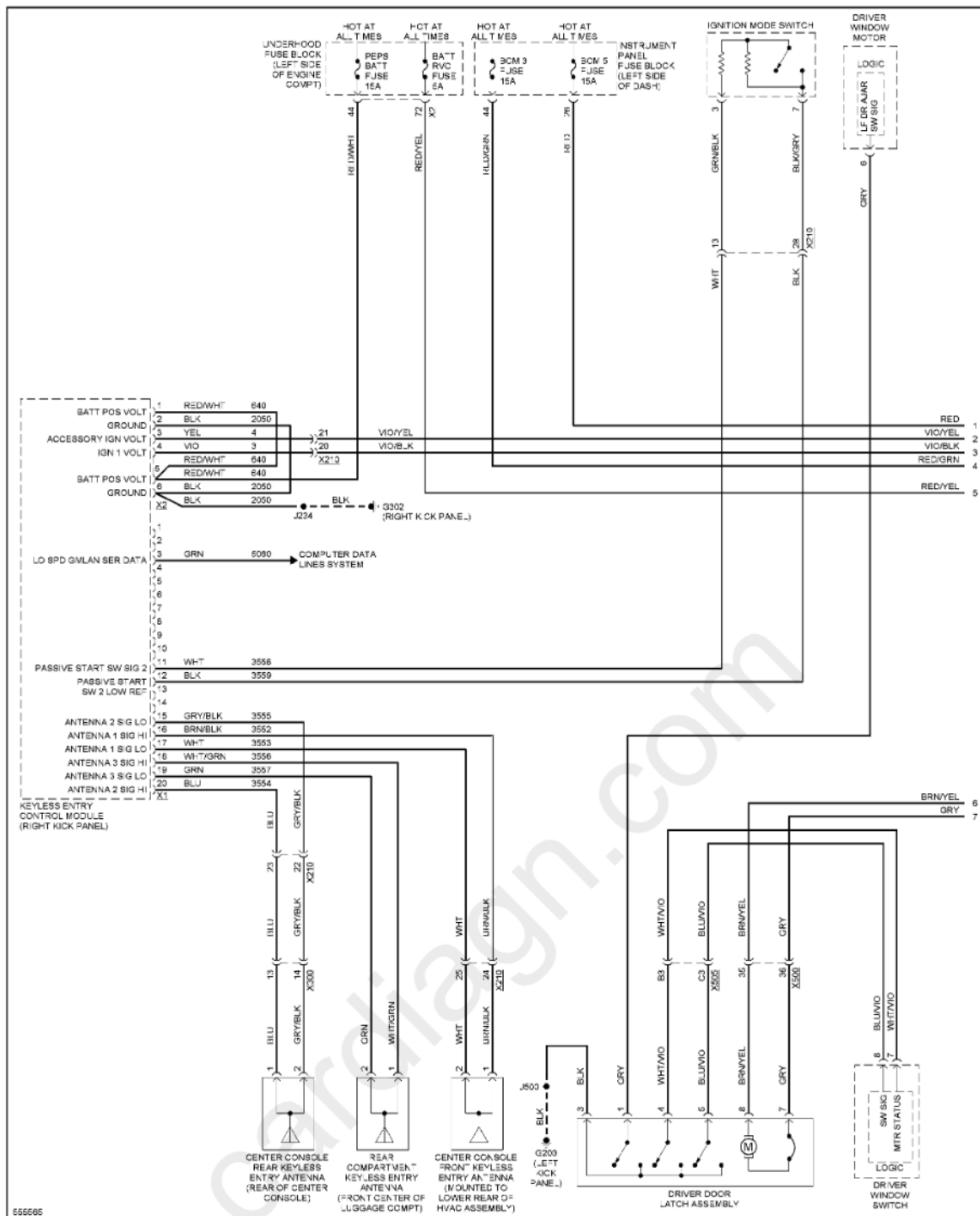
Fig. 91: Power Door Locks Circuit, W/ Passive Keyless Entry (1 of 4)
