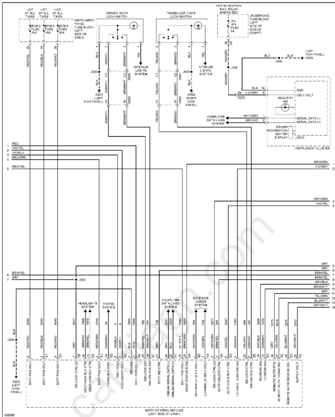
Fig. 92: Power Door Locks Circuit, W/ Passive Keyless Entry (2 of 4)
