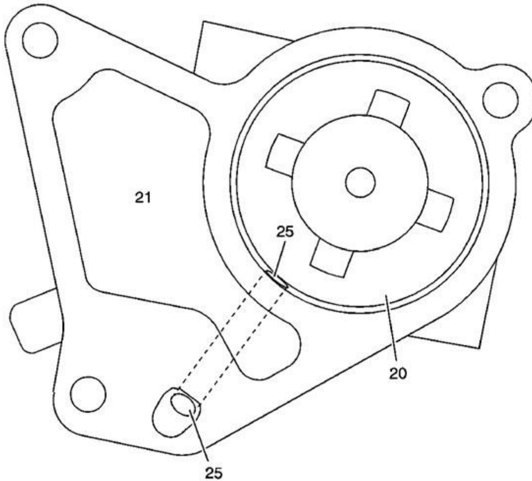
Fig. 570: 1-2 Accumulator Cover Fluid Passages Courtesy of GENERAL MOTORS CORP.
