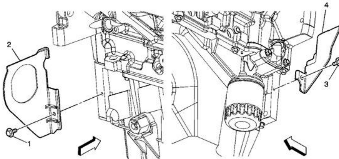
Fig. 120: View Of Torque Converter Covers & Bolts Courtesy of GENERAL MOTORS CORP.
