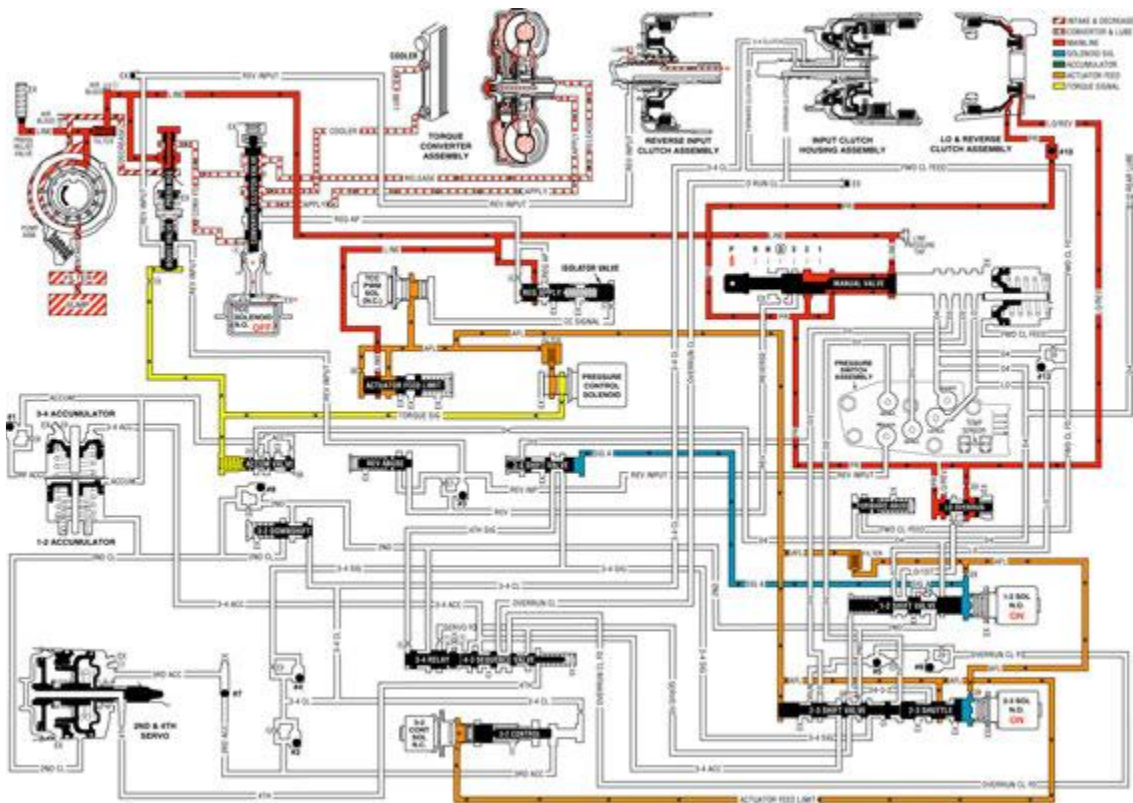
Fig. 547: Park - Engine Running Courtesy of GENERAL MOTORS CORP.
