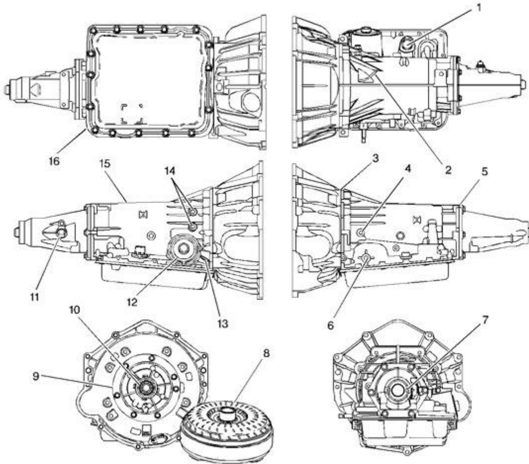
Fig. 4: Leak Inspection Points Courtesy of GENERAL MOTORS CORP.
