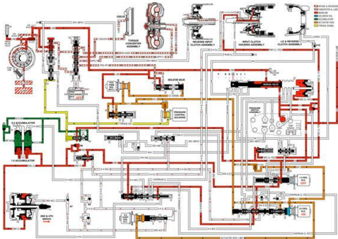
Fig. 555: Overdrive Range, 3-2 Downshift Courtesy of GENERAL MOTORS CORP.
