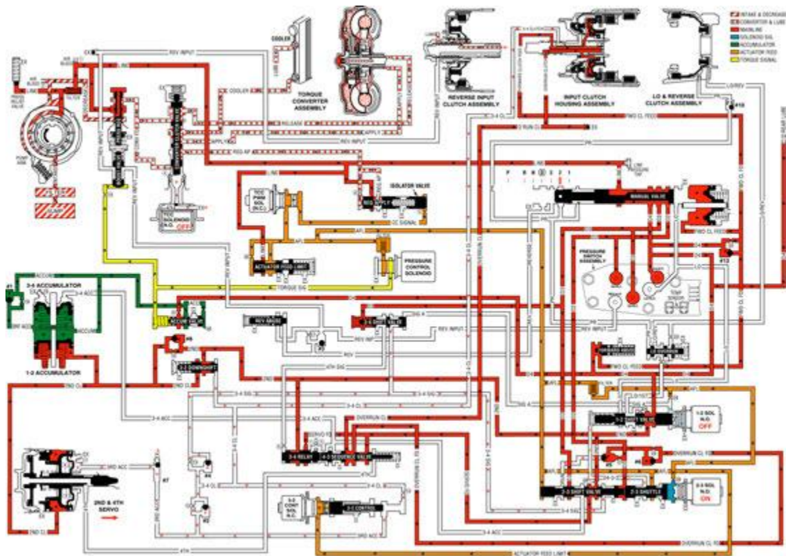
Fig. 557: Manual Second Gear Courtesy of GENERAL MOTORS CORP.
