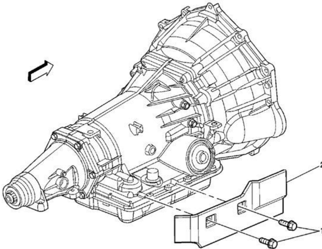
Fig. 121: Transmission Heat Shield Replacement Courtesy of GENERAL MOTORS CORP.
