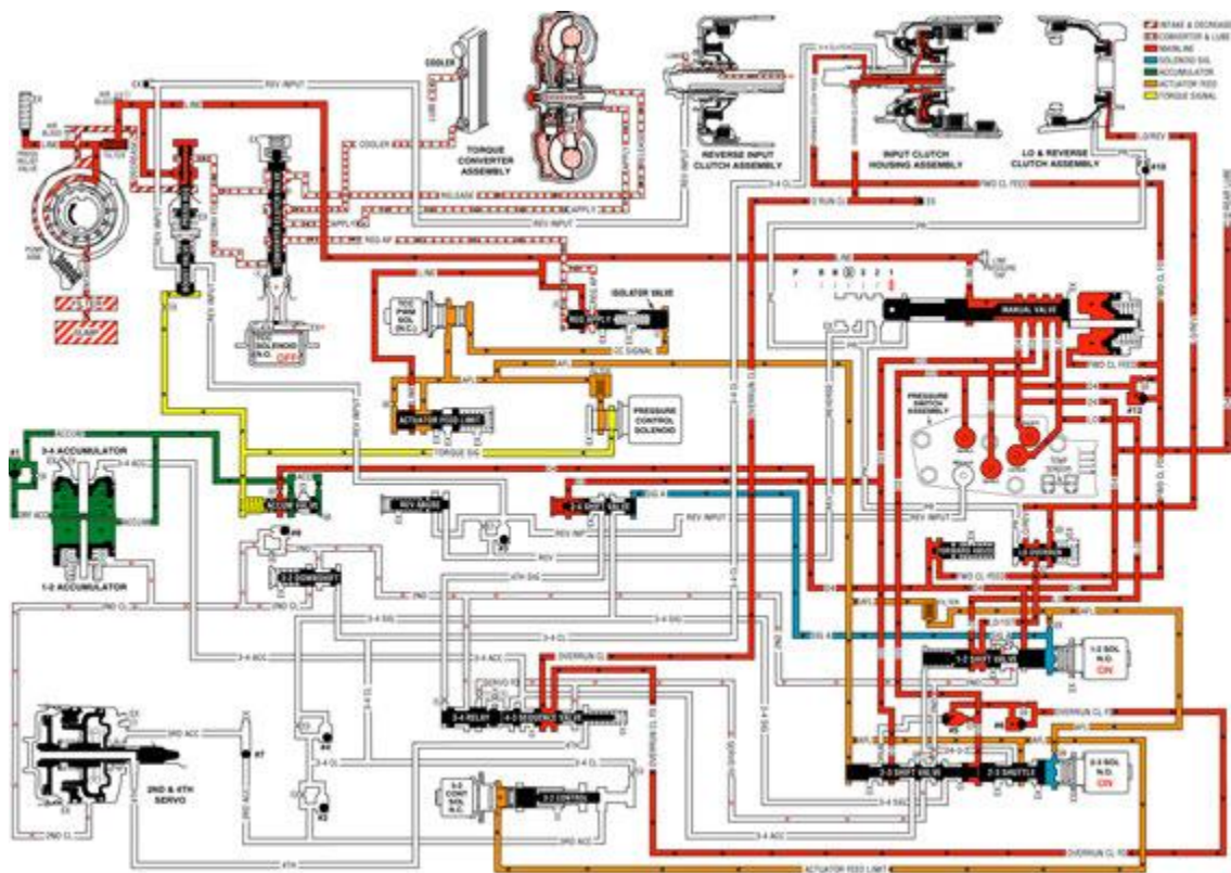
Fig. 558: Manual First Gear Courtesy of GENERAL MOTORS CORP.
