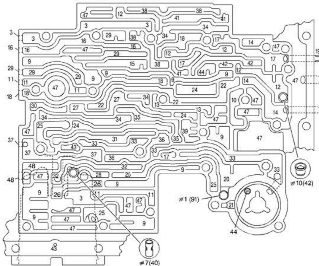
Fig. 563: Case Fluid Passages (Control Valve Body Side)
