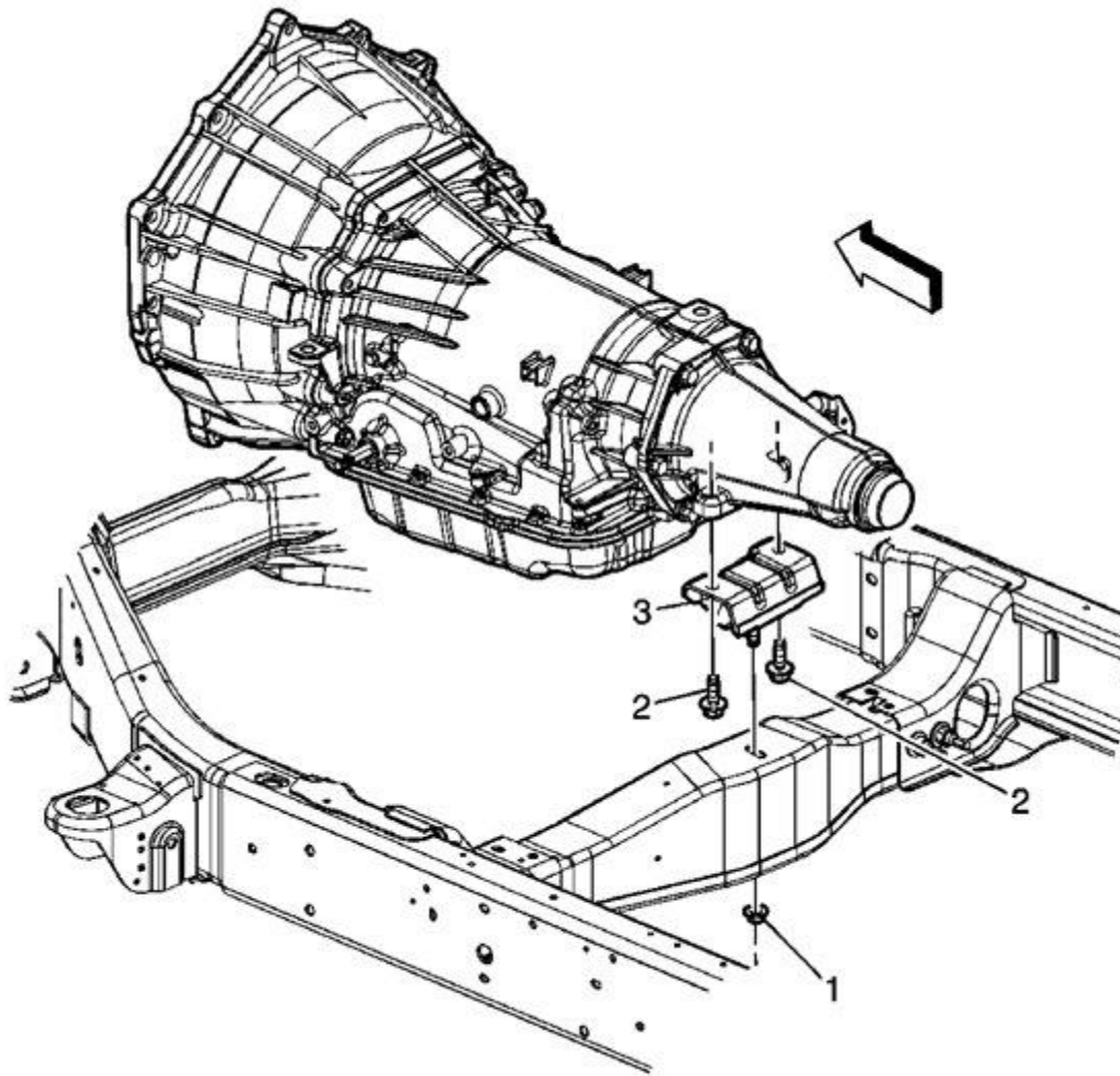
Fig. 204: Transmission Mount Replacement (2WD) Courtesy of GENERAL MOTORS CORP.
