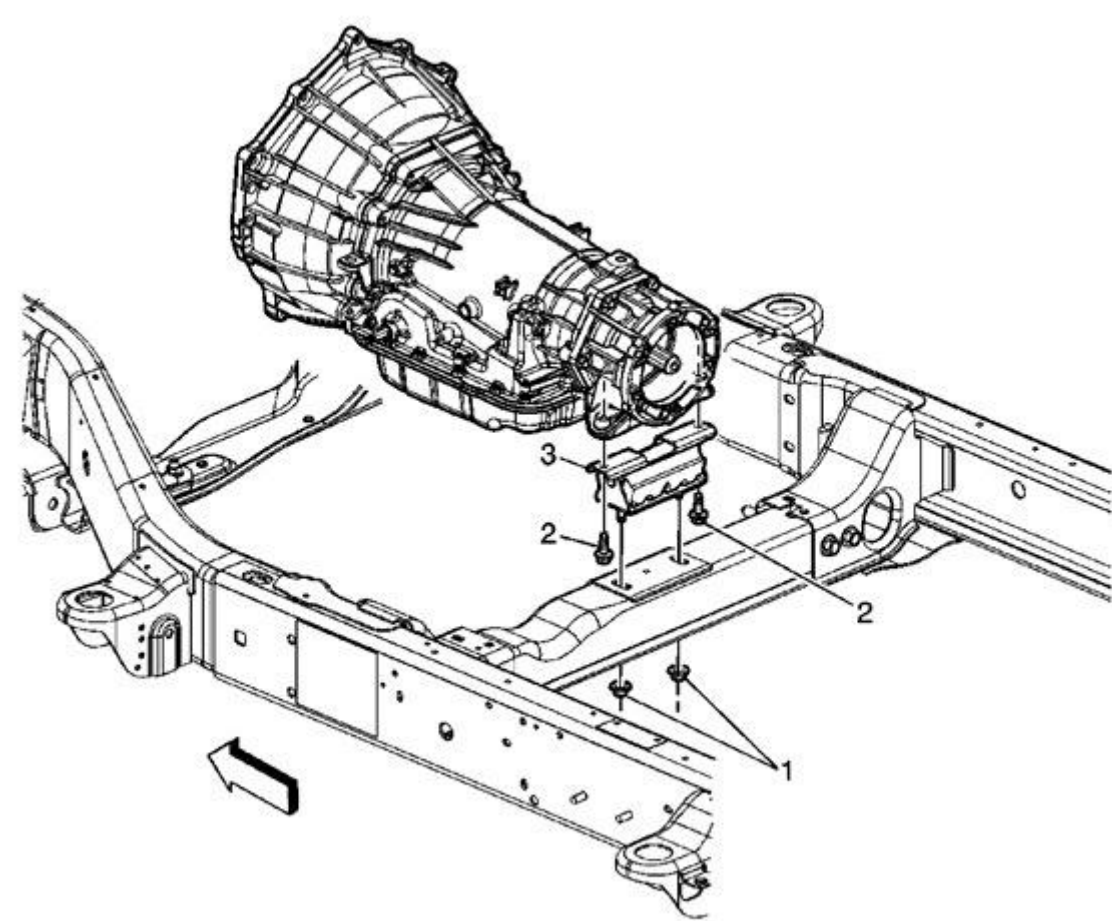
Fig. 205: Transmission Mount Replacement (4WD) Courtesy of GENERAL MOTORS CORP.
