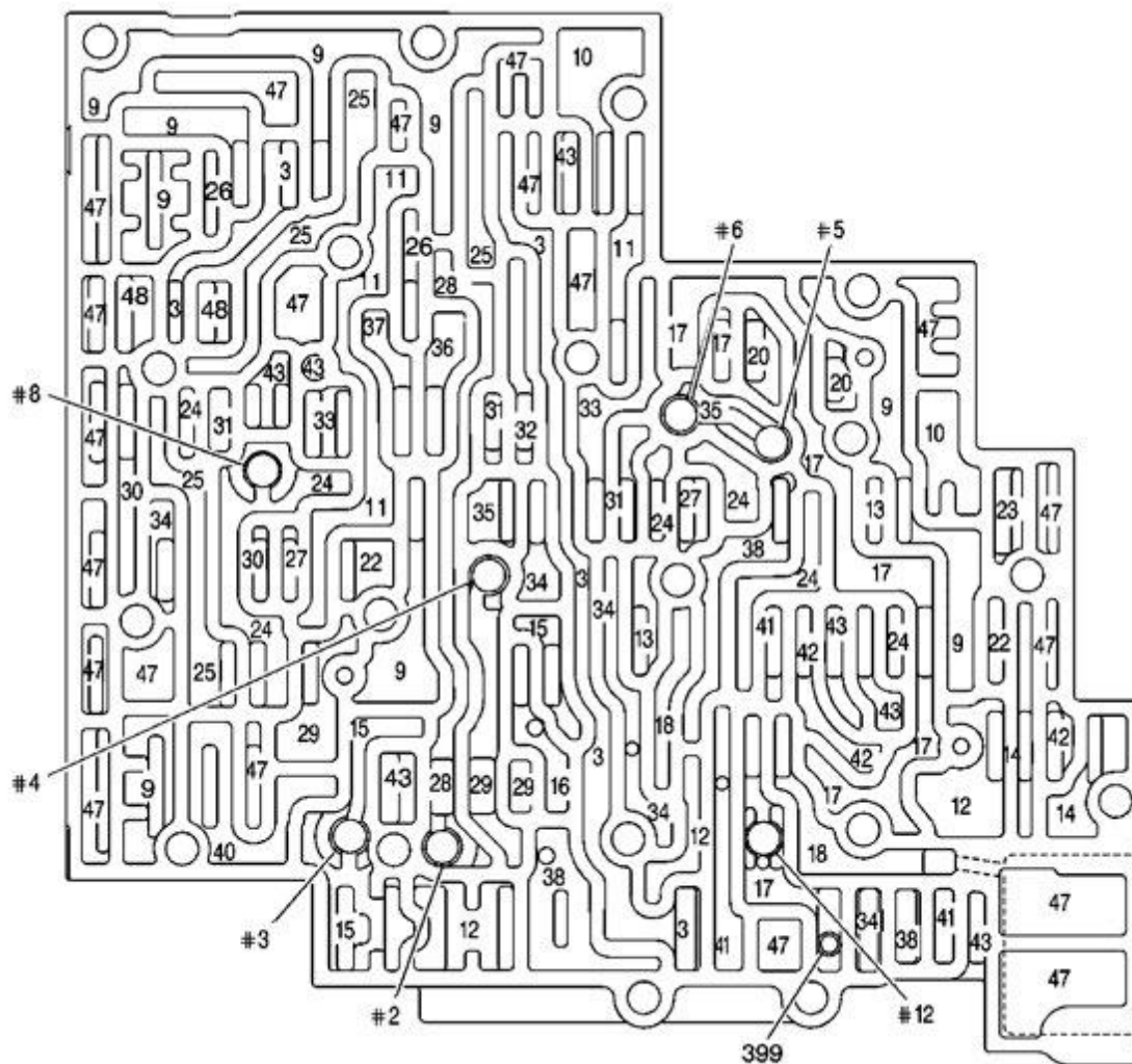
Fig. 567: Control Valve Body Fluid Passages (Case Side) Courtesy of GENERAL MOTORS CORP.
