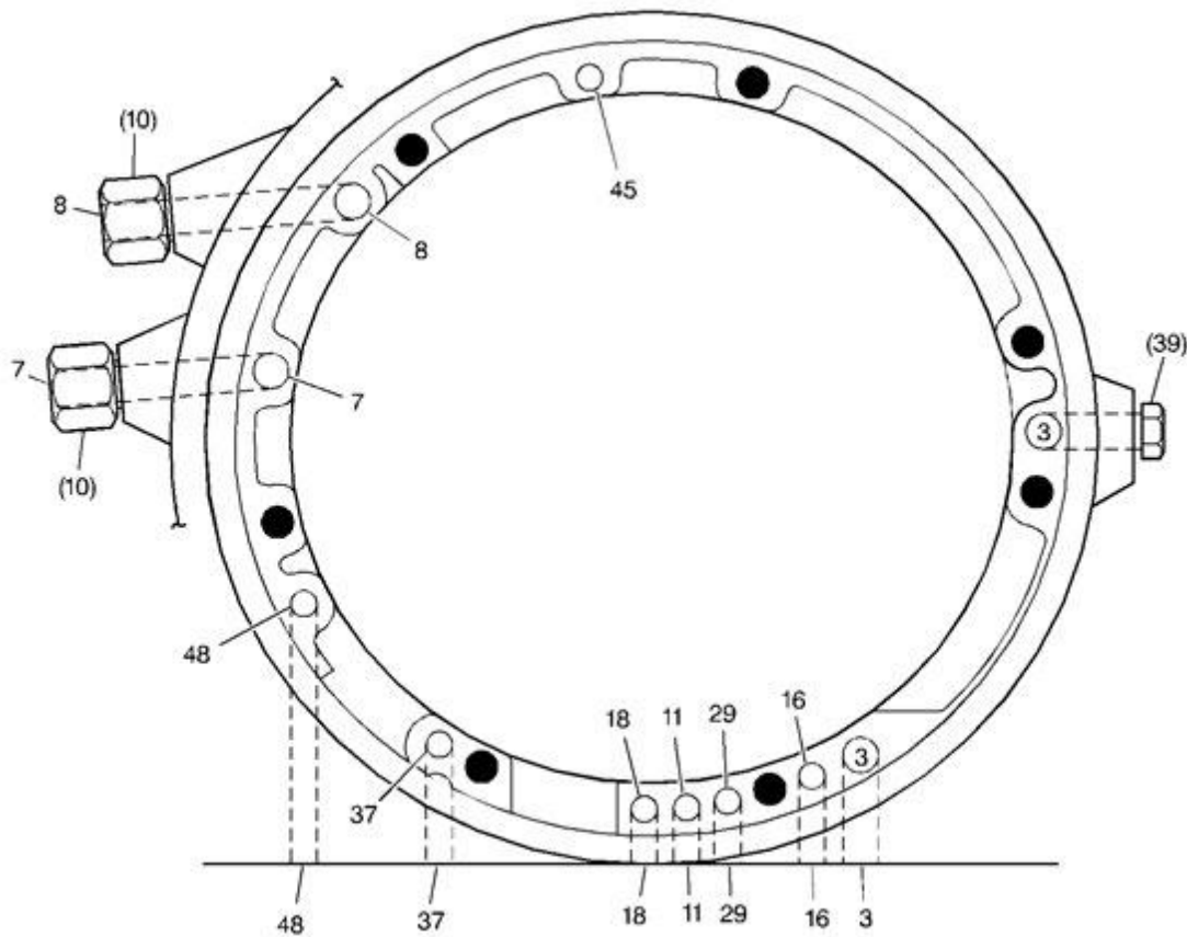
Fig. 562: Case Fluid Passages (Pump Cover Side) Courtesy of GENERAL MOTORS CORP.
