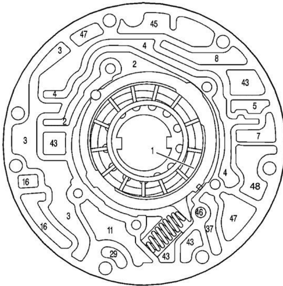
Fig. 559: Pump Body Fluid Passages (Pump Cover Side) Courtesy of GENERAL MOTORS CORP.
