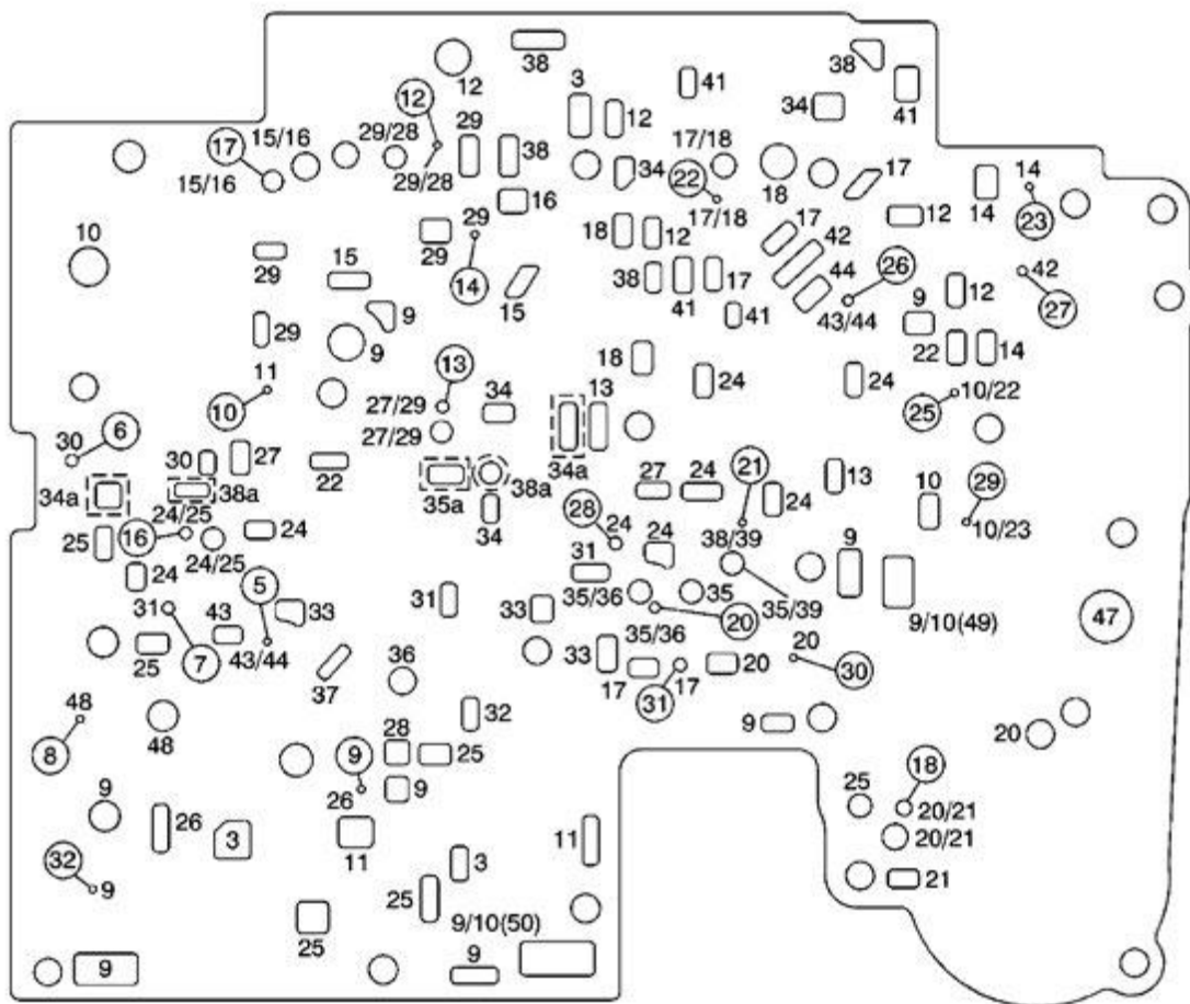
Fig. 565: Spacer Plate Fluid Passages Courtesy of GENERAL MOTORS CORP.
