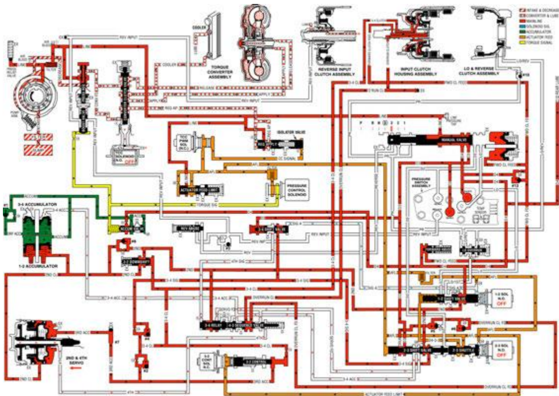
Fig. 556: Manual Third Gear Courtesy of GENERAL MOTORS CORP.
