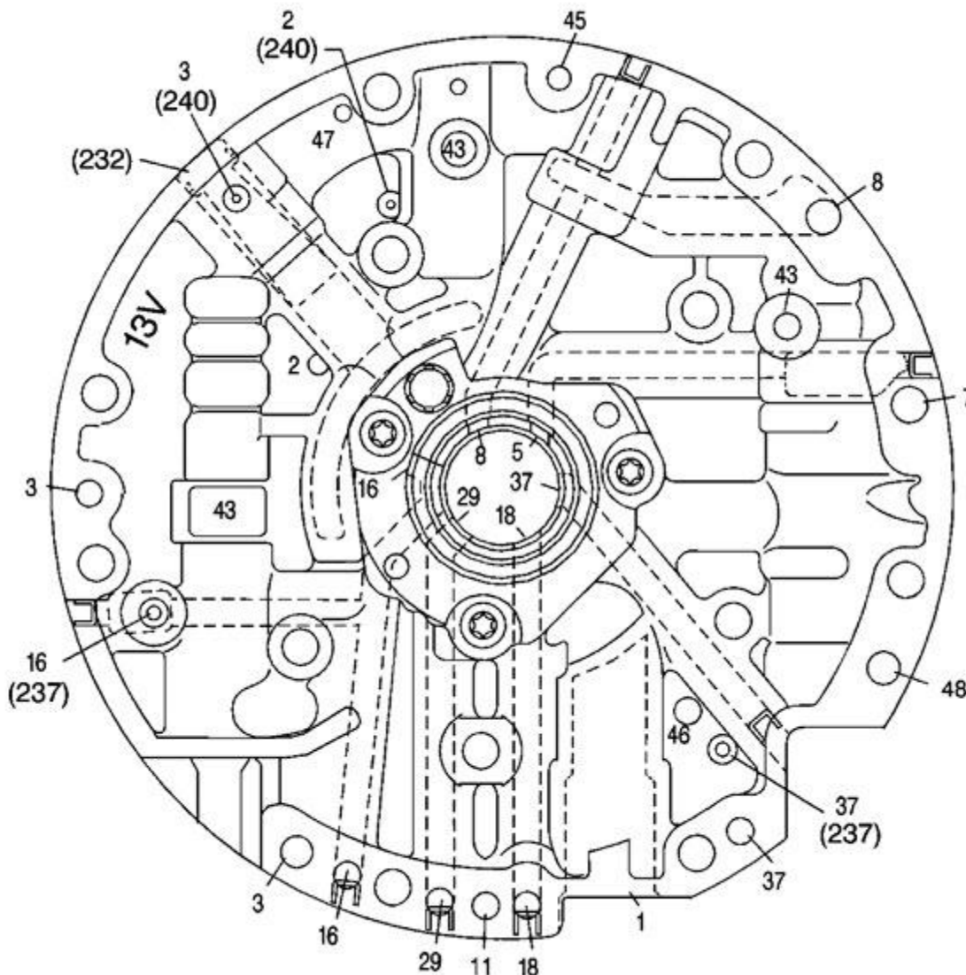
Fig. 561: Identifying Pump Cover Fluid Passages (Case Side) Courtesy of GENERAL MOTORS CORP.
