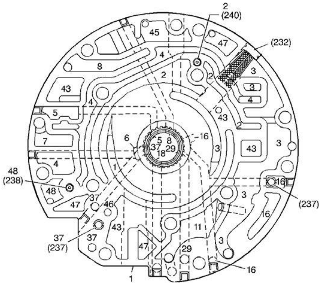
Fig. 560: Pump Cover Fluid Passages (Pump Body Side) Courtesy of GENERAL MOTORS CORP.
