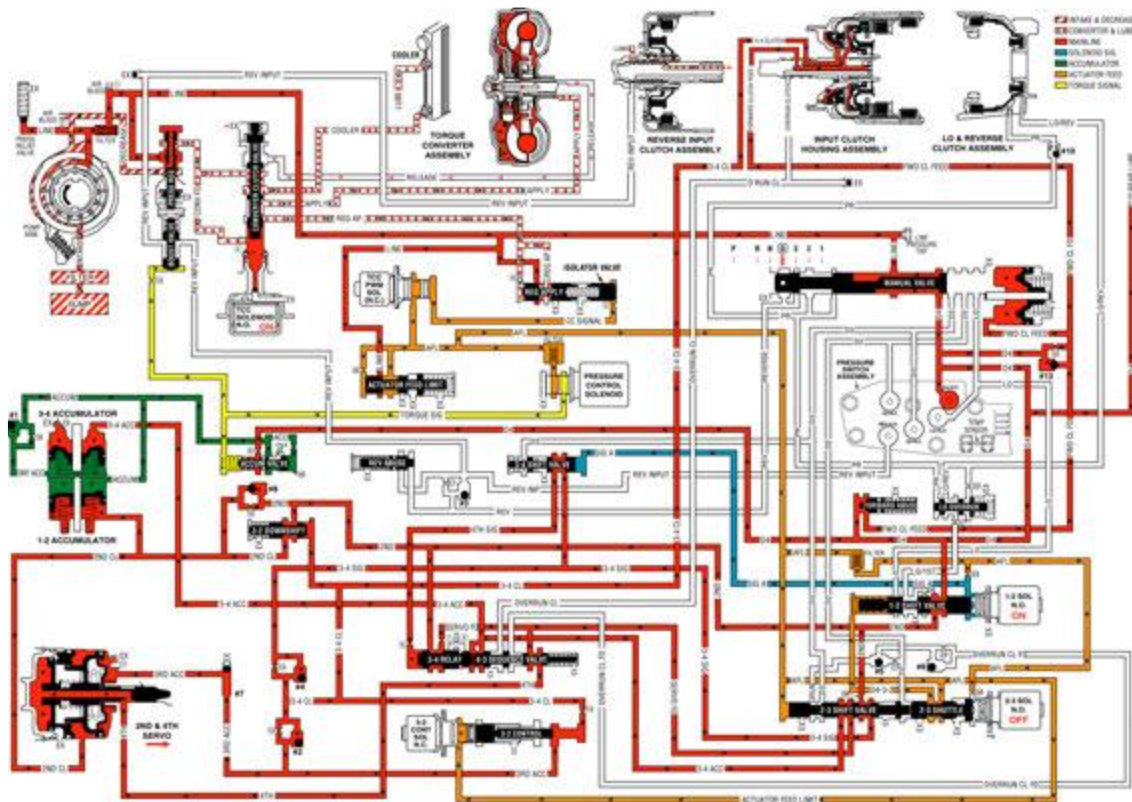
Fig. 553: Overdrive Range, Fourth Gear - TCC Applied Courtesy of GENERAL MOTORS CORP.
