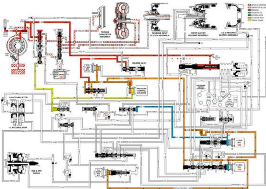
Fig. 549: Neutral - Engine Running Courtesy of GENERAL MOTORS CORP.
