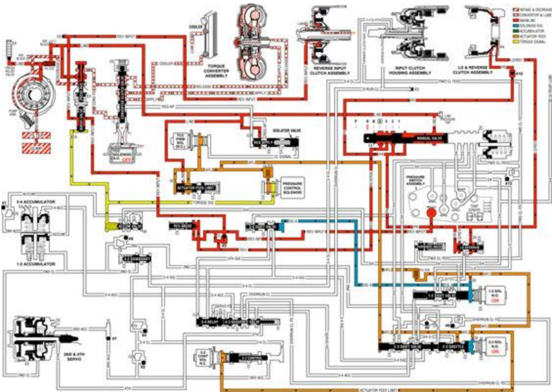
Fig. 548: Reverse Courtesy of GENERAL MOTORS CORP.
