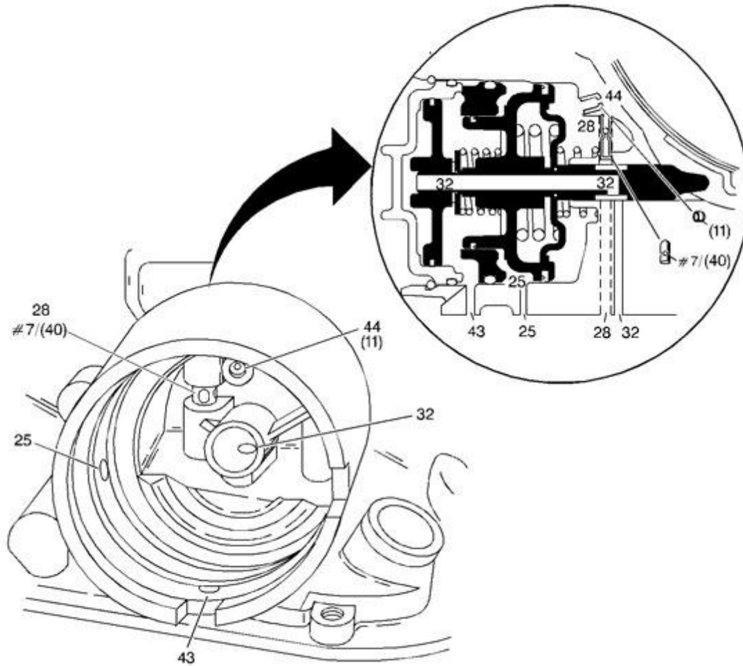
Fig. 568: 2-4 Servo Fluid Passages Courtesy of GENERAL MOTORS CORP.
