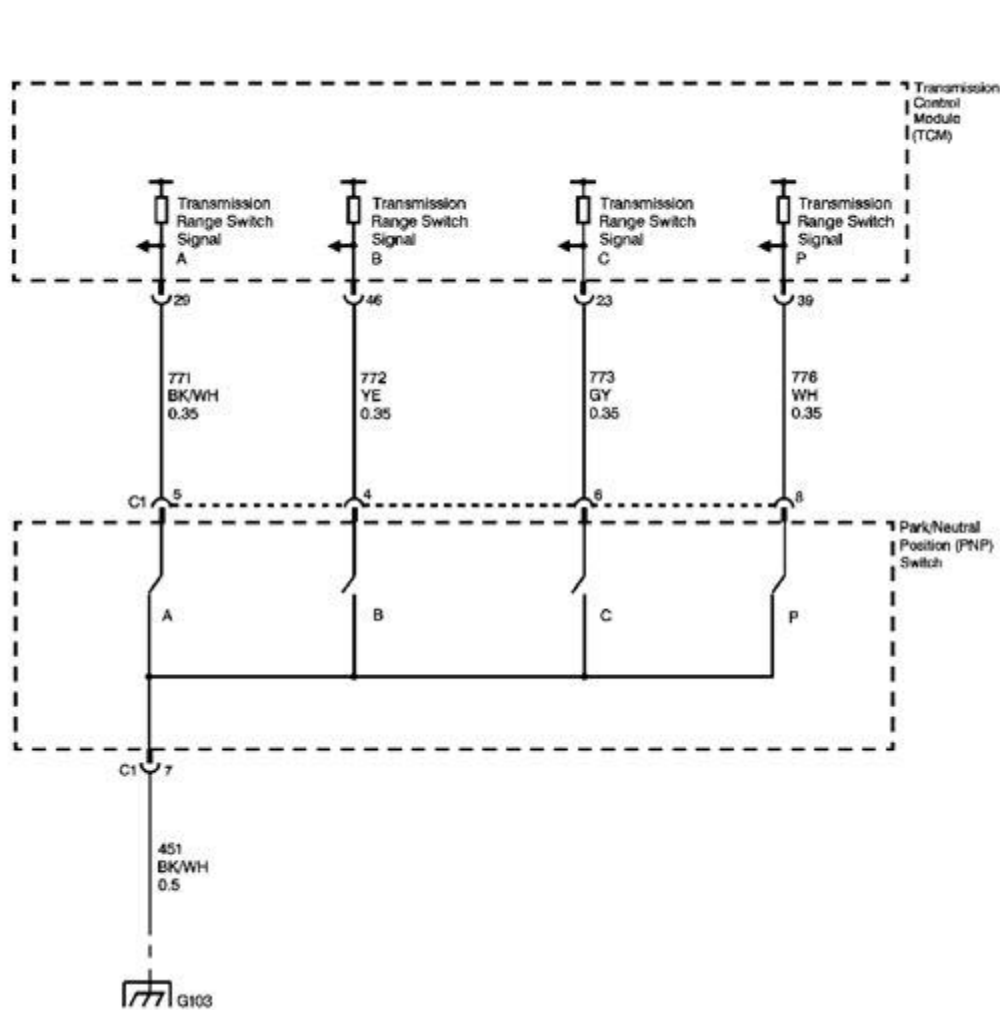
Fig. 1: Range Selector Schematic Courtesy of GENERAL MOTORS CORP.
