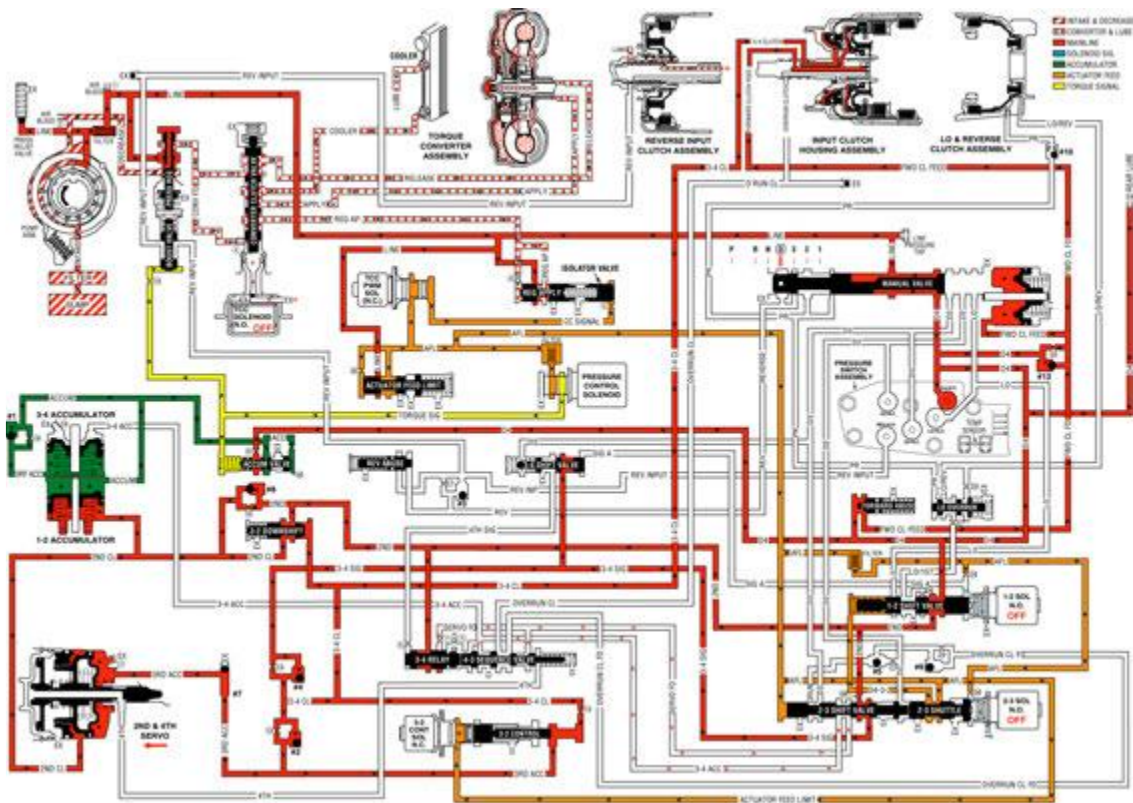
Fig. 552: Overdrive Range, Third Gear Courtesy of GENERAL MOTORS CORP.
