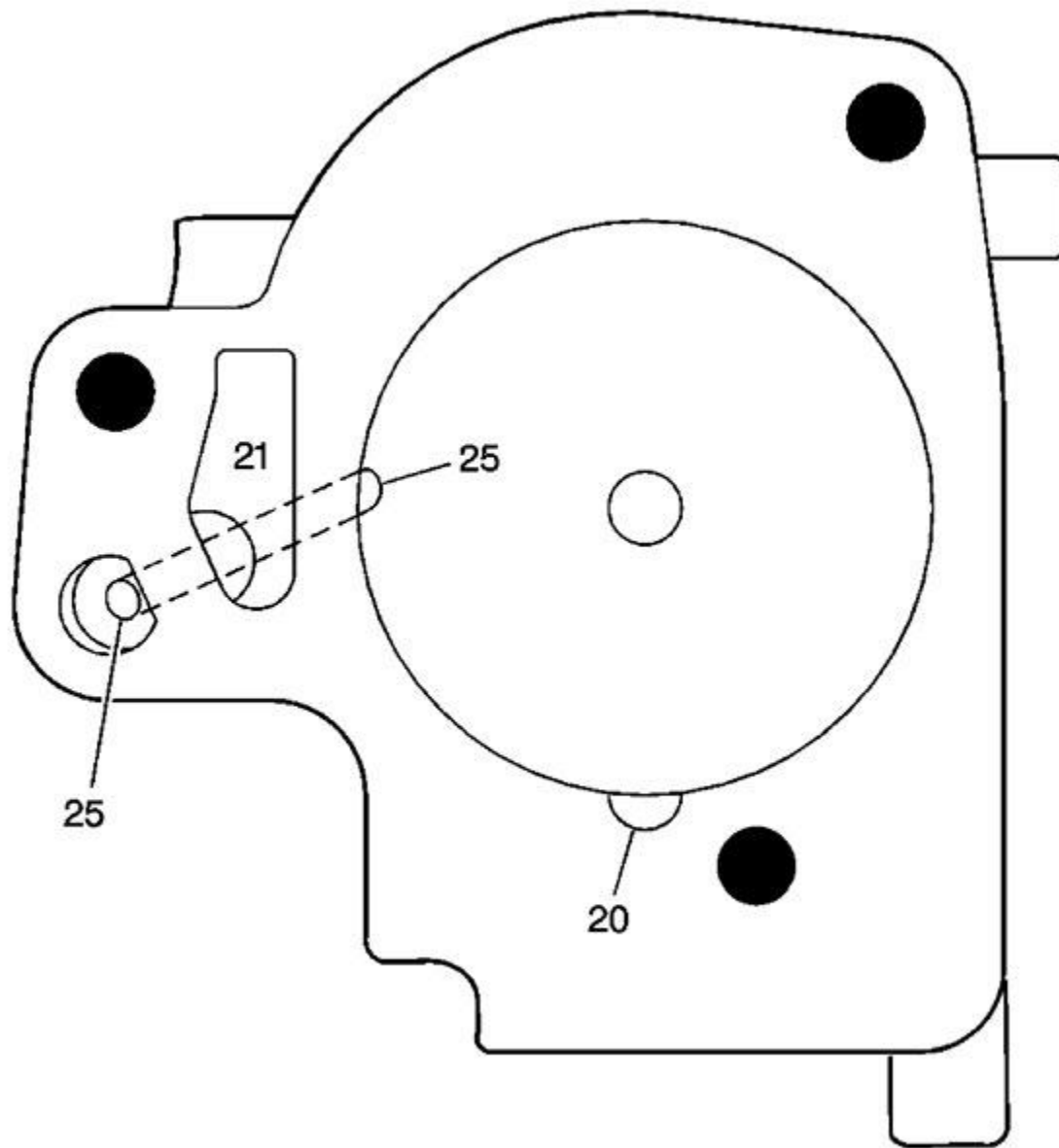
Fig. 569: 1-2 Accumulator Cover Fluid Passages Courtesy of GENERAL MOTORS CORP.
