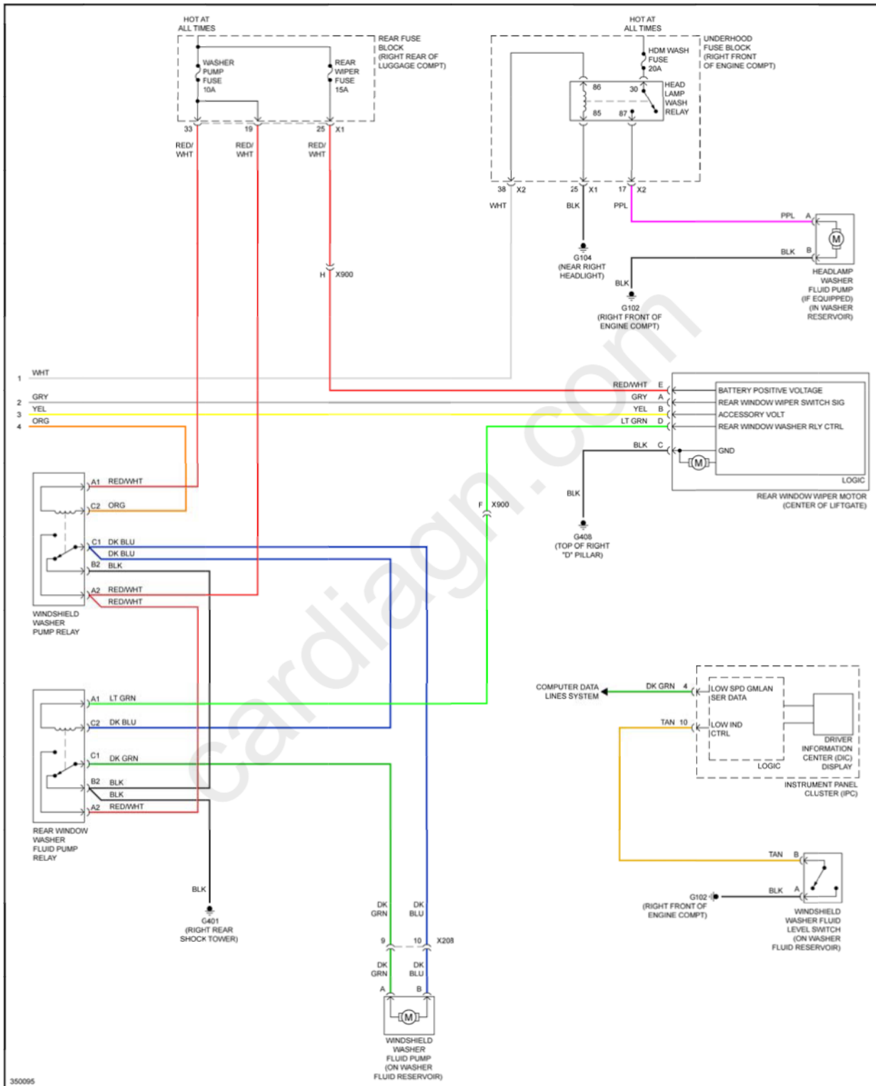
Fig. 124: Wiper/Washer Circuit, Wagon (2 of 2)
