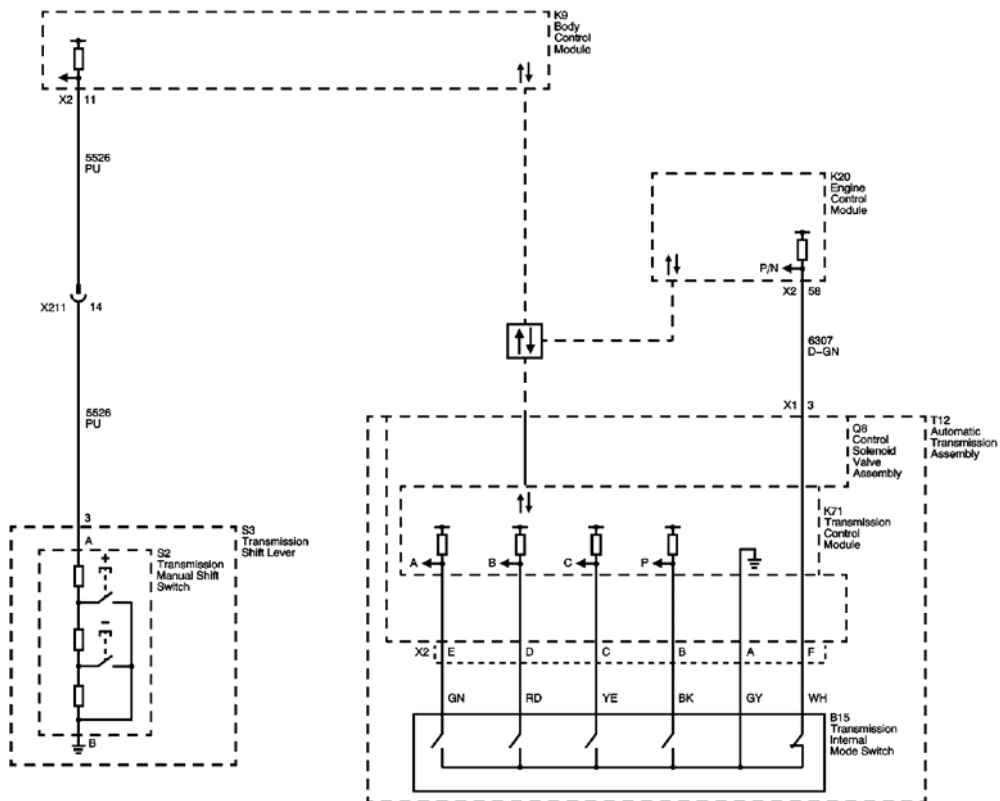
Fig. 3: IMS and Tap Up/Tap Down (MH7 or MHC) Courtesy of GENERAL MOTORS CORP.
