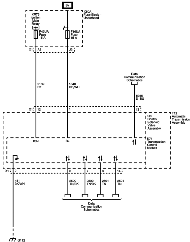
Fig. 1: Module Power, Ground, and Serial Data (MH7 or MHC) Courtesy of GENERAL MOTORS CORP.
