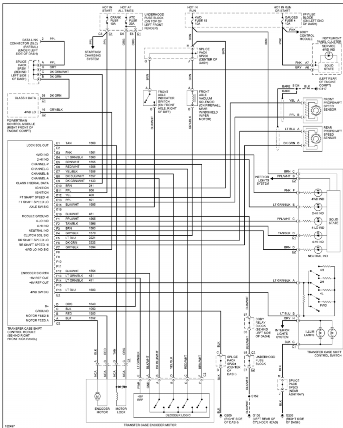
Fig. 55: 4.3L VIN W, Transfer Case Circuit, W/ 2-Speed Automatic Transfer Case
