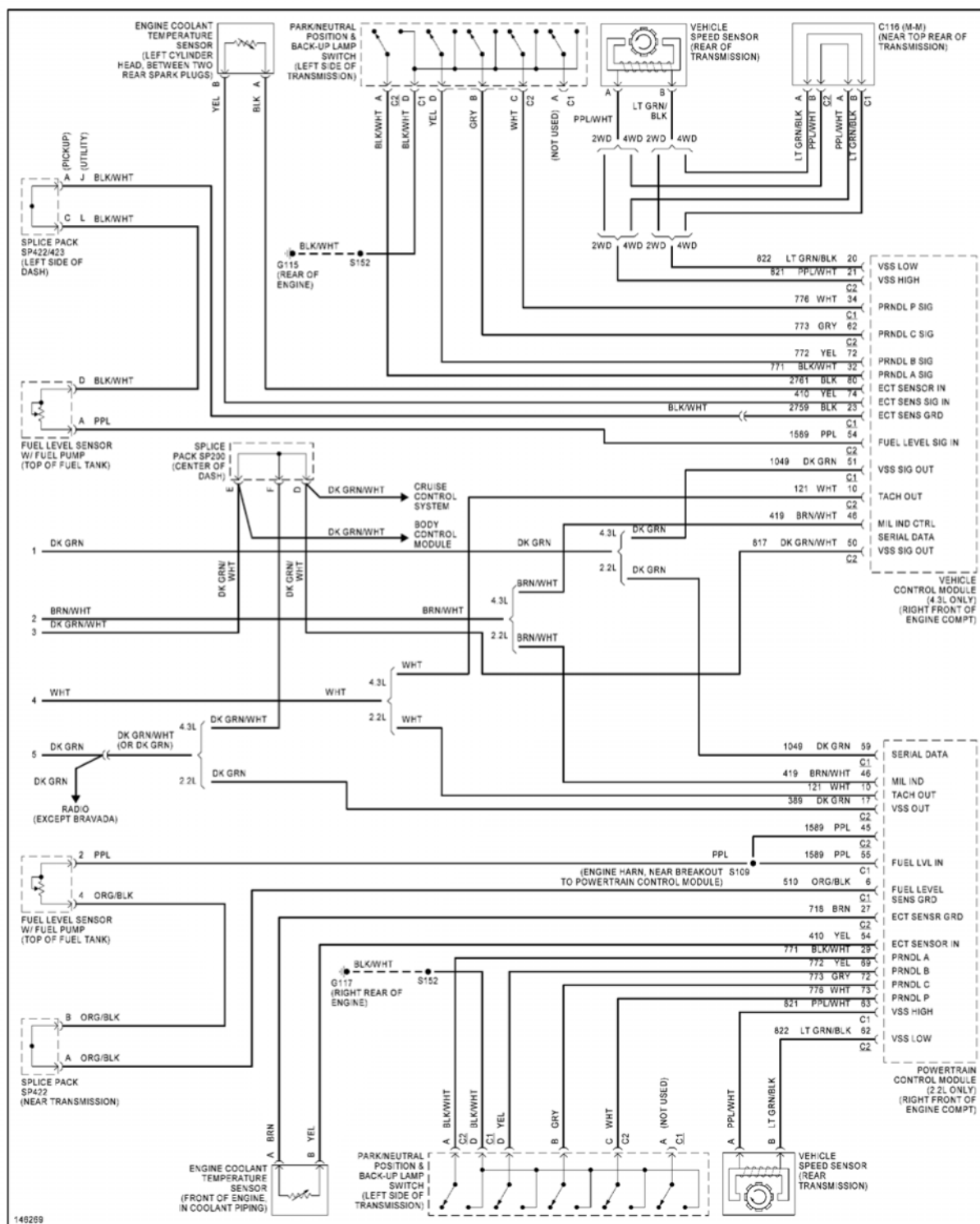
Fig. 27: Instrument Cluster Circuit (2 of 2)
