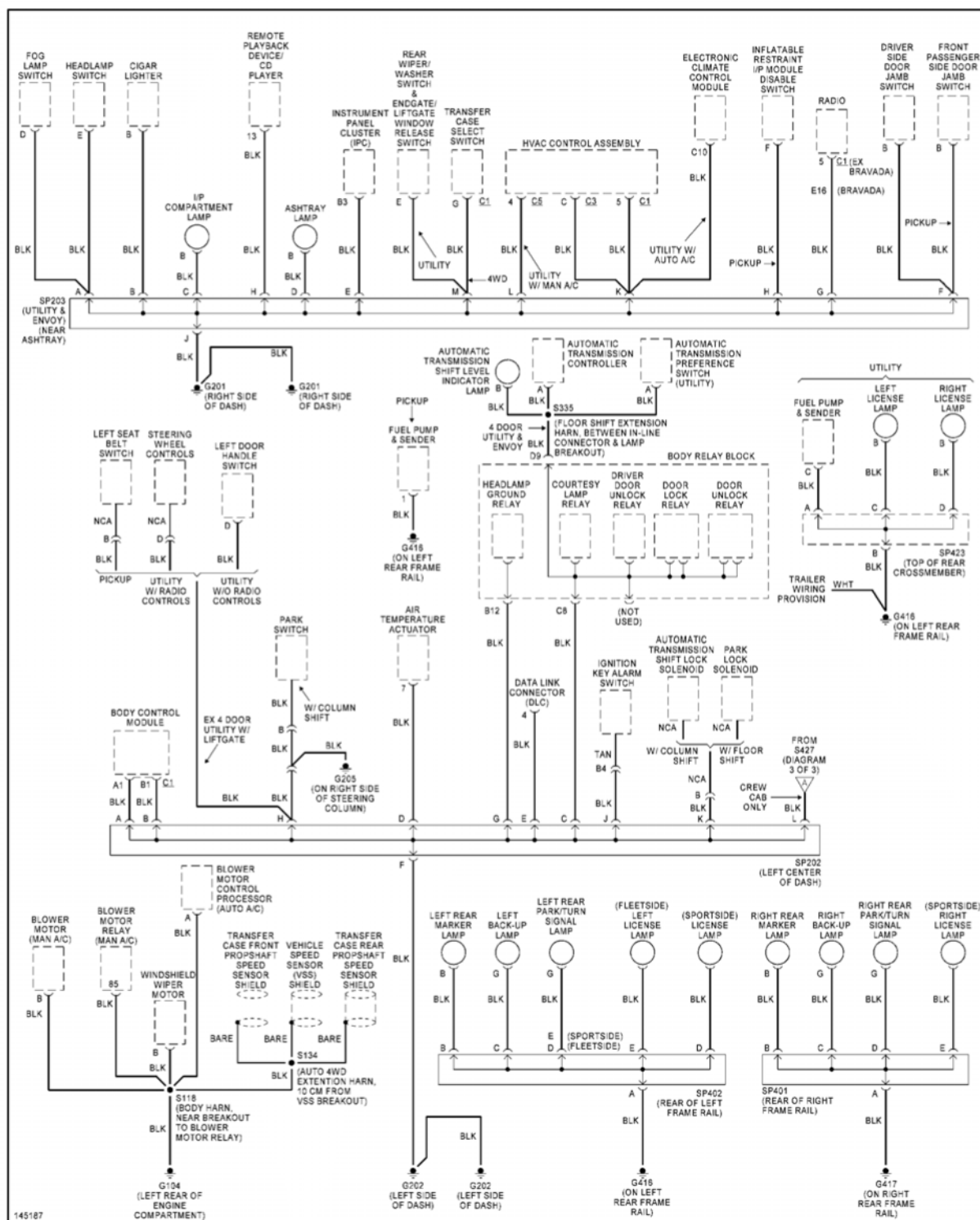
Fig. 21: Ground Distribution Circuit (2 of 3)
