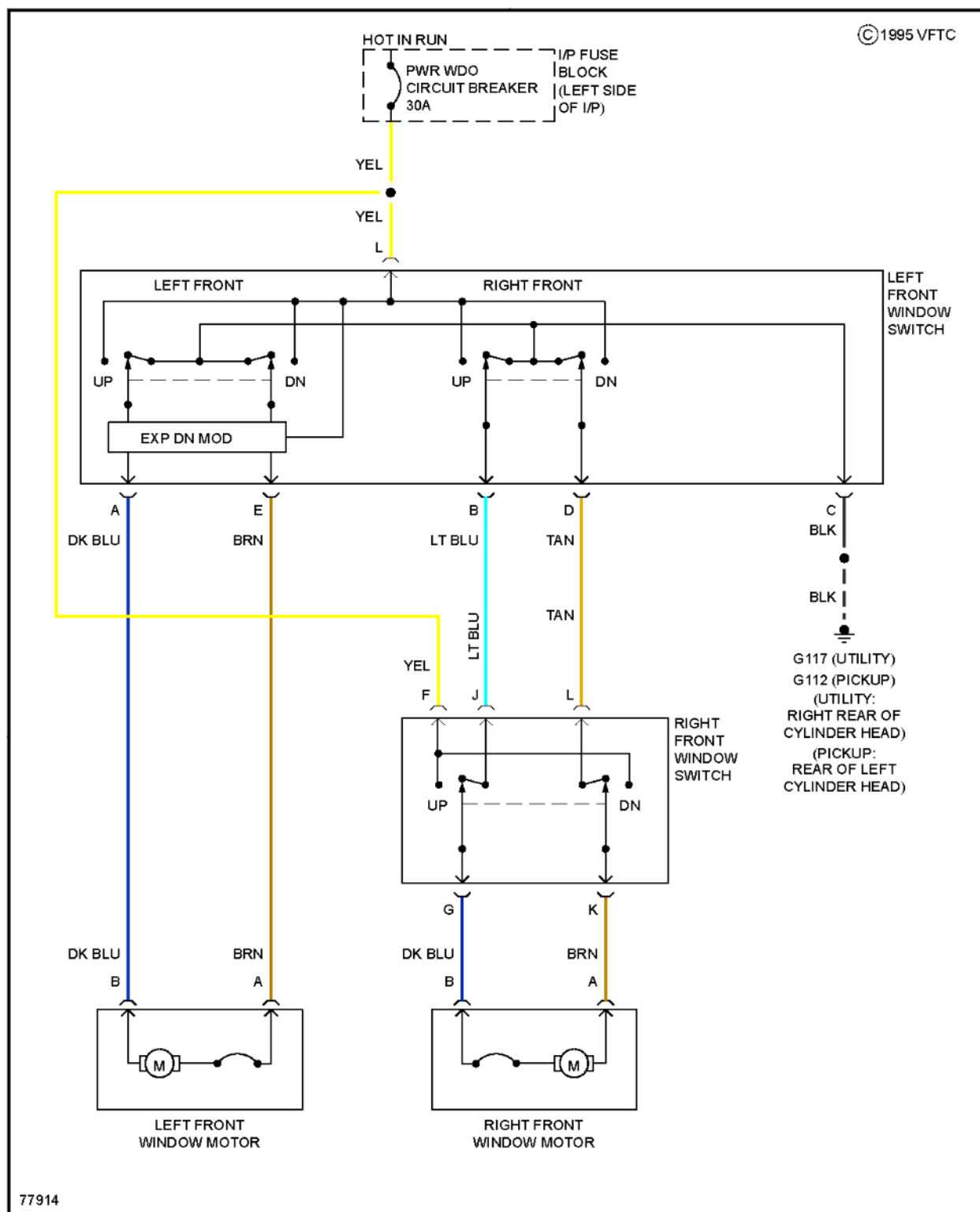
Fig. 28: Power Window Circuit, 2 Door
