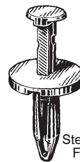
12756 (5973996) Brown Nylon Fascia Retainer Stem: 7/8"/Head Dia: 1" Shoulder Length: 1/4" Fits Into 1/2" Hole GM: 1982-On
