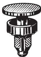
18165 (91508-SR3-000) Black Nylon Cowl Panel Push-Type Retainer Head Diameter: 17mm Stem Length: 9mm Fits Into 8mm Hole Honda 1990-On
