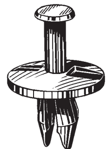
14010 (14045480) Black Nylon Fascia Retainer Stem: 23/32" / Head Dia: 1" Panel Range: 1/4" Fits Into 3/8" Hole GM 1982-On
