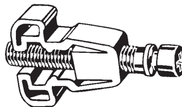
11657 (1606642, 1618890) 1/4"-28 x 1-7/8" Headlight Adjusting Screw & Nut Assembly Cadillac & Oldsmobile 1975-On UNIT PACKAGE: 100
