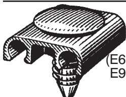
12133 (EOVB-13A506-BA) Nylon Clip Retainer Stem: 9/32" x 15/32" Long Ford 1979-On
