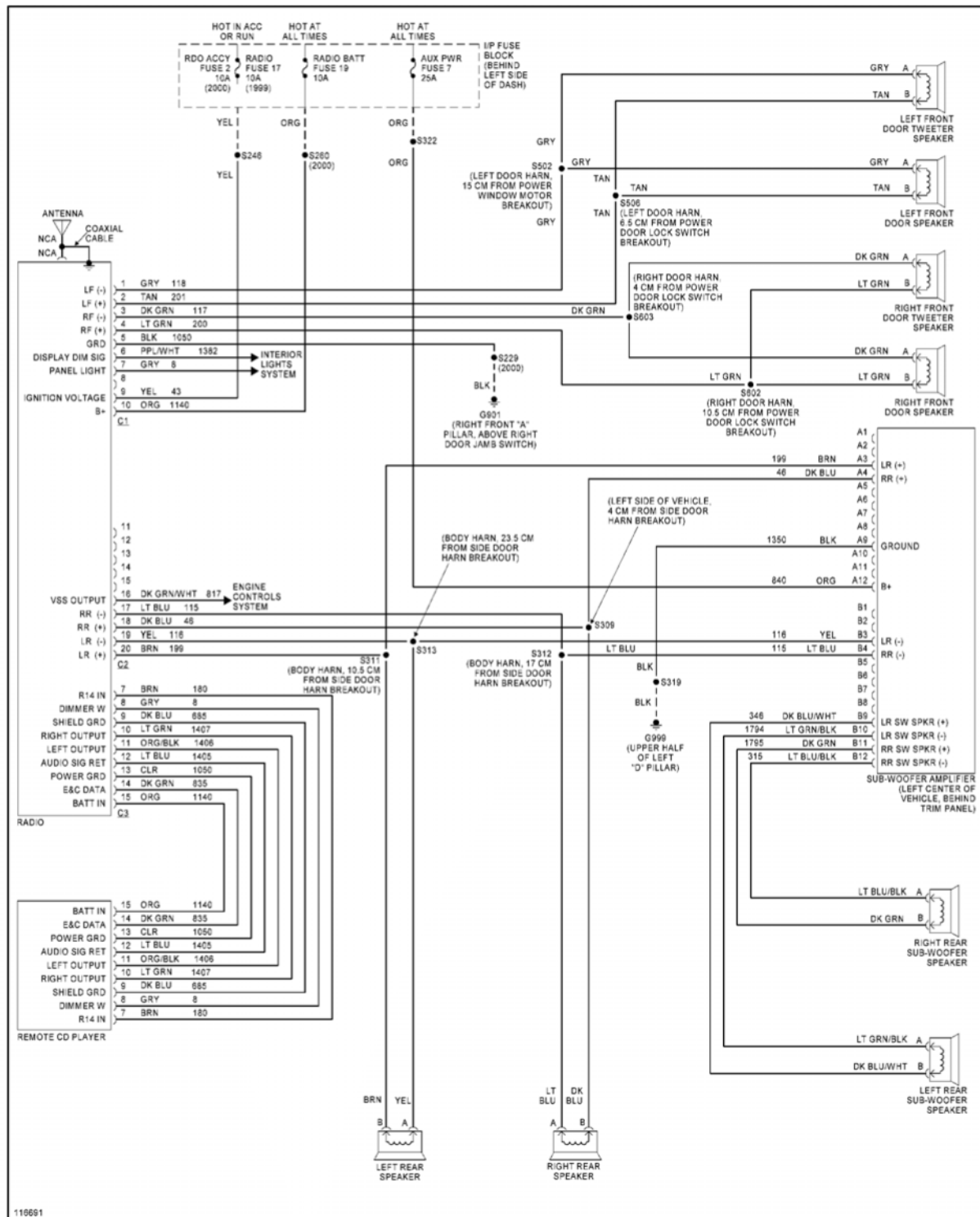
Fig. 36: Premium Sound Radio Circuit, W/O Rear Controls
