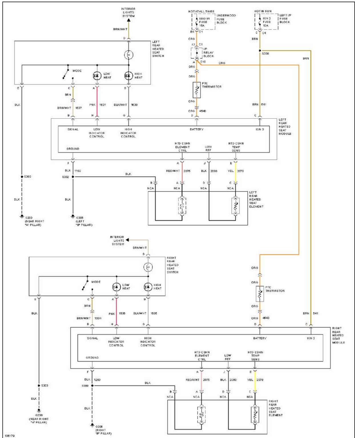
Fig. 67: Rear Heated Seats Circuit
