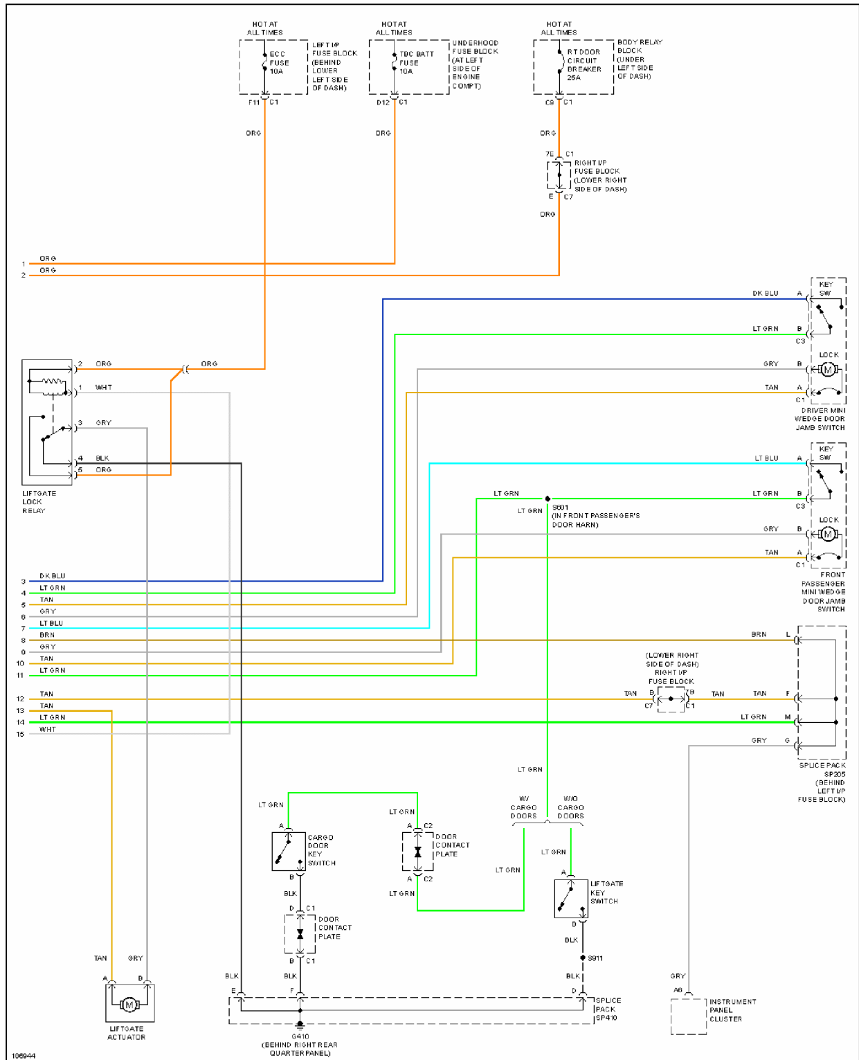
Fig. 59: Power Door Locks Circuit (2 of 2)
