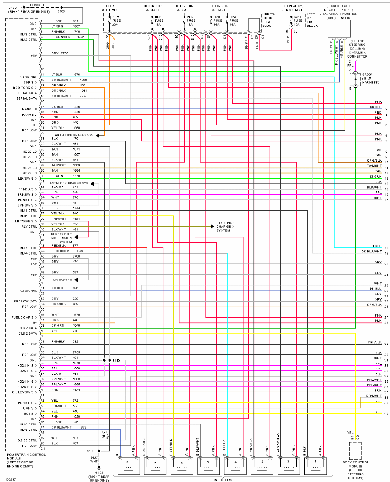
Fig. 23: 6.0L VIN N, Engine Performance Circuit (1 of 5)
