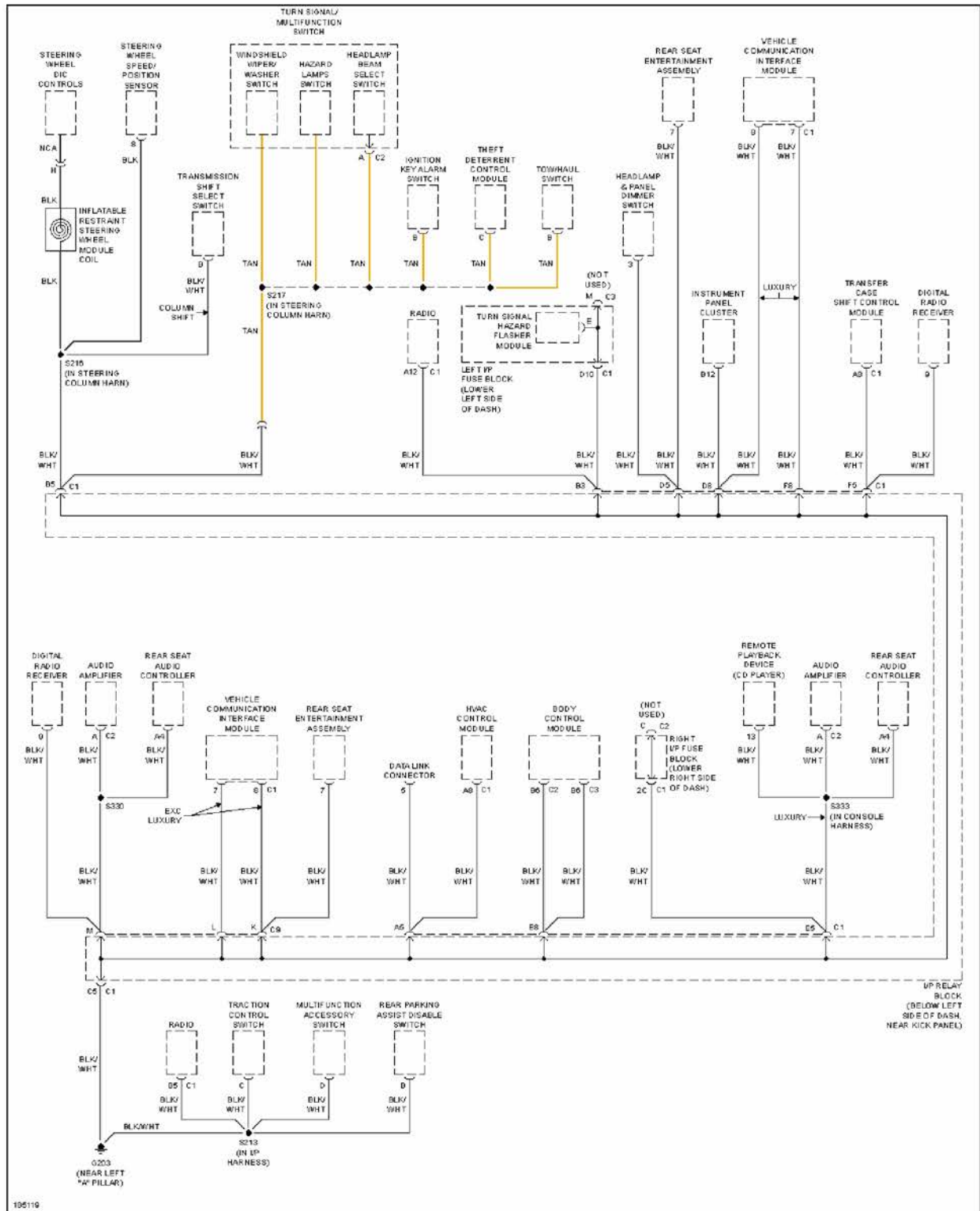
Fig. 35: Ground Distribution Circuit (4 of 5)
