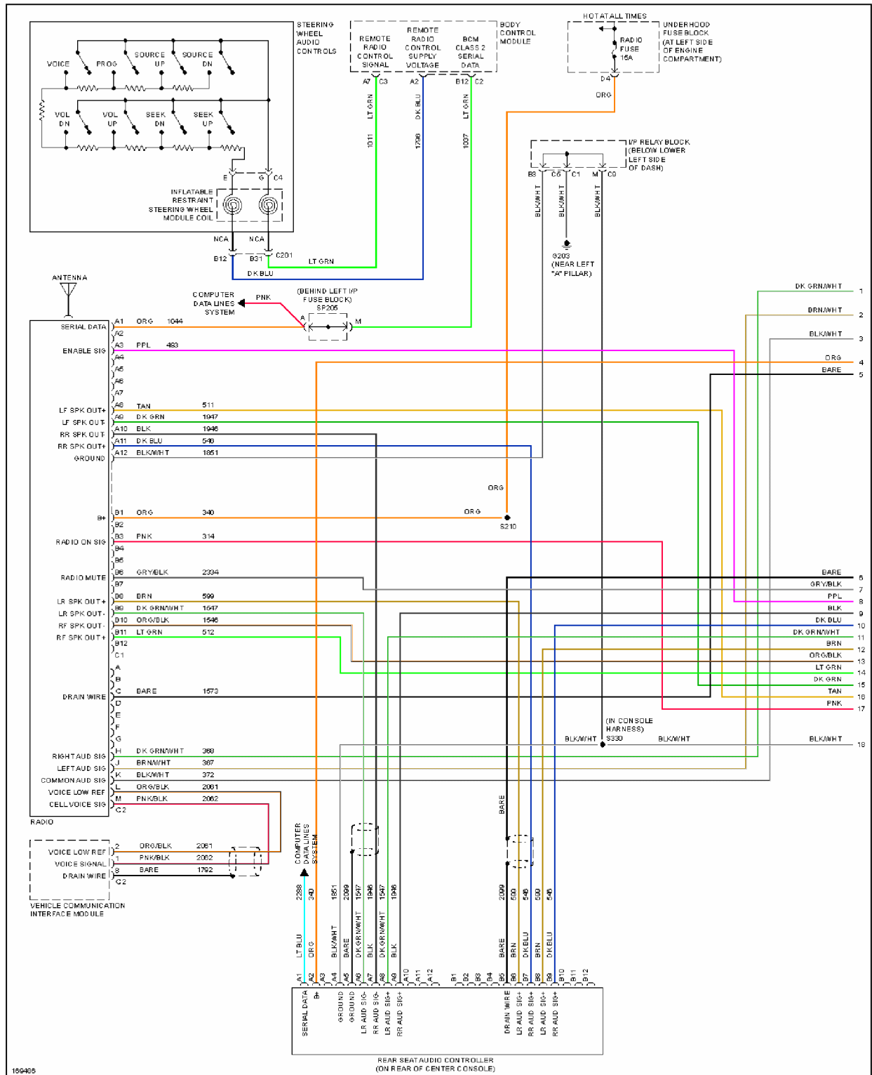
Fig. 71: Mid-Line Radio Circuit, W/ Rear Seat Audio (1 of 3)
