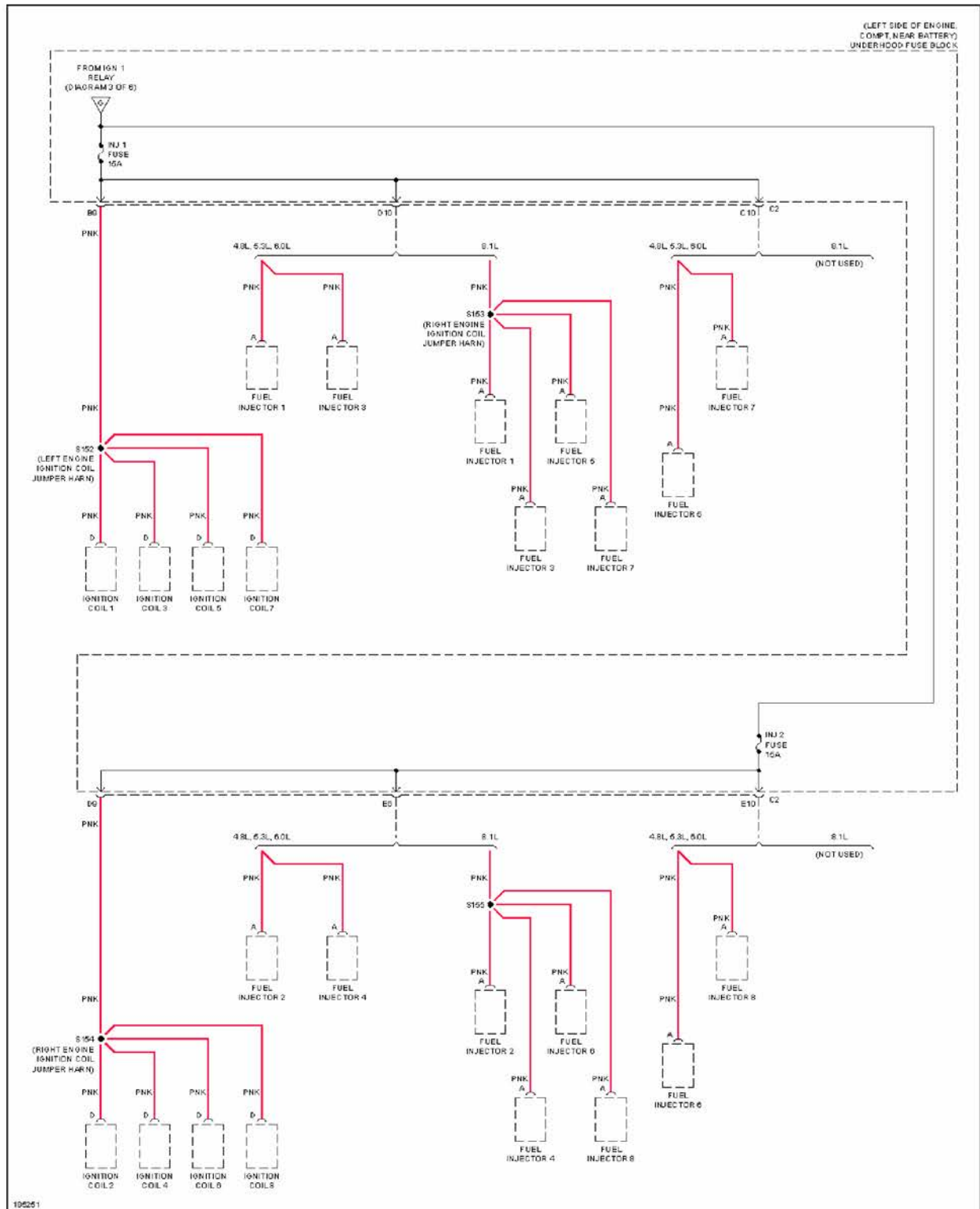
Fig. 55: Power Distribution Circuit (4 of 6)
