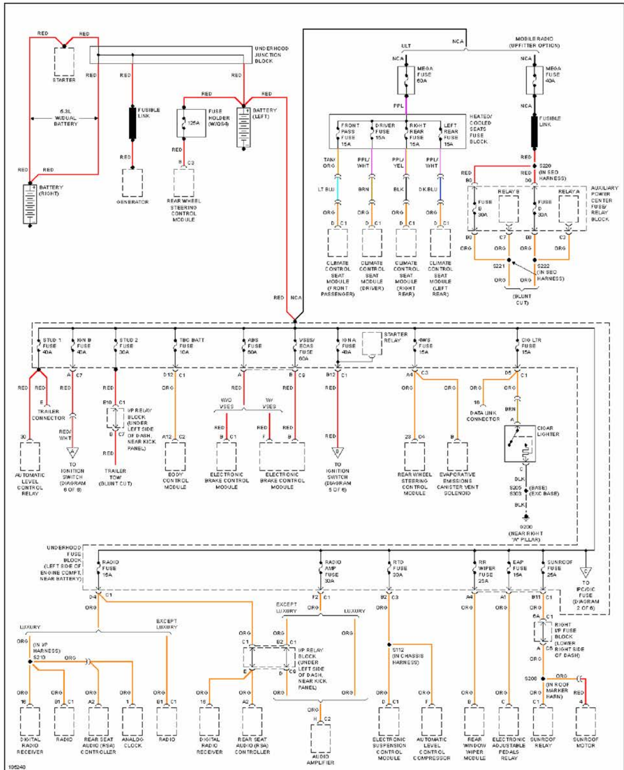
Fig. 52: Power Distribution Circuit (1 of 6)
