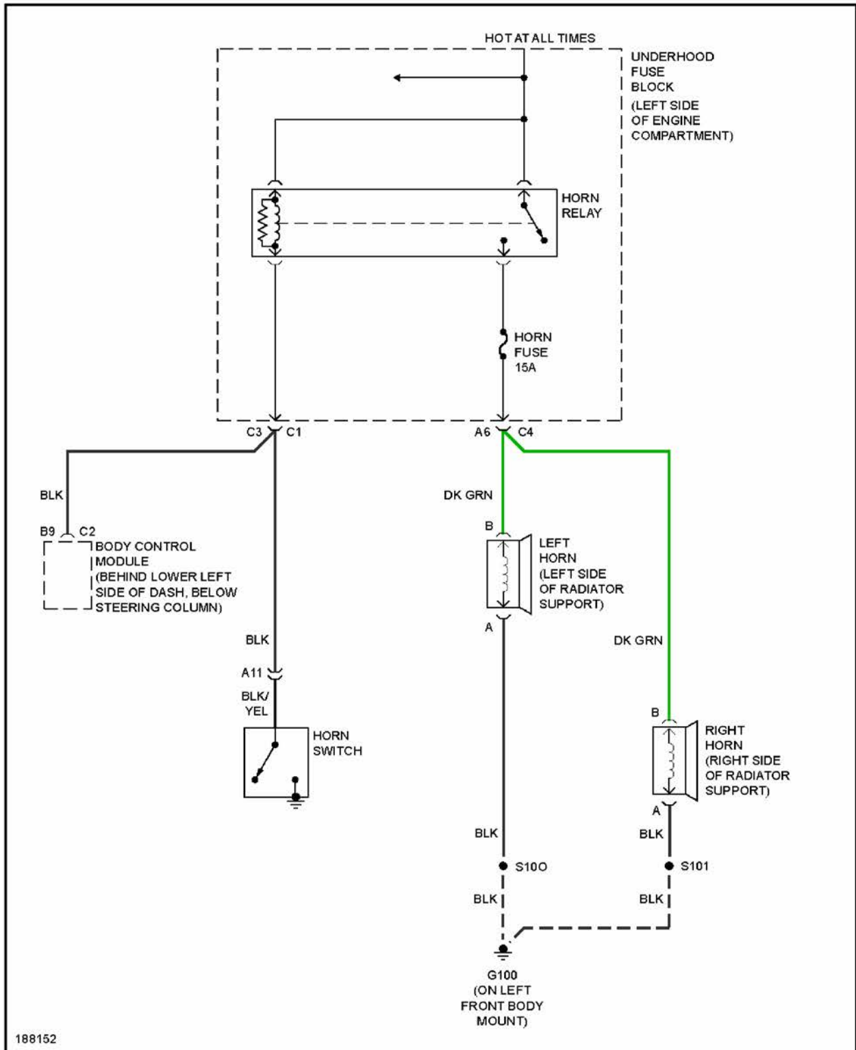
Fig. 38: Horn Circuit
