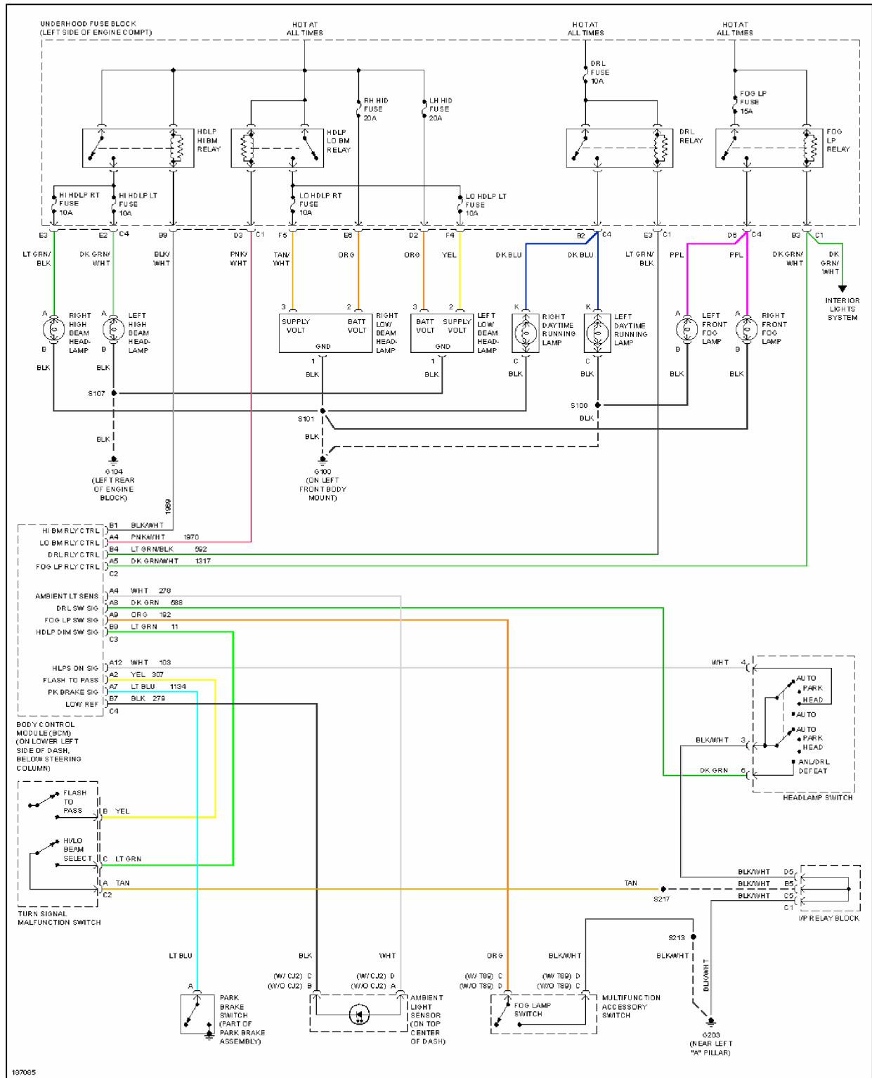
Fig. 37: Headlights Circuit
