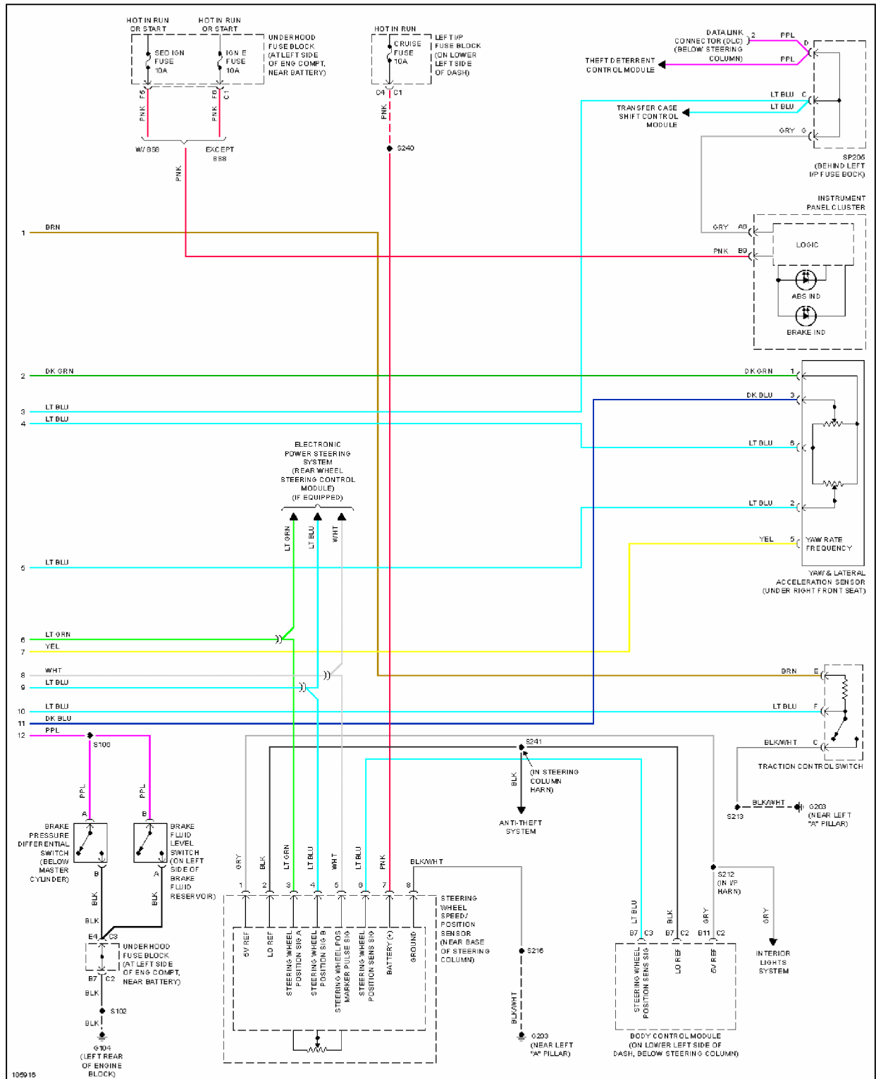
Fig. 6: Anti-lock Brakes Circuit, W/ Vehicle Speed Enhancement Stability (2 of 2)
