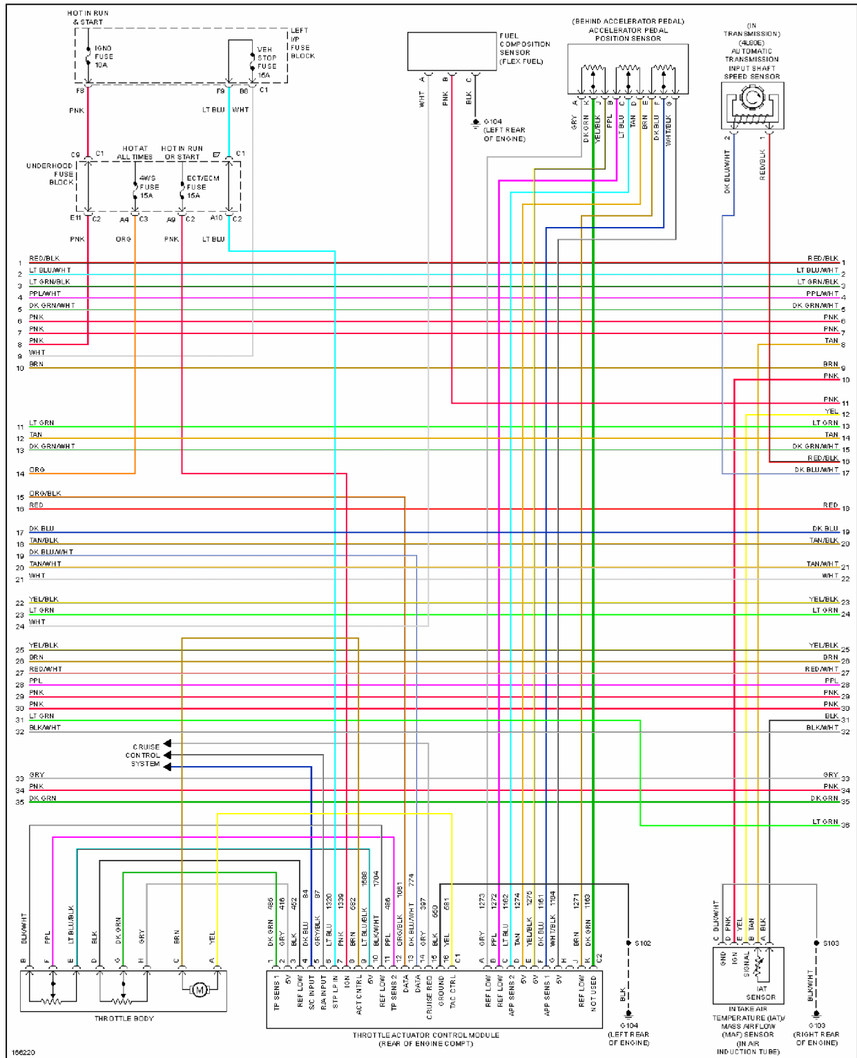
Fig. 26: 6.0L VIN N, Engine Performance Circuit (4 of 5)
