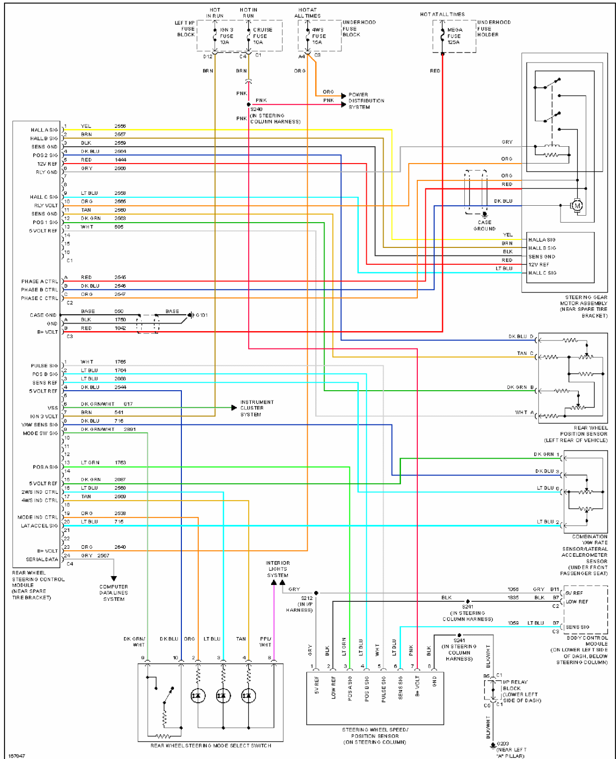
Fig. 16: Rear Wheel Steering Circuit
