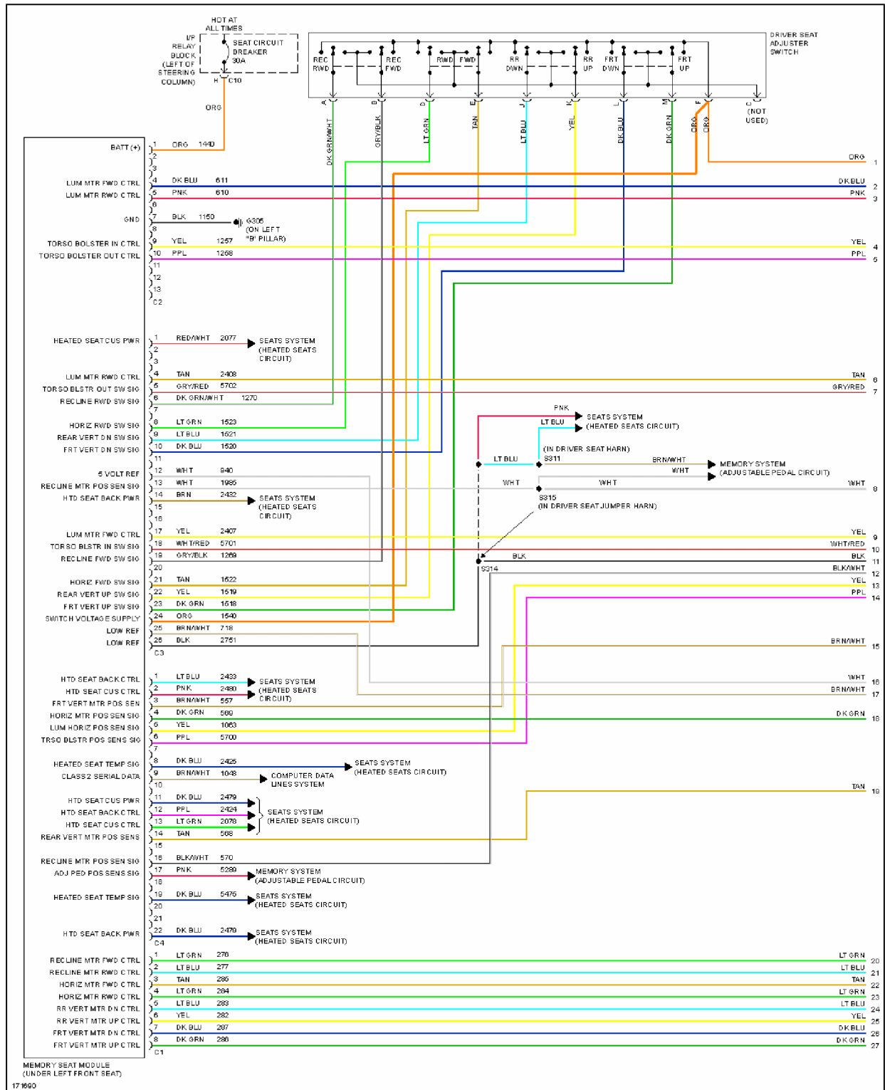
Fig. 49: Memory Seat Circuit (1 of 2)
