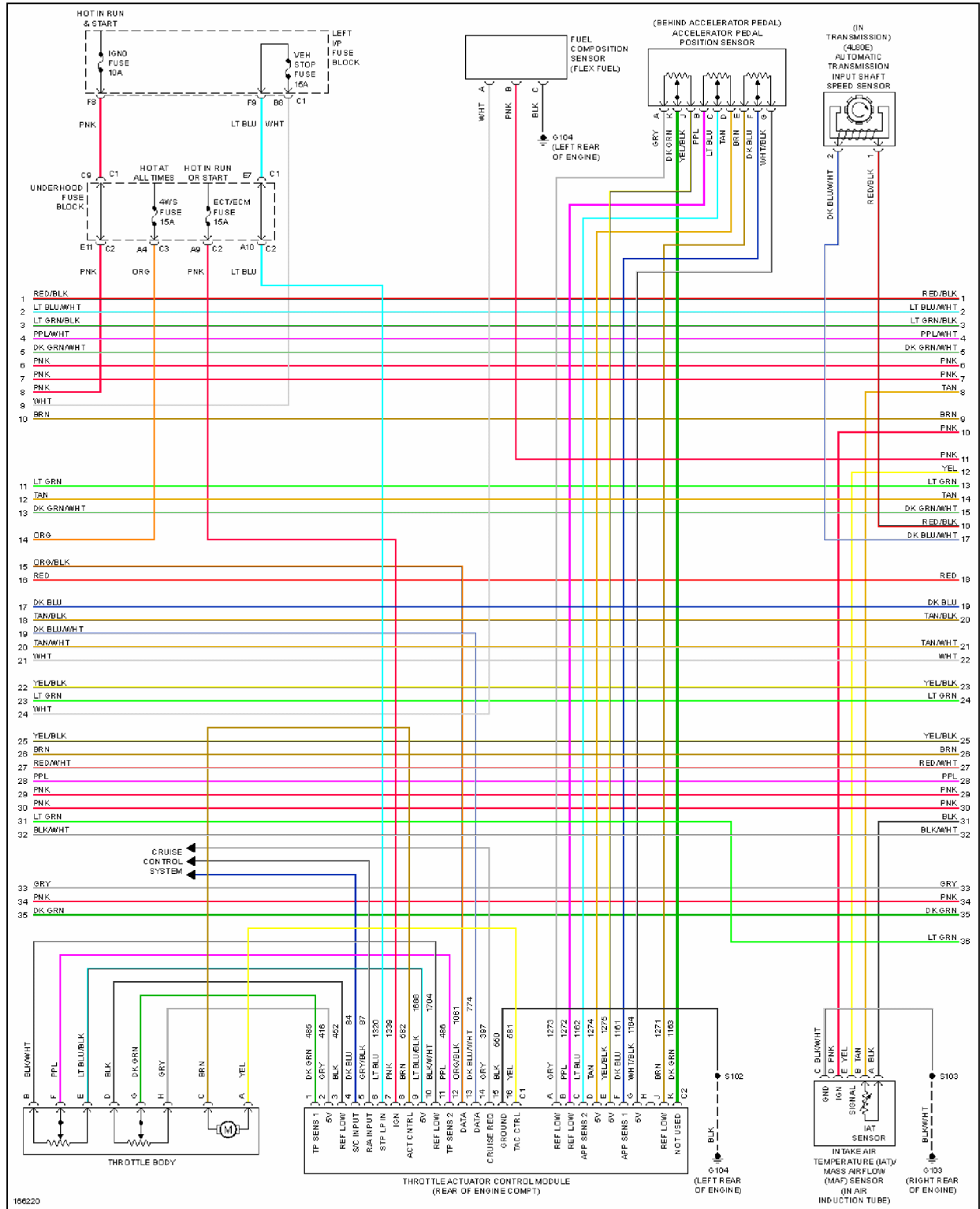
Fig. 21: 5.3L VIN T, Engine Performance Circuit (4 of 5)
