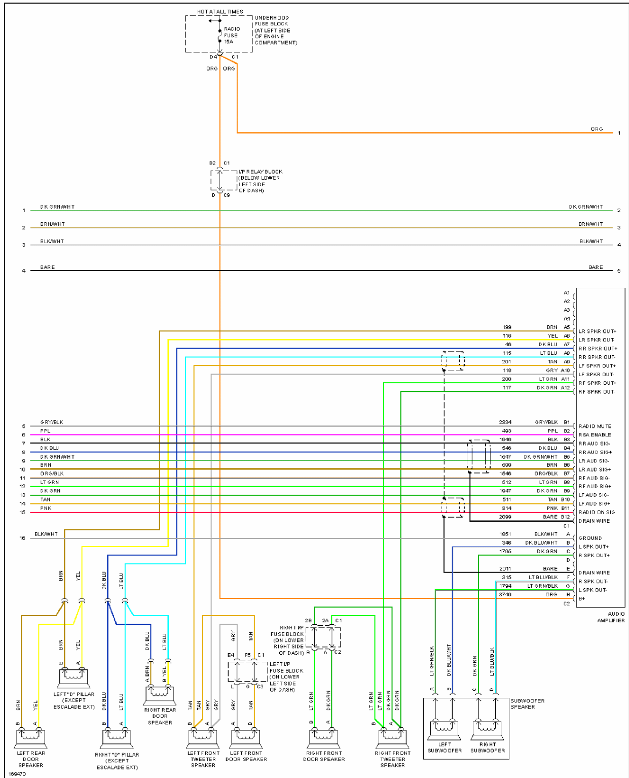
Fig. 75: Mid-Line Radio Circuit, W/O Rear Seat Audio (2 of 3)
