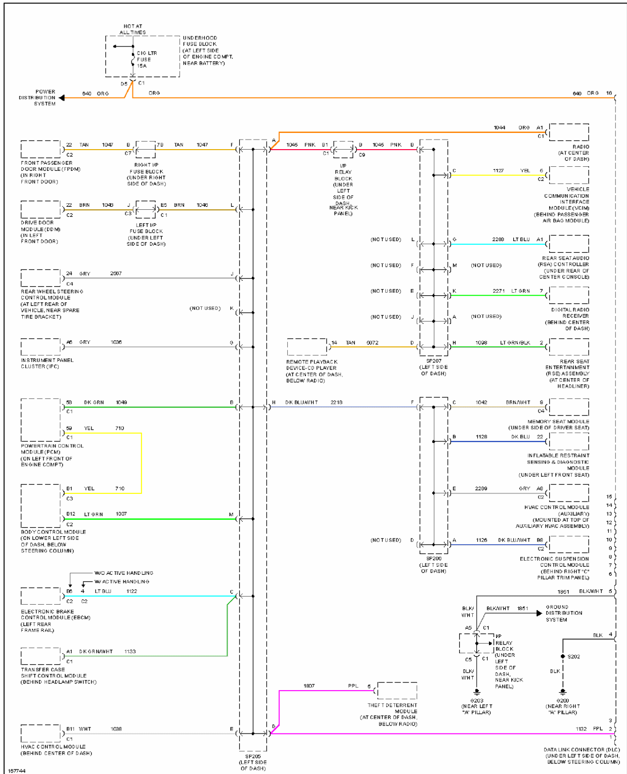
Fig. 11: Computer Data Lines Circuit, Base & Up-Level
