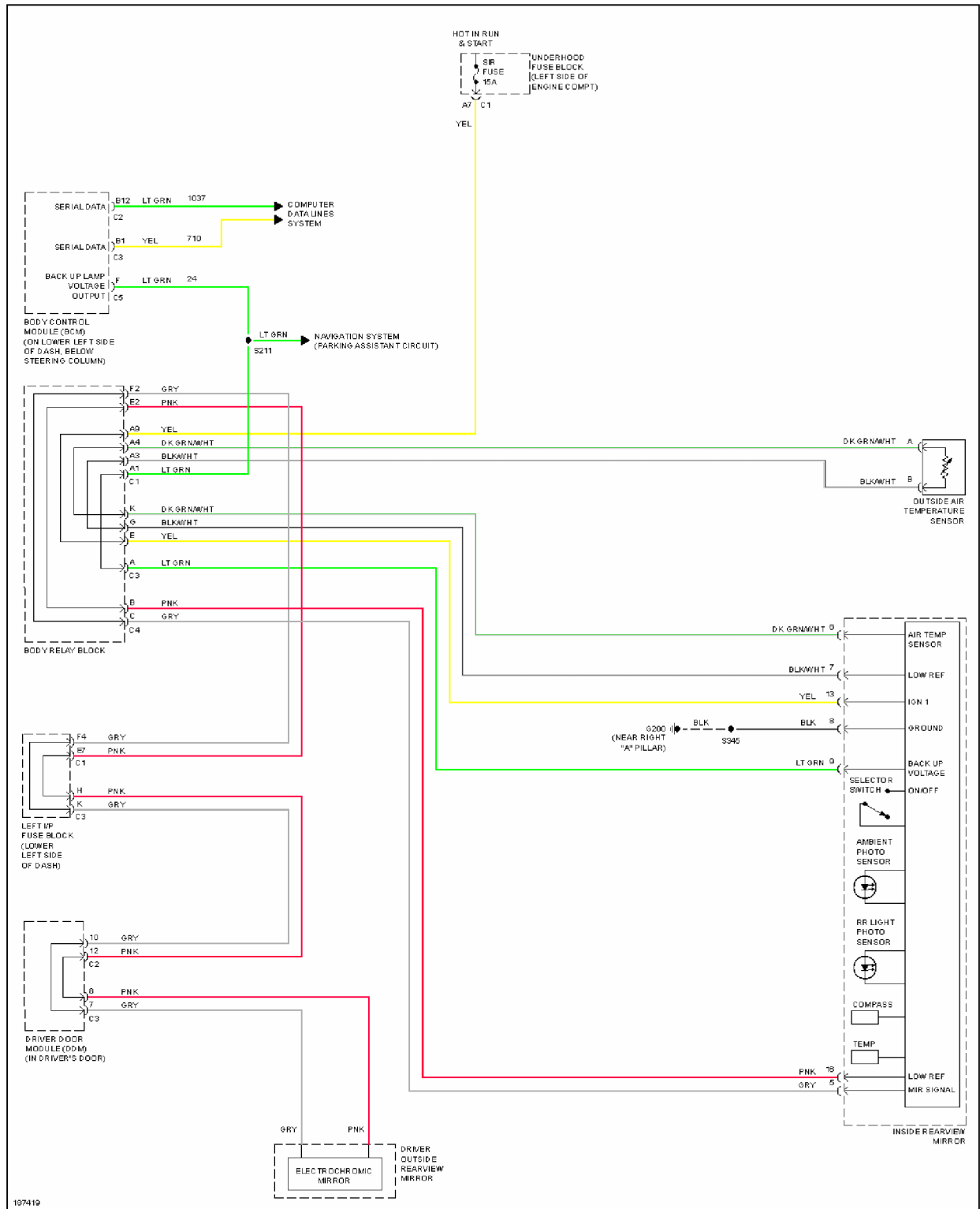
Fig. 60: Electrochromic Mirror Circuit
