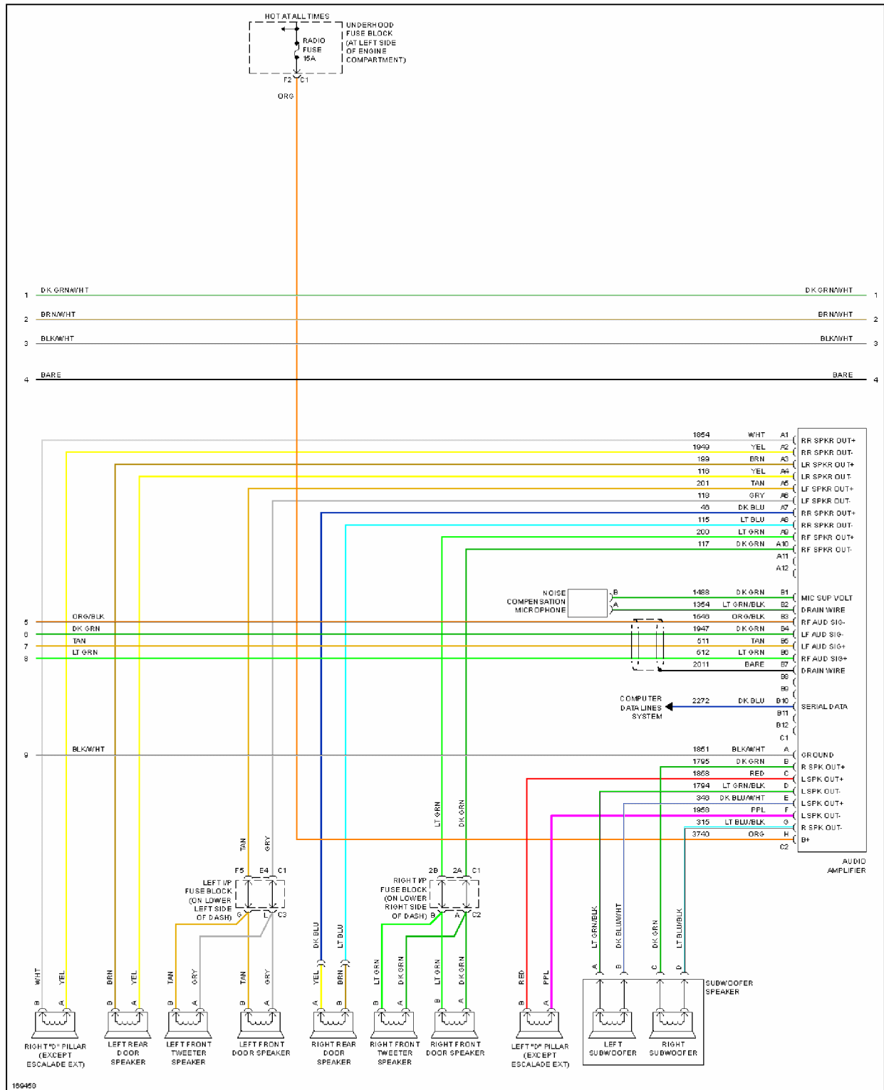
Fig. 78: Premium Sound Radio Circuit, W/ CD, W/ Rear Entertainment, W/ Digital Receiver (2 of 3)
