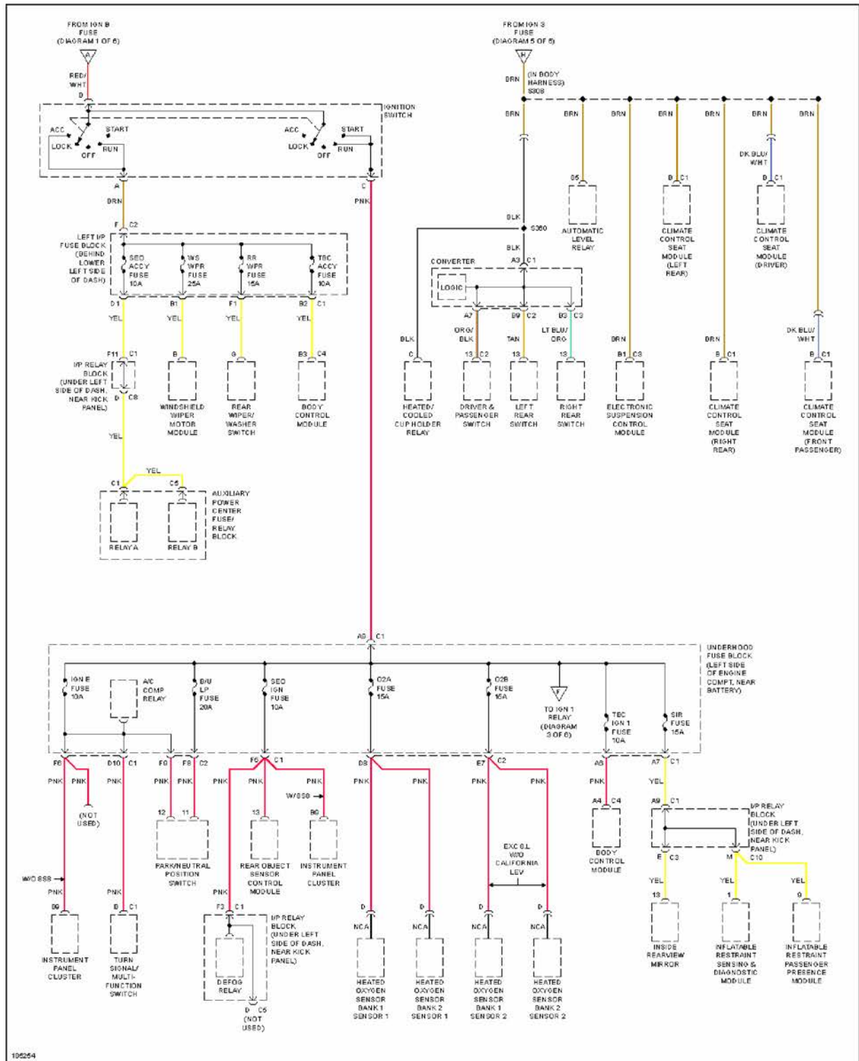
Fig. 57: Power Distribution Circuit (6 of 6)
