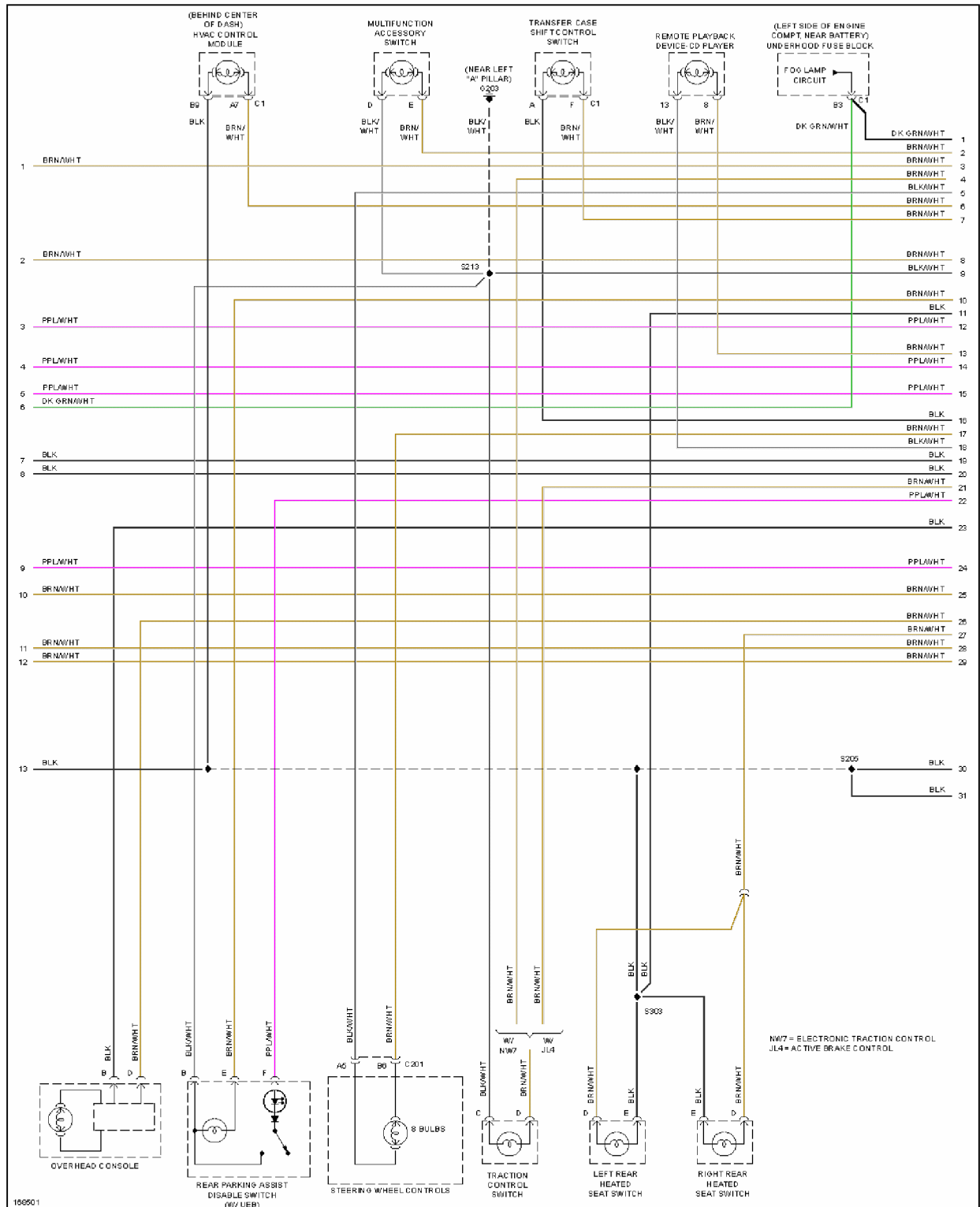
Fig. 45: Instrument Illumination Circuit (2 of 3)
