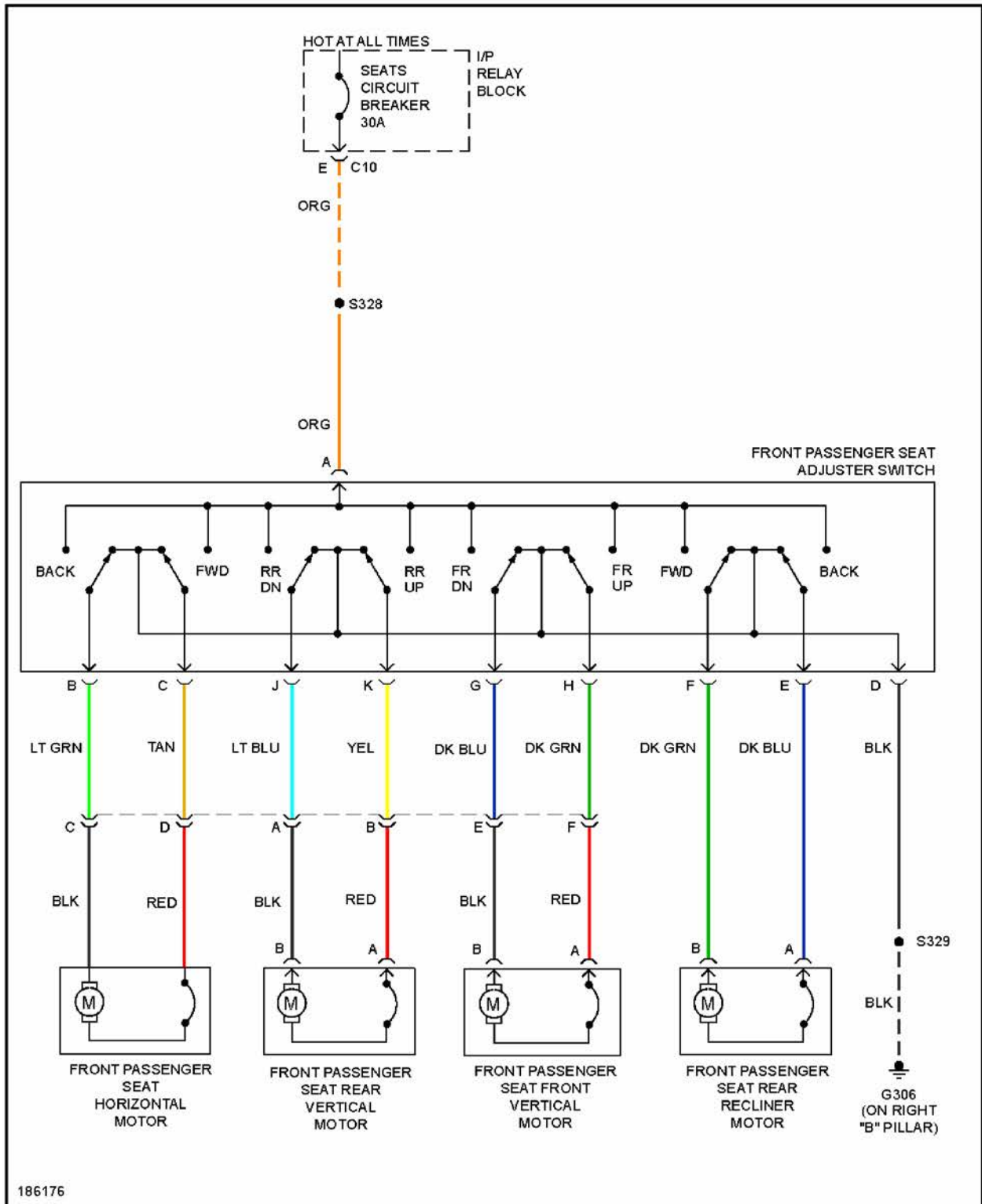
Fig. 64: Passenger Full Feature Seat Circuit
