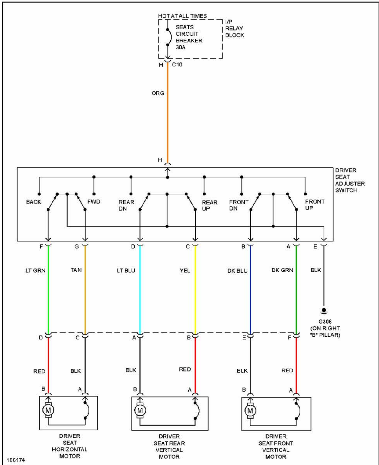
Fig. 62: Driver Seat Circuit
