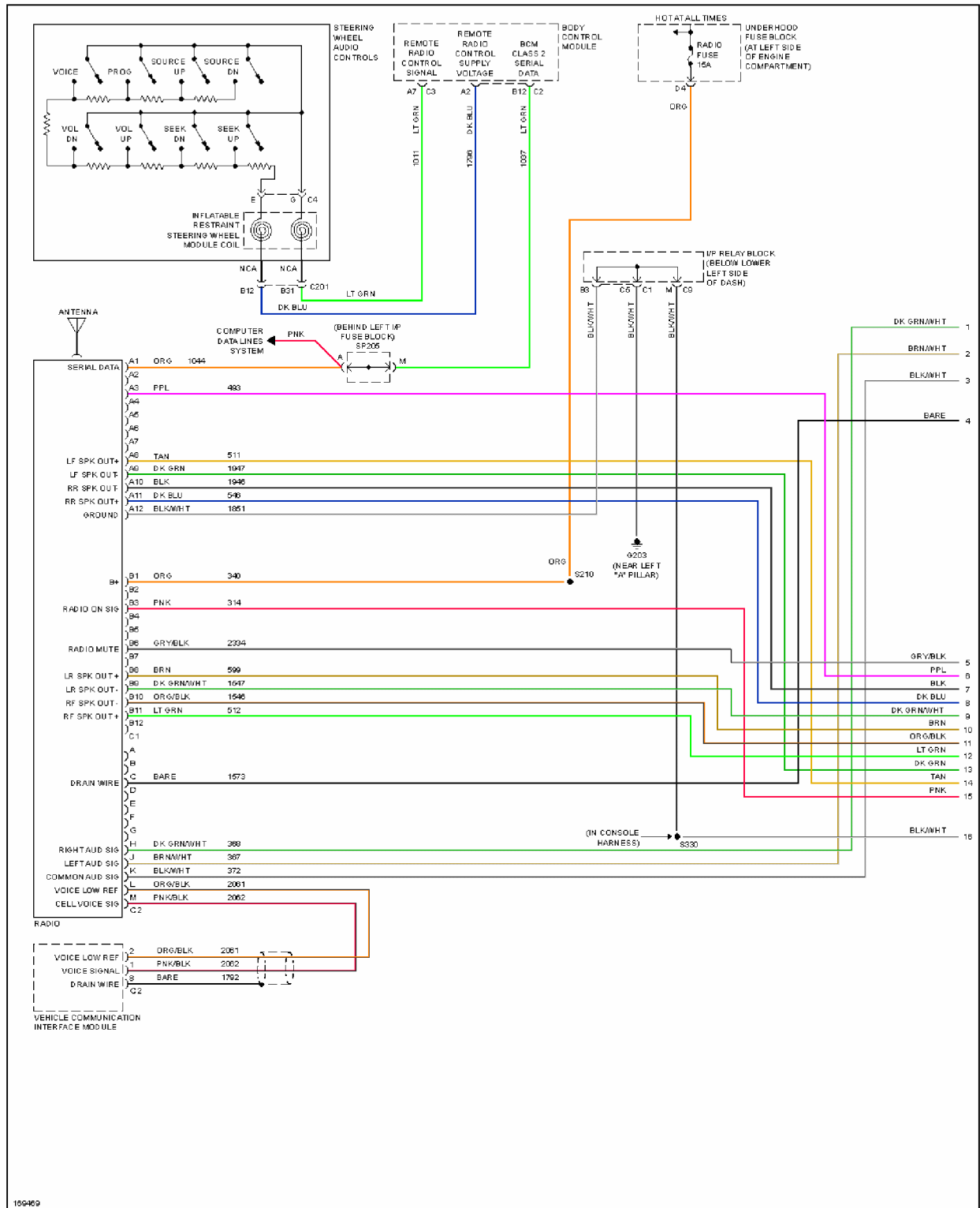
Fig. 74: Mid-Line Radio Circuit, W/O Rear Seat Audio (1 of 3)
