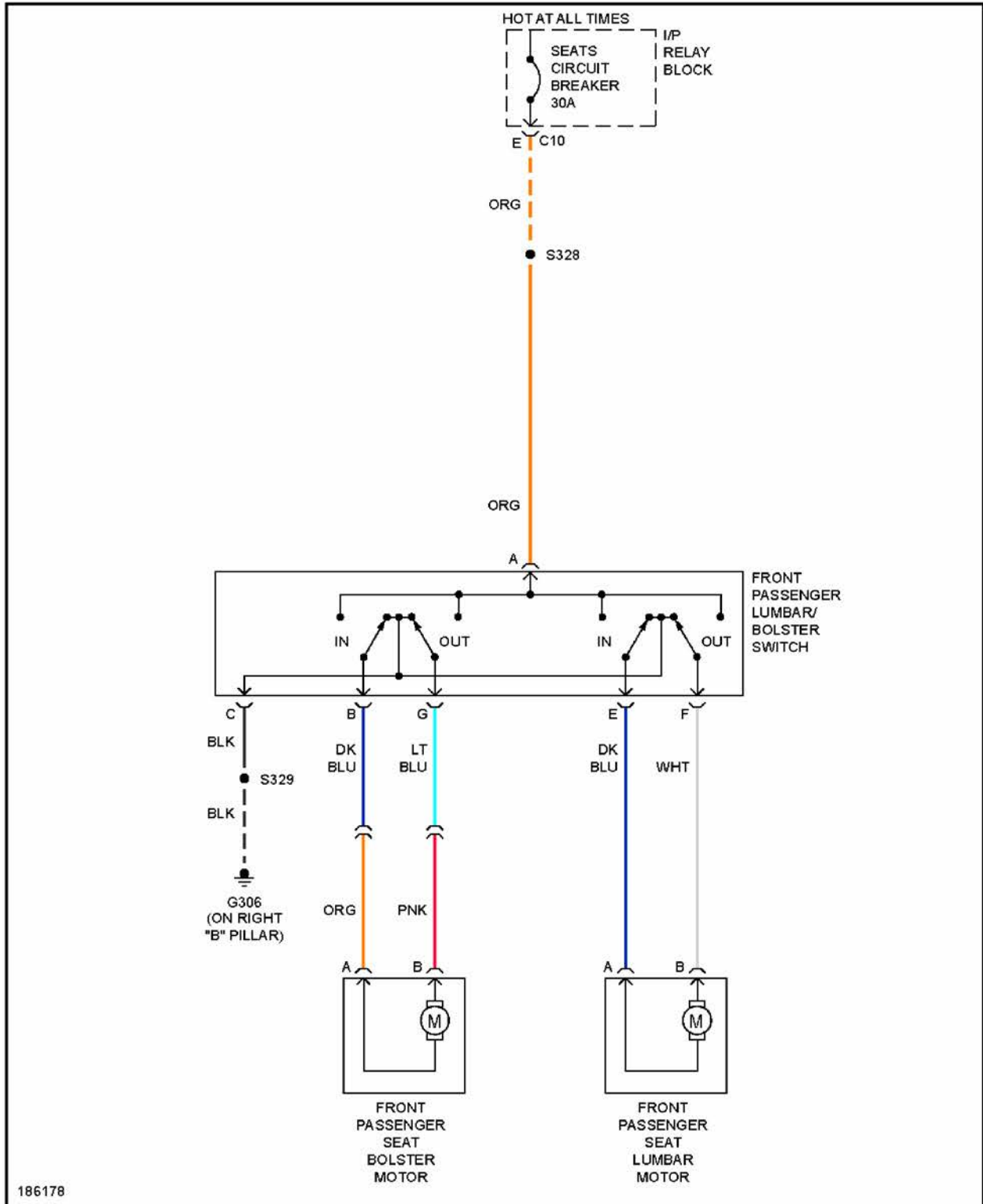
Fig. 66: Passenger's Lumbar Circuit
