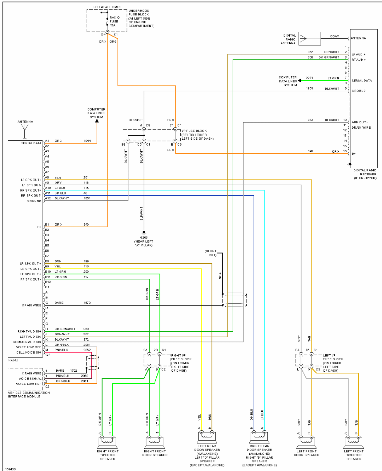
Fig. 70: Base Radio Circuit
