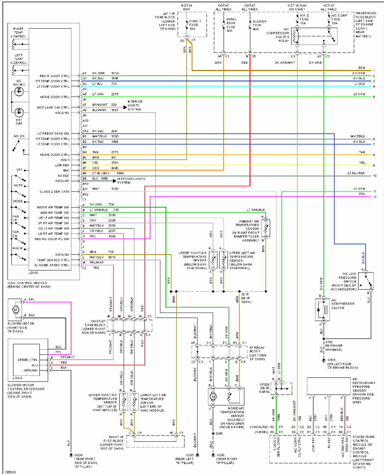
Fig. 1: Automatic A/C Circuit, Front A/C (1 of 2)
