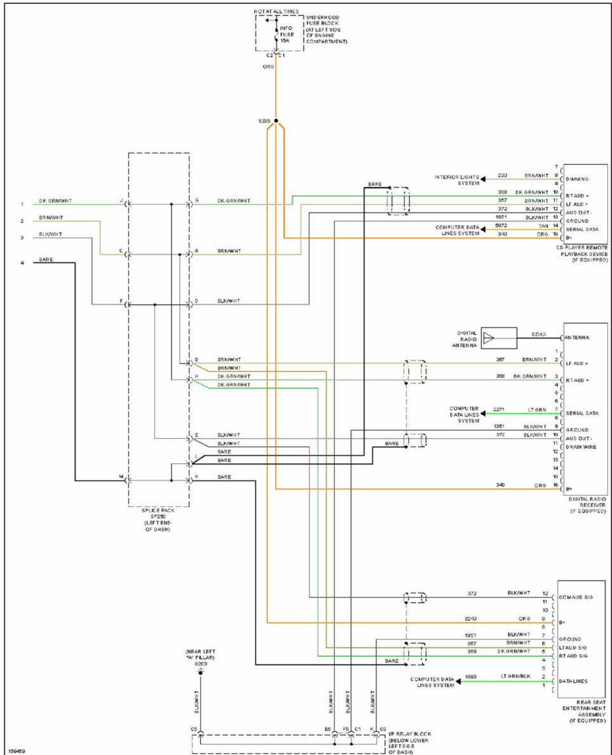
Fig. 79: Premium Sound Radio Circuit, W/ CD, W/ Rear Entertainment, W/ Digital Receiver (3 of 3)
