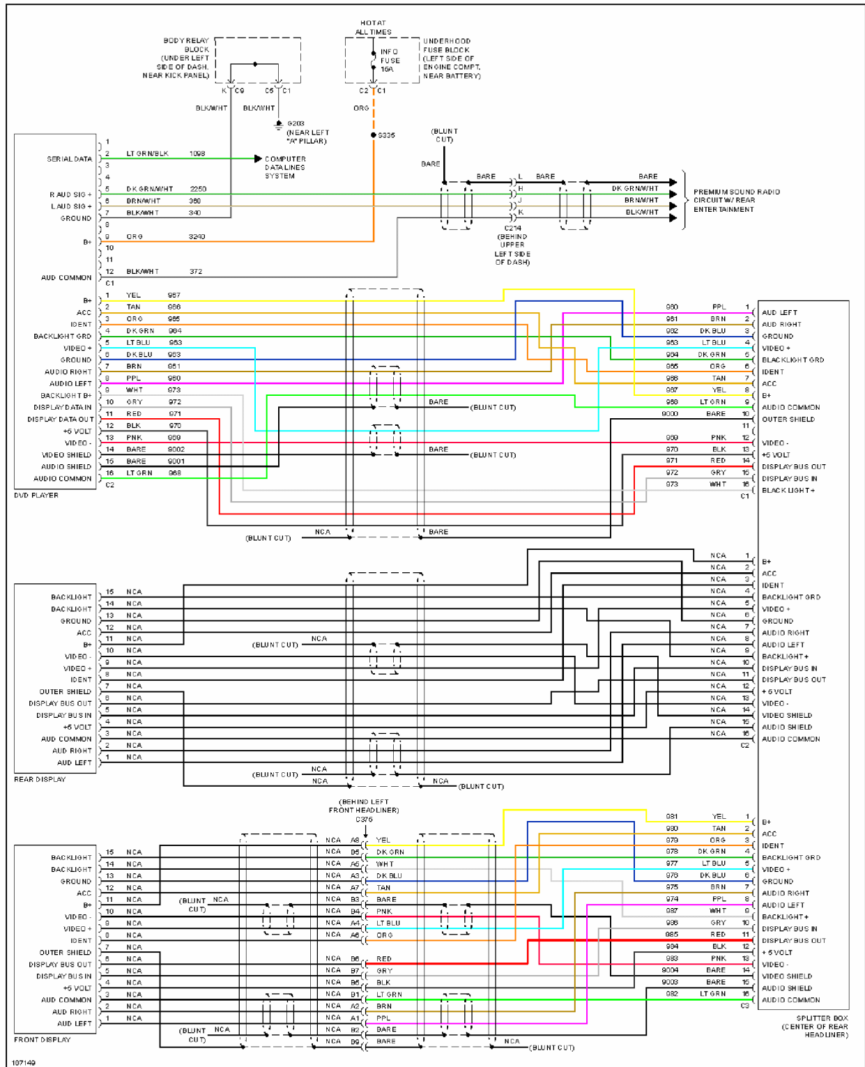
Fig. 86: Video System Circuit
