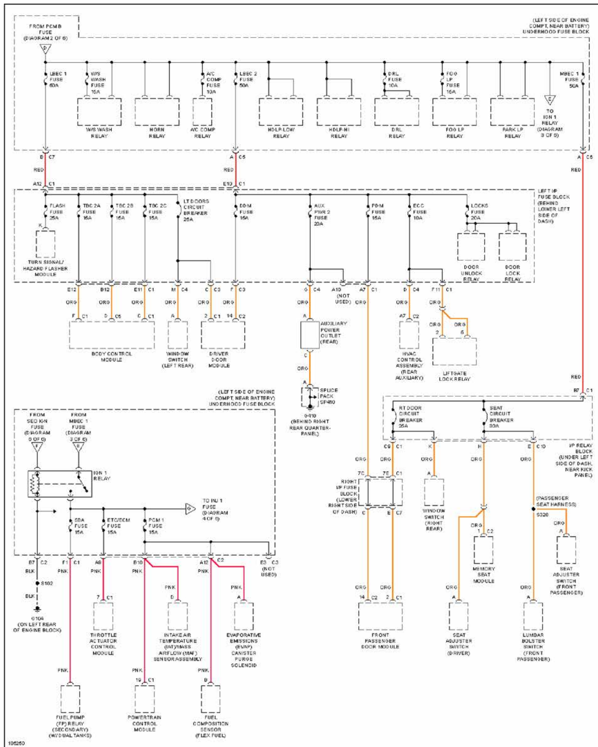
Fig. 54: Power Distribution Circuit (3 of 6)
