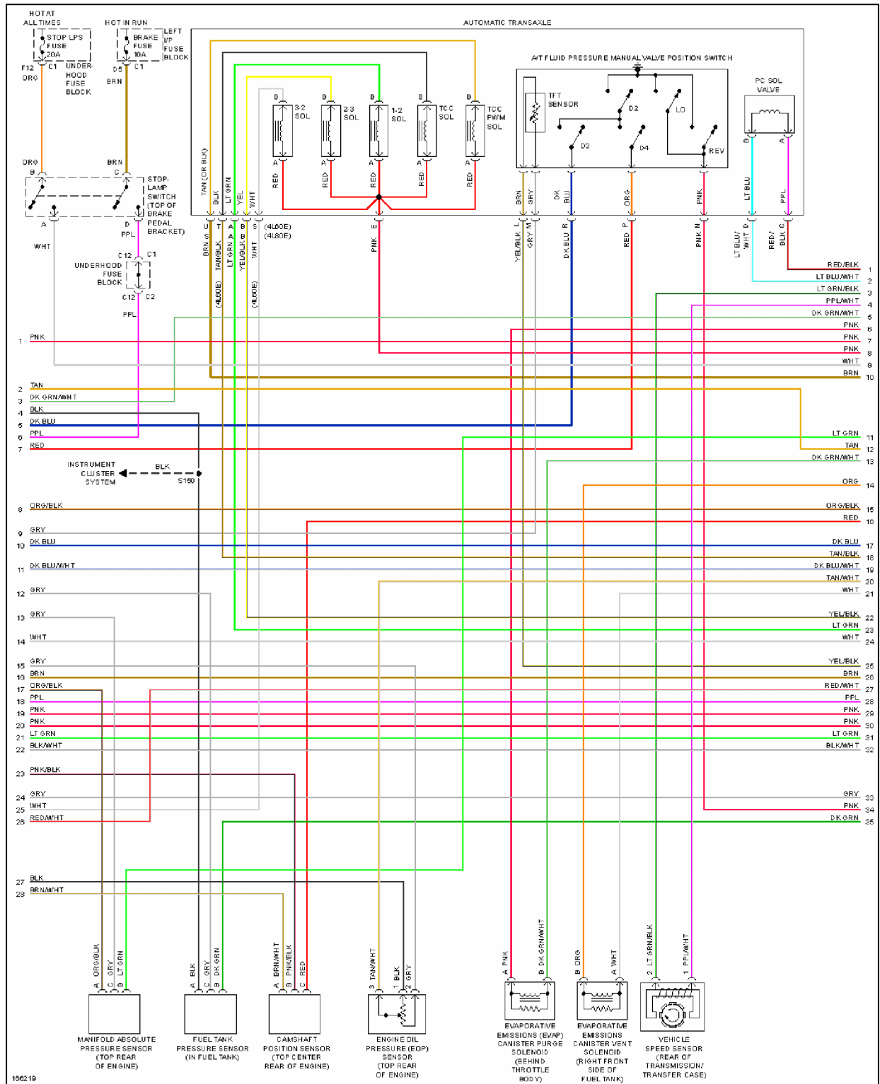
Fig. 20: 5.3L VIN T, Engine Performance Circuit (3 of 5)
