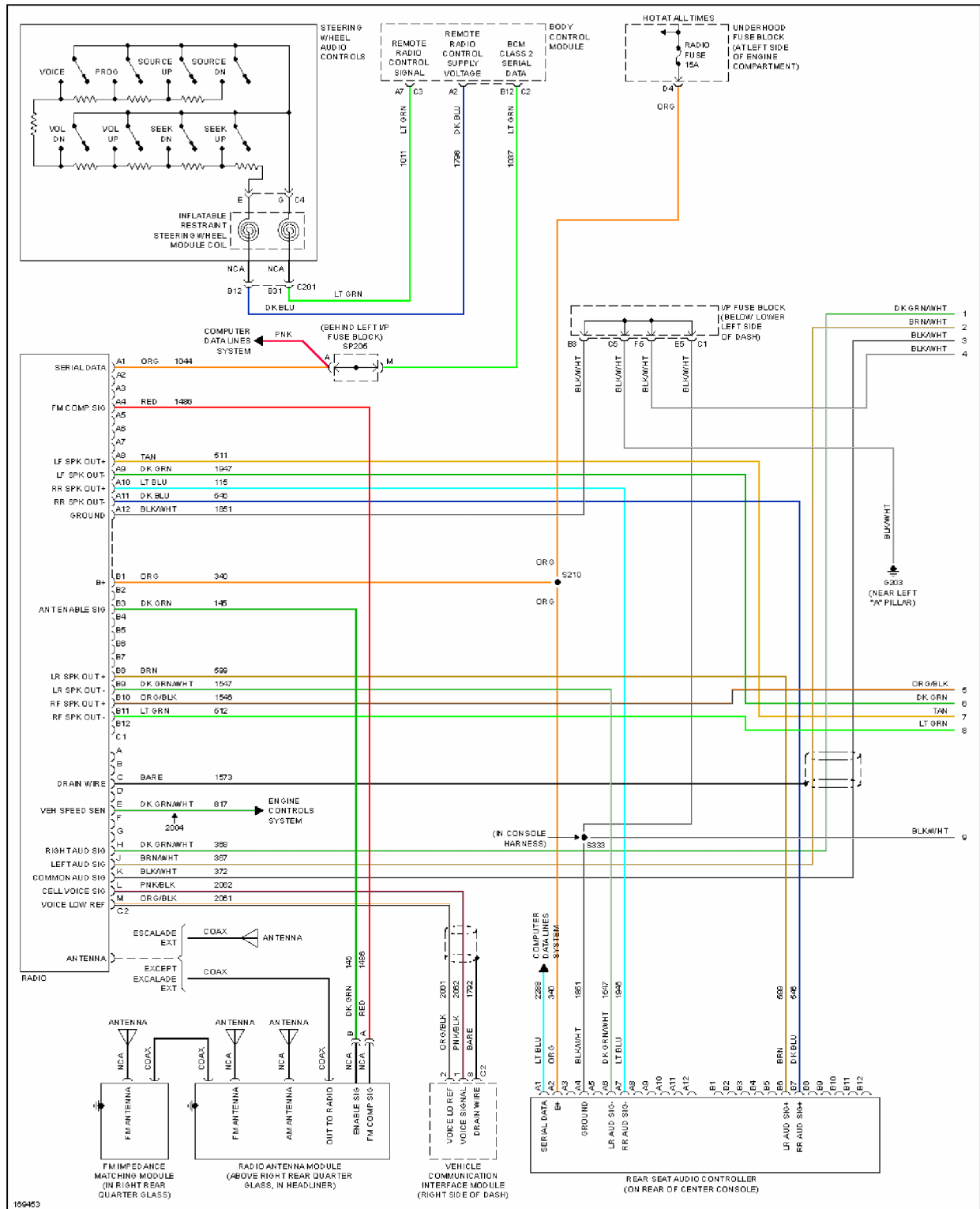
Fig. 80: Premium Sound Radio Circuit, W/ CD (1 of 2)
