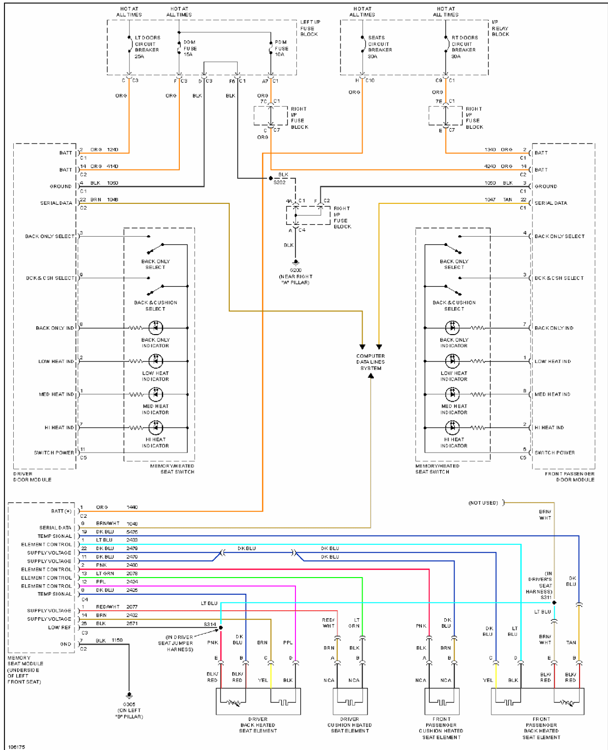
Fig. 63: Front Seat Heater Circuit
