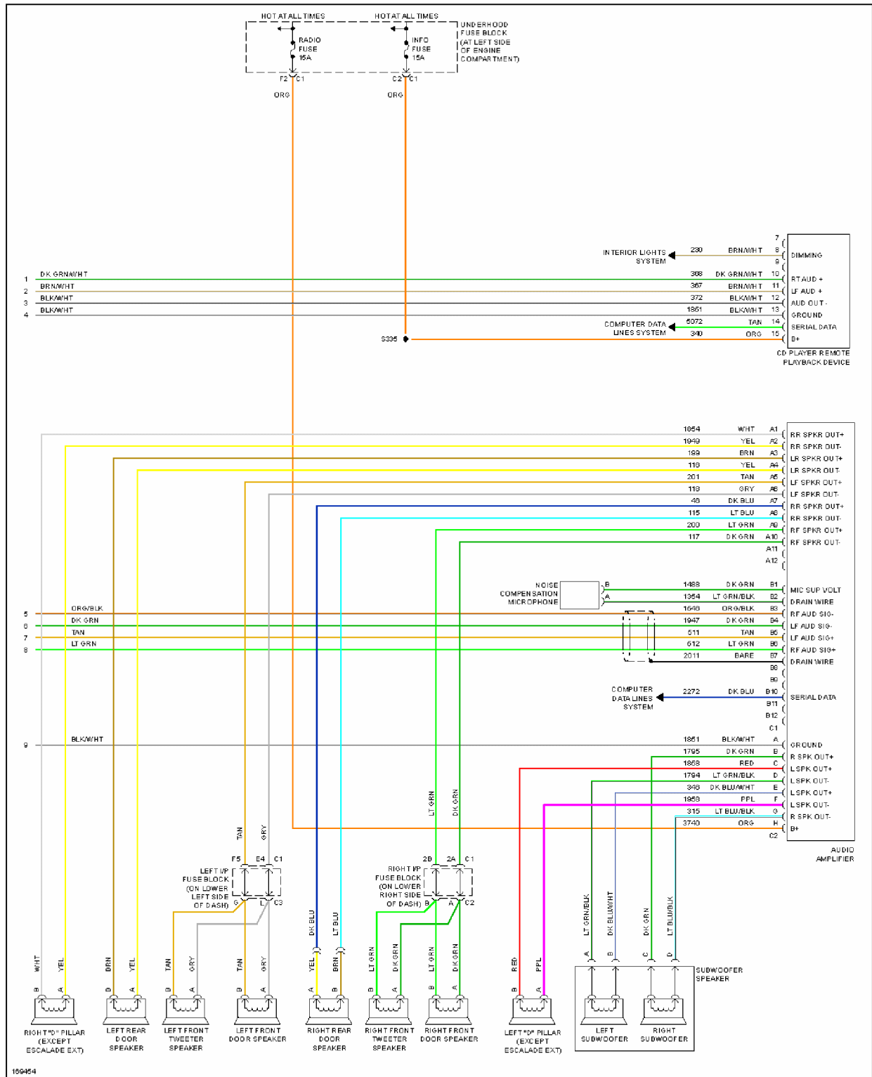
Fig. 81: Premium Sound Radio Circuit, W/ CD (2 of 2)
