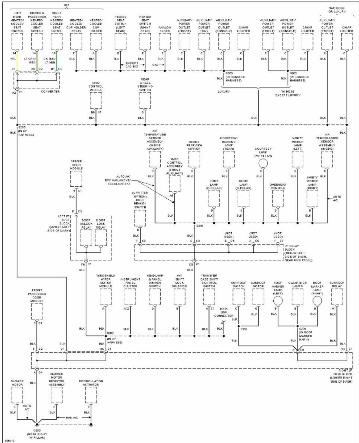
Fig. 34: Ground Distribution Circuit (3 of 5)
