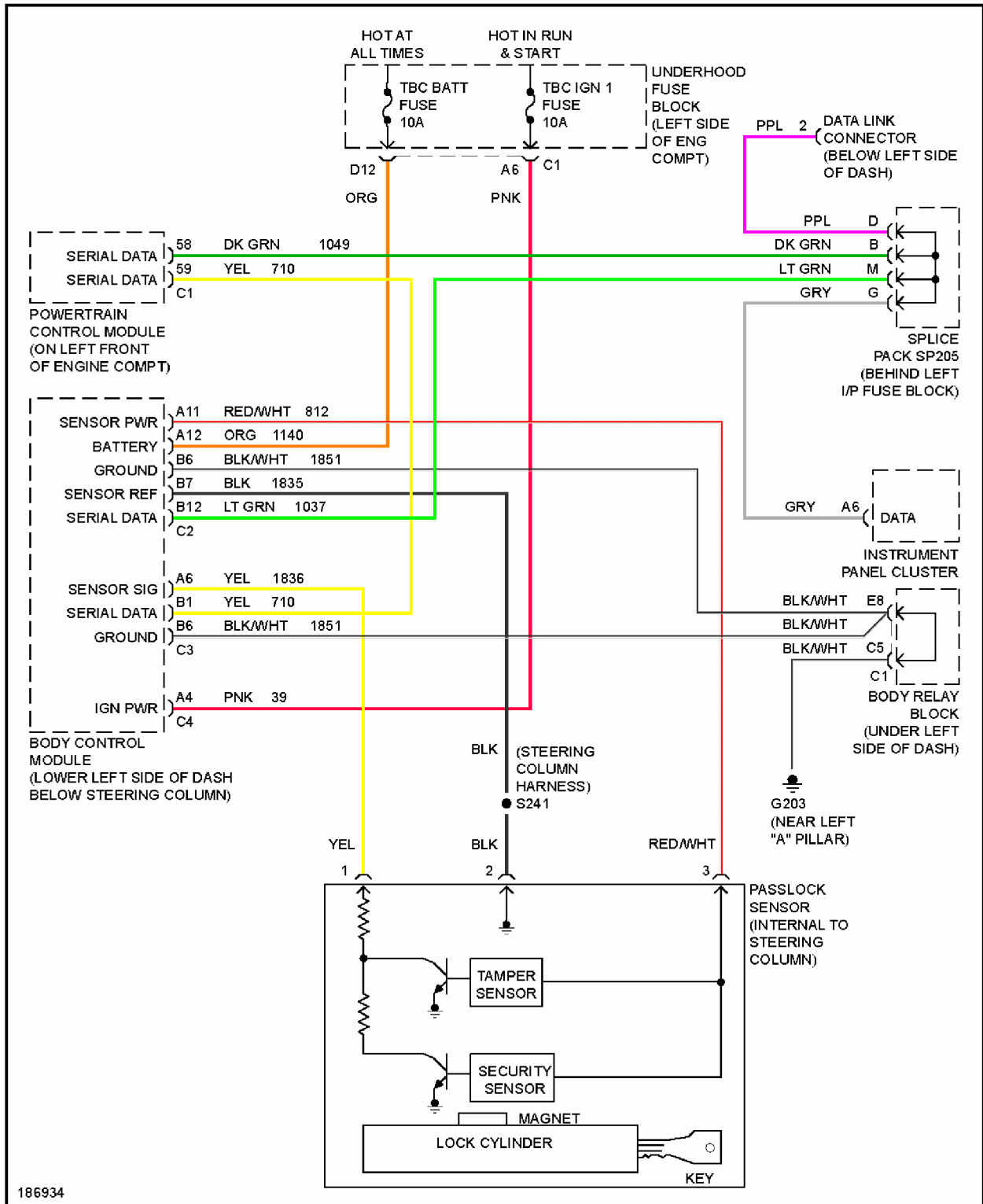
Fig. 8: Passlock Circuit
