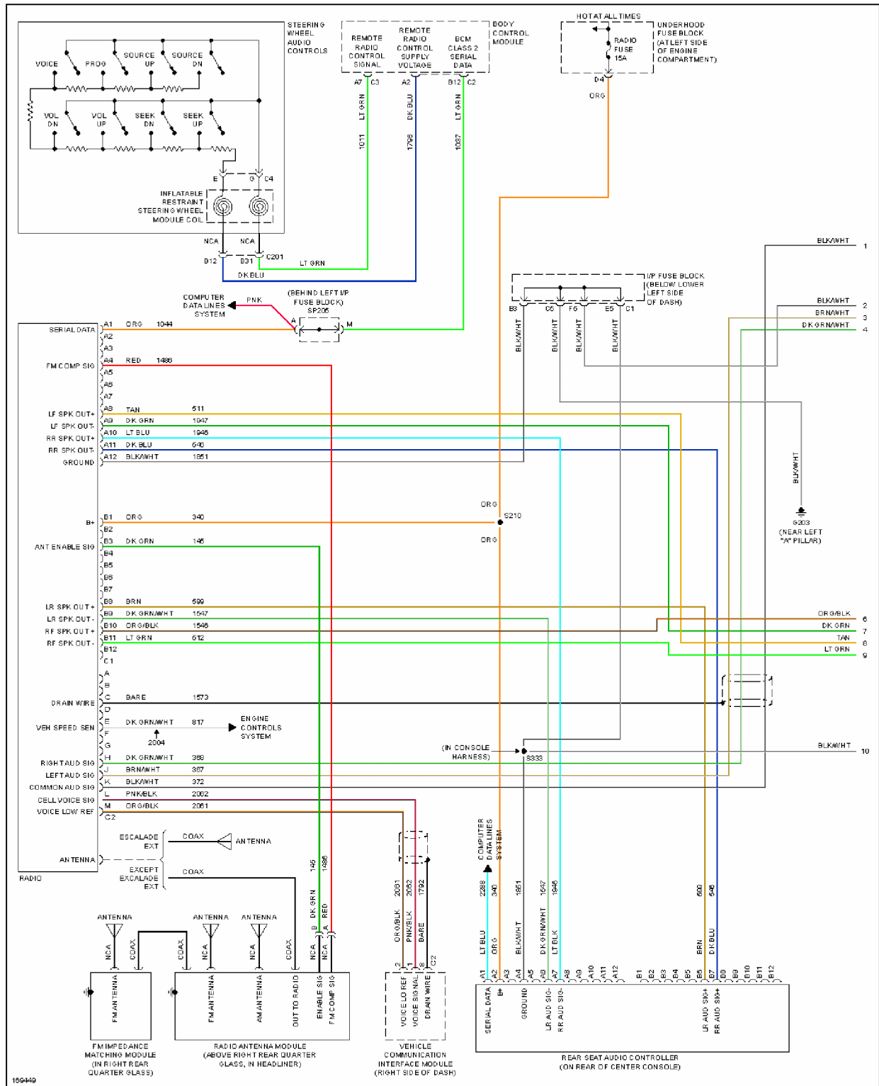
Fig. 84: Premium Sound Radio Circuit, W/ Rear Entertainment (1 of 2)
