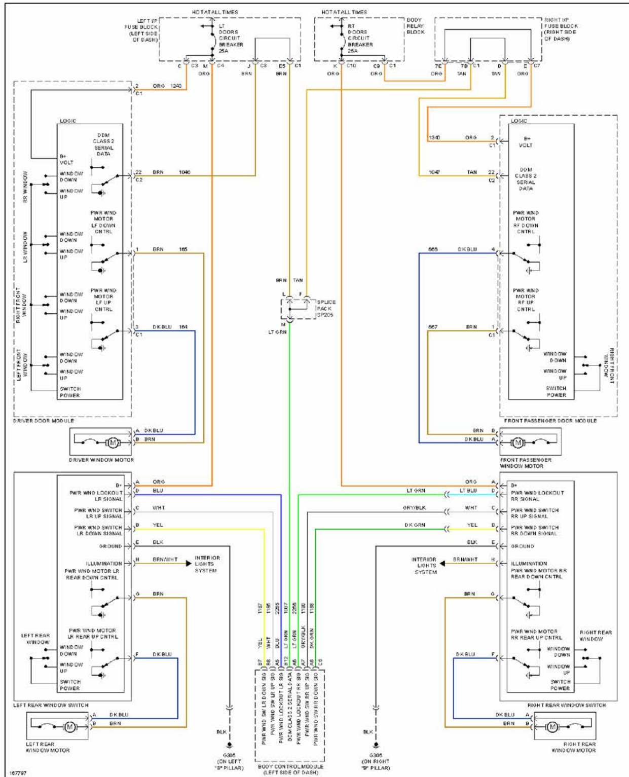
Fig. 69: Power Windows Circuit
