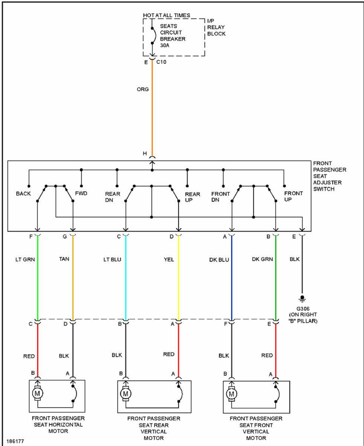
Fig. 65: Passenger Power Seat Circuit
