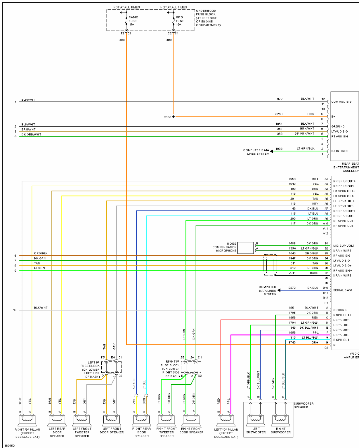
Fig. 85: Premium Sound Radio Circuit, W/ Rear Entertainment (2 of 2)
