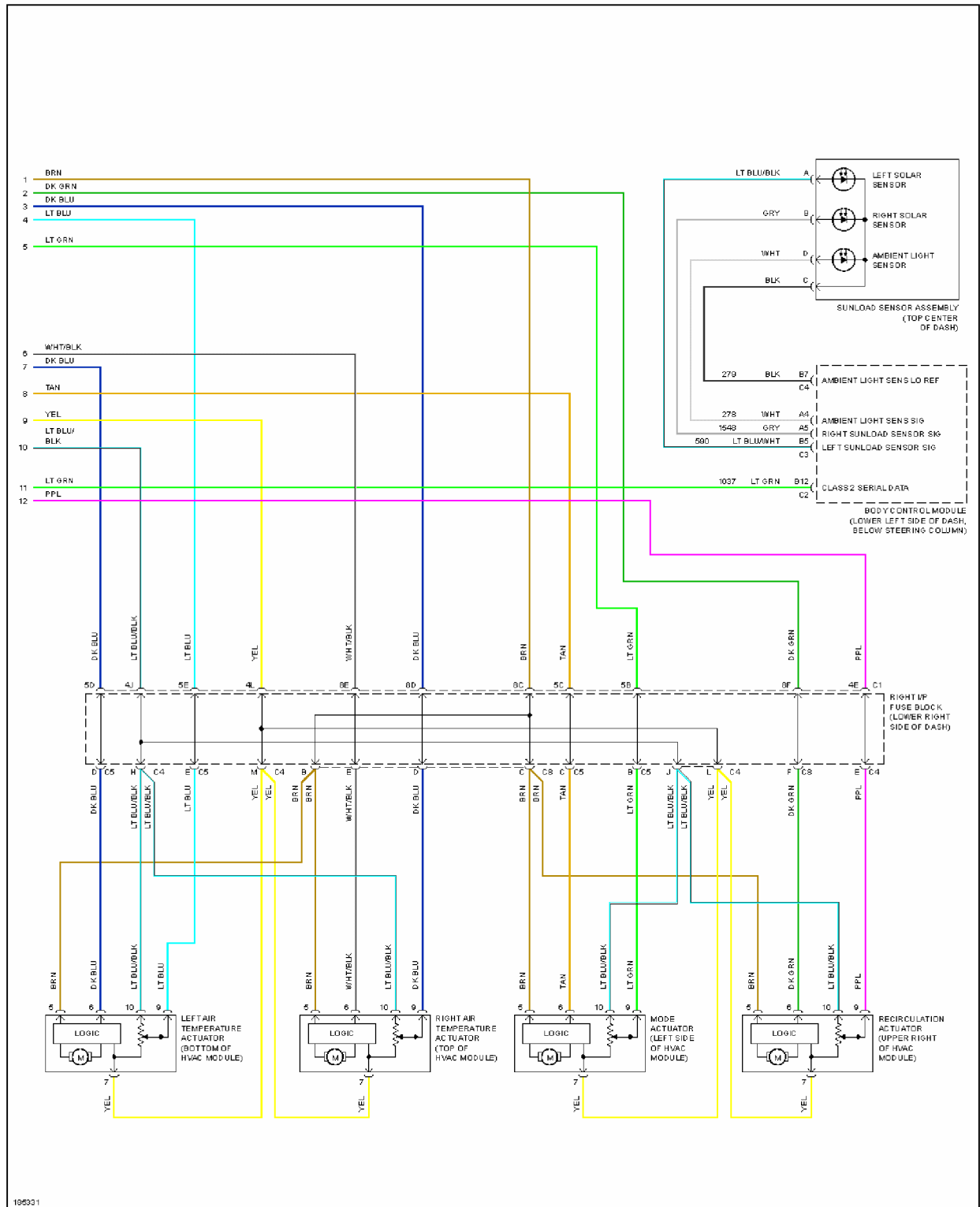
Fig. 2: Automatic A/C Circuit, Front A/C (2 of 2)
