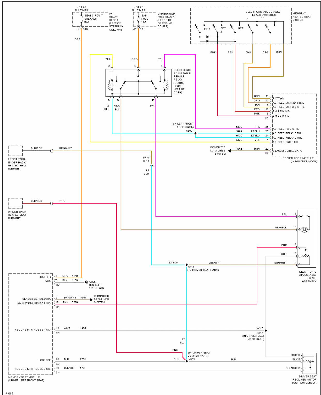
Fig. 47: Adjustable Pedal Circuit
