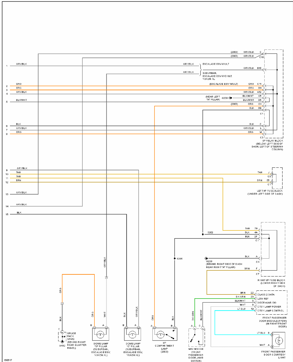
Fig. 43: Courtesy Lamps Circuit (3 of 3)
