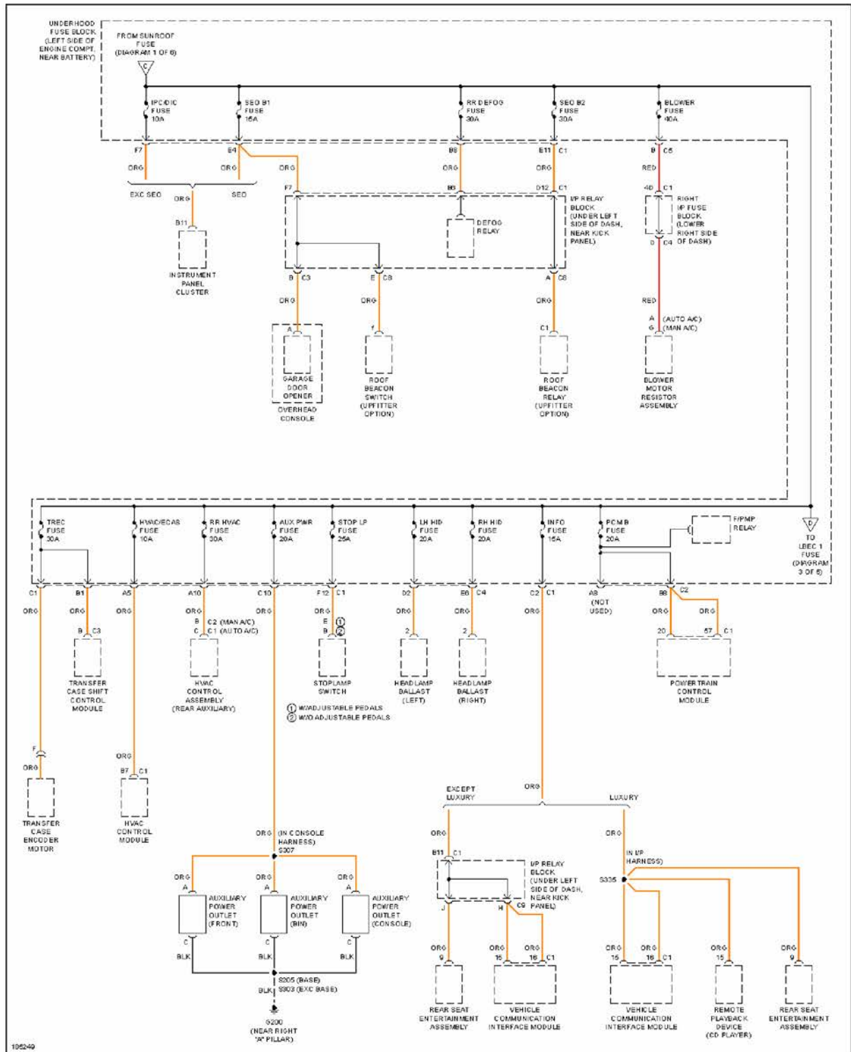
Fig. 53: Power Distribution Circuit (2 of 6)
