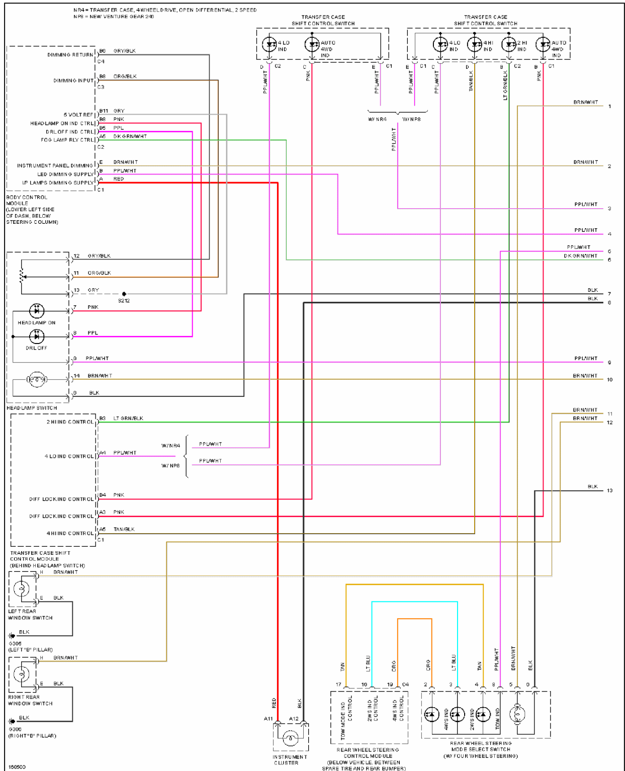
Fig. 44: Instrument Illumination Circuit (1 of 3)
