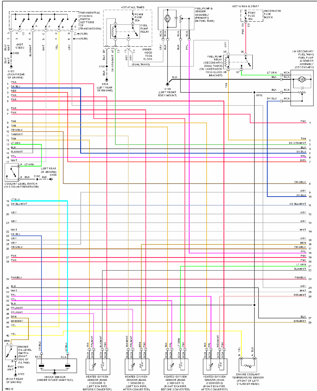
Fig. 19: 5.3L VIN T, Engine Performance Circuit (2 of 5)
