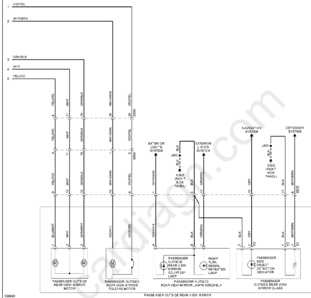
Fig. 100: Power Mirrors Circuit (2 of 2)
