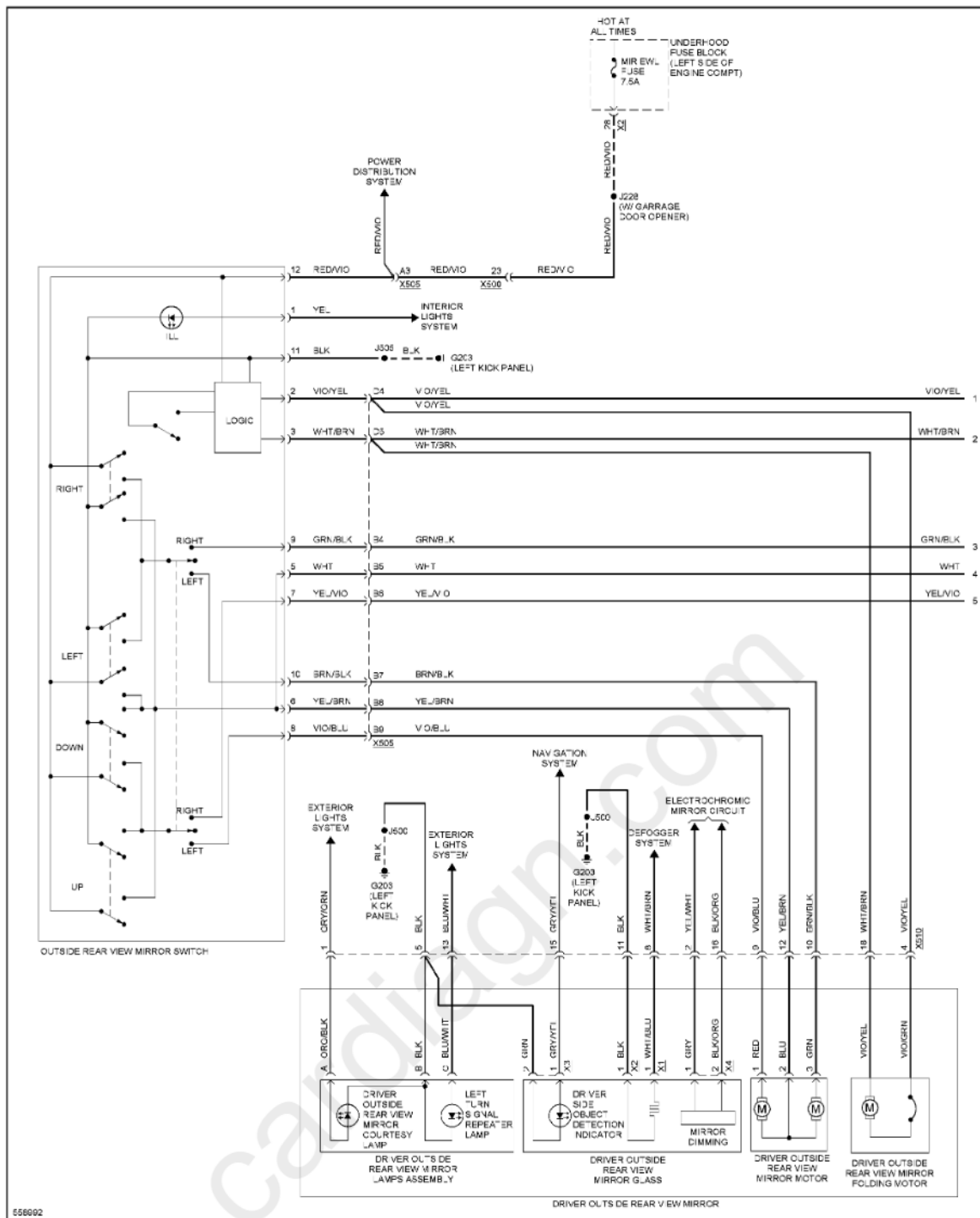
Fig. 99: Power Mirrors Circuit (1 of 2)
