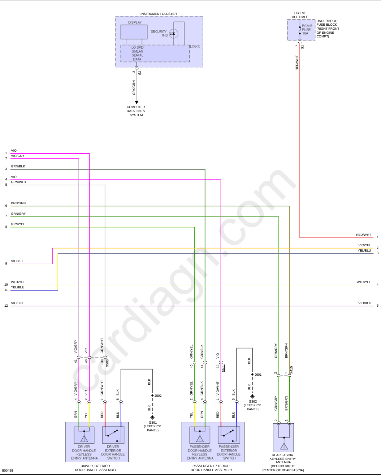
Fig 2: Power Door Locks Circuit (2 of 4)
