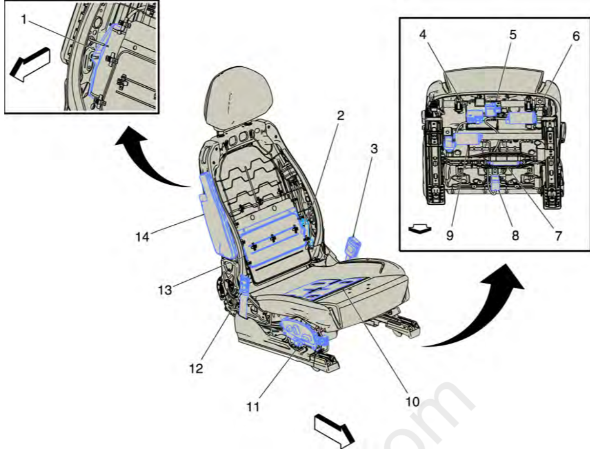
Fig. 6: Passenger Seat Components
