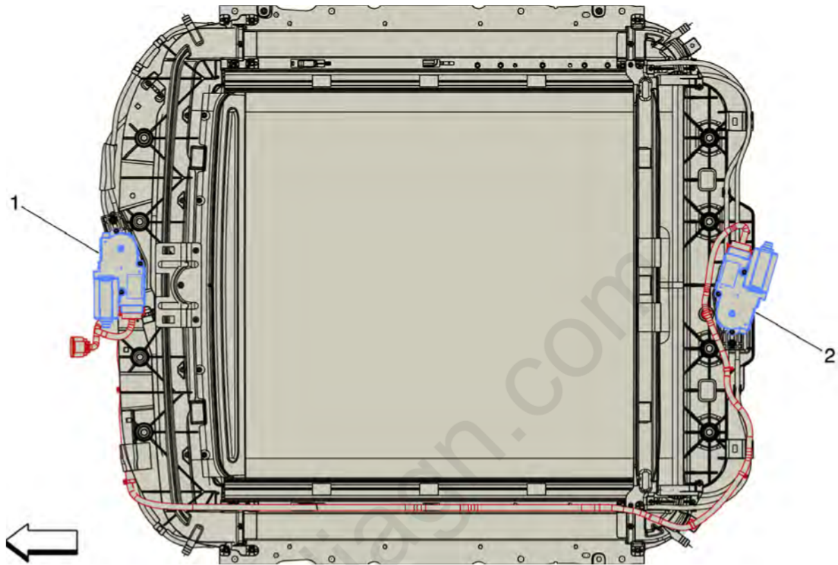
Fig. 2: Sunroof Components (C3U)
