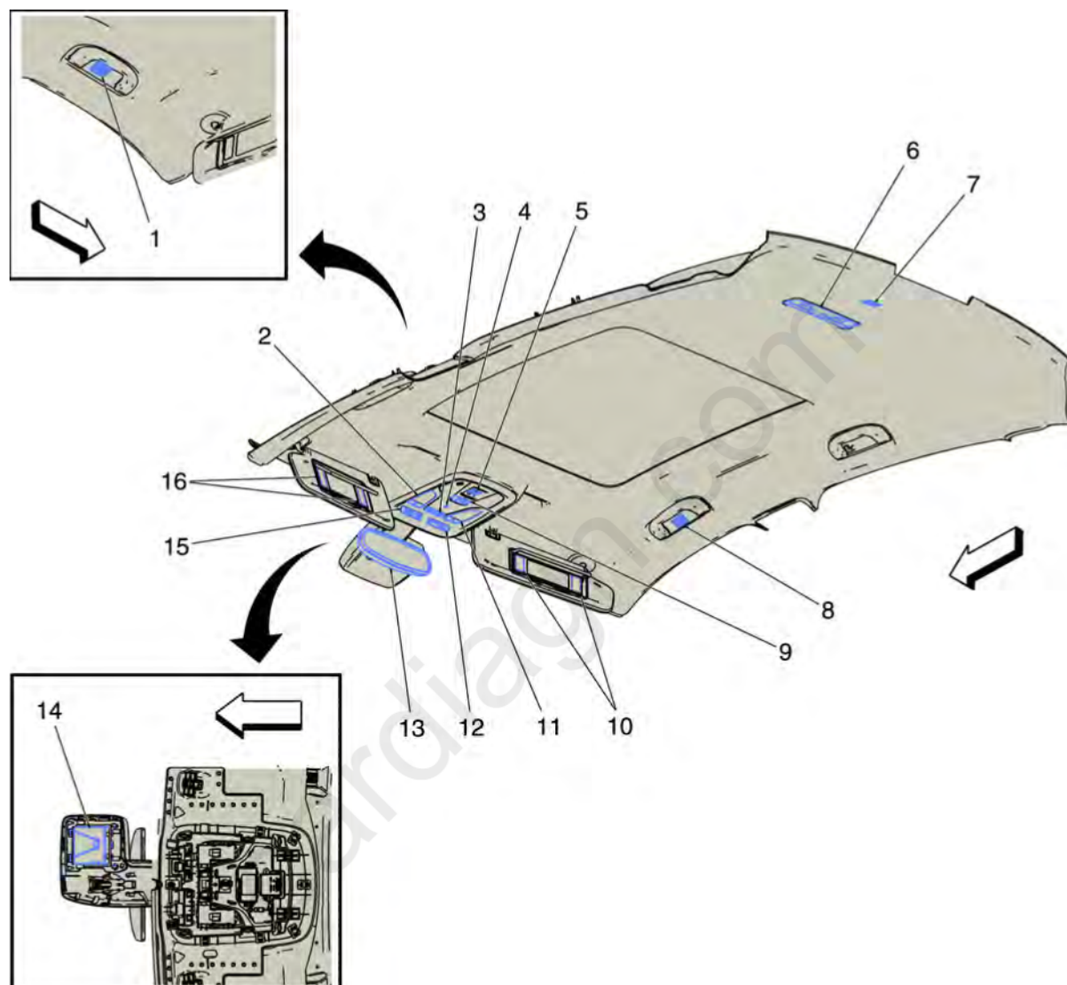
Fig. 1: Headliner Components
