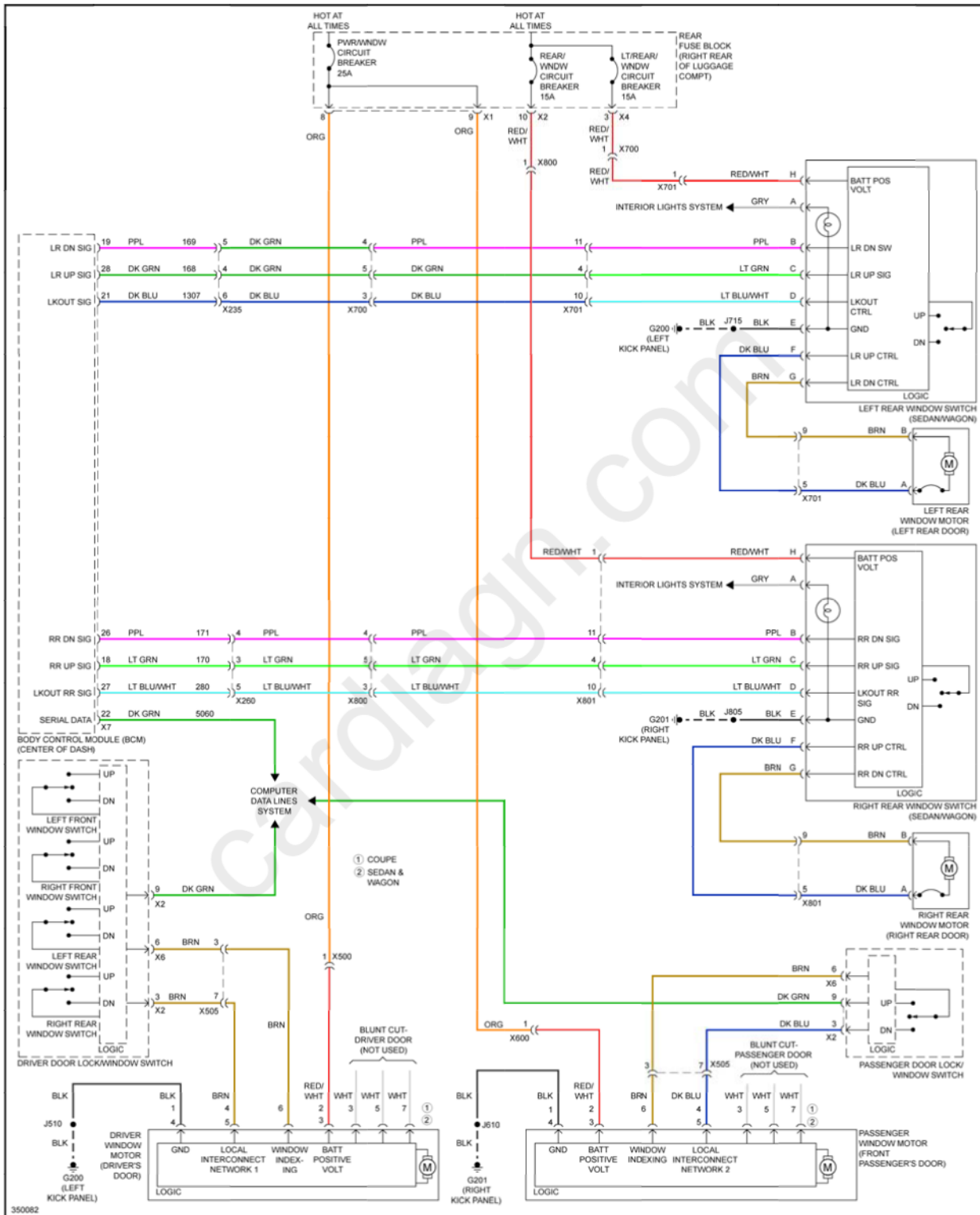
Fig. 98: Power Windows Circuit
