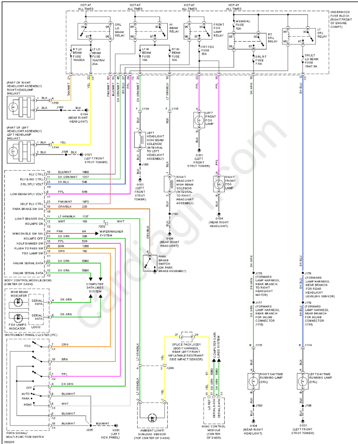
Fig. 51: Headlamps Circuit, W/ High Intensity Discharge
