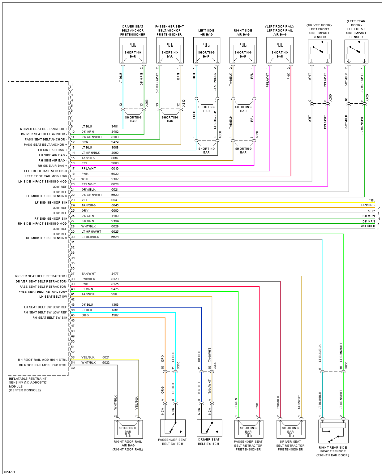
Fig. 73: Supplemental Restraints Circuit (1 of 2)
