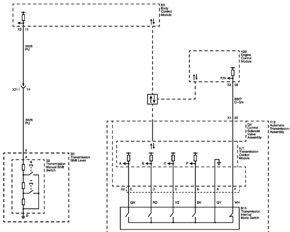
Fig. 3: IMS and Tap Up/Tap Down (MH2 or MH4) Courtesy of GENERAL MOTORS CORP.
