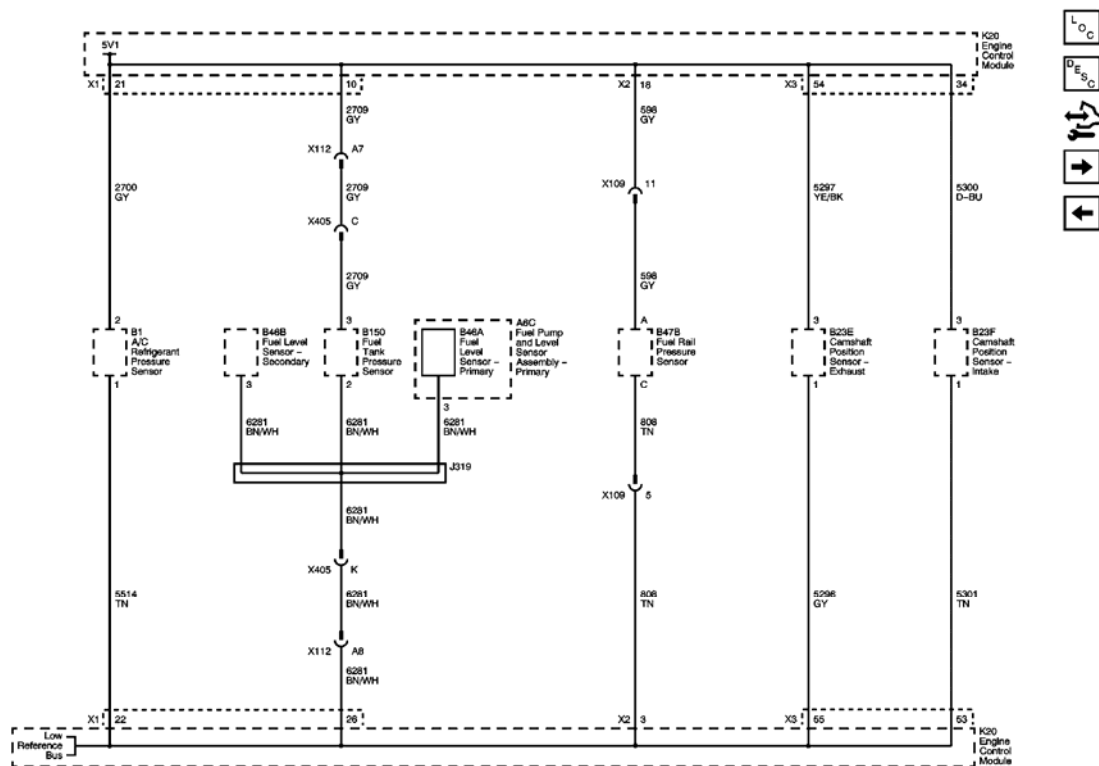
Fig. 2: 5V1 and Low Reference Bus (LAF) Courtesy of GENERAL MOTORS CORP.
