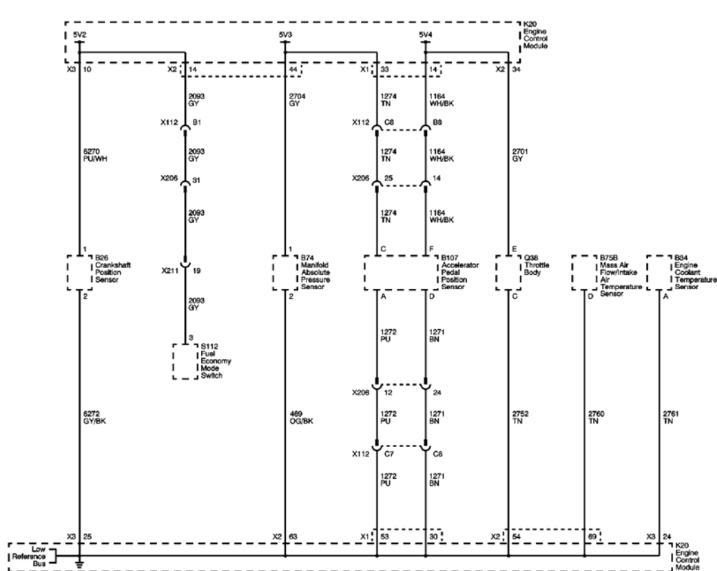
Fig. 3: 5V2, 5V3, 5V4, and Low Reference Bus (LAF) Courtesy of GENERAL MOTORS CORP.
