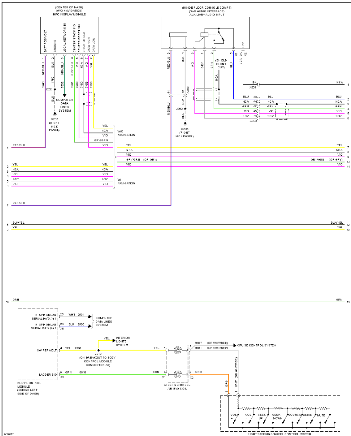
Fig. 119: Radio Circuit, W/O Amplifier (3 of 4)
