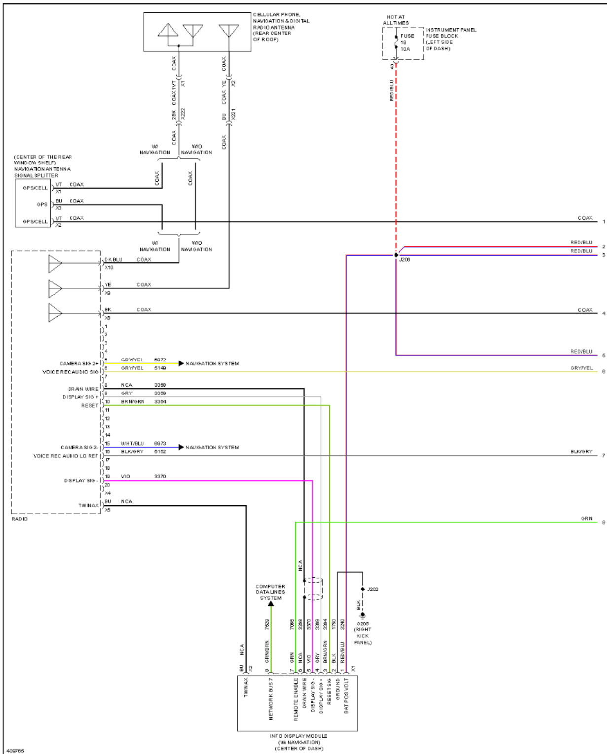
Fig. 117: Radio Circuit, W/O Amplifier (1 of 4)
