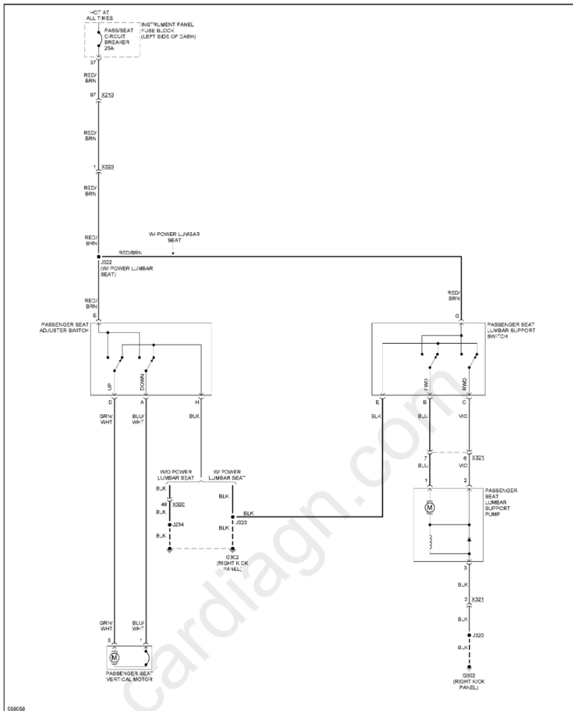
Fig. 106: Passenger Power Seat Circuit, 2-Way Power Seat
