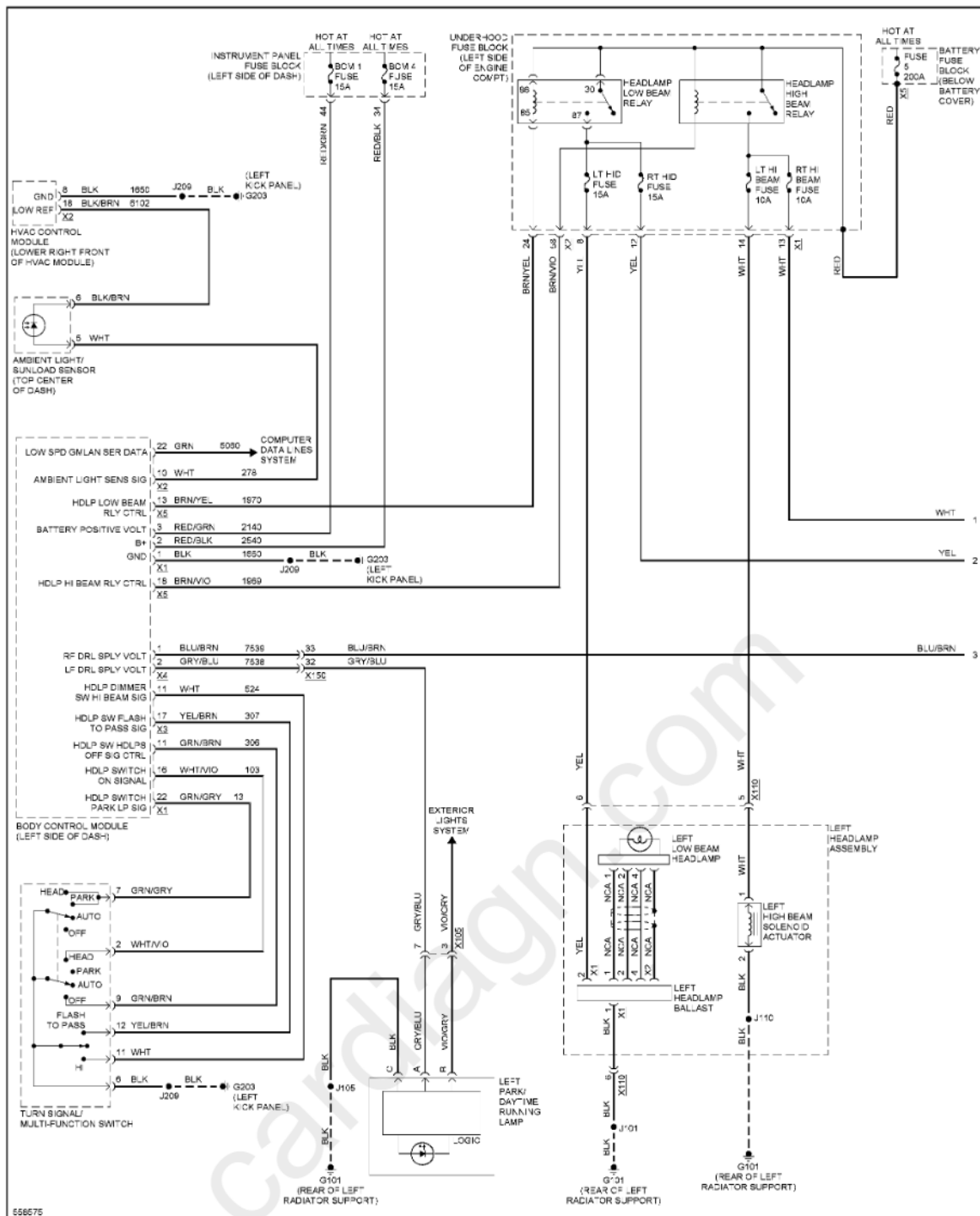
Fig. 58: Headlights Circuit, W/ High Intensity Discharge (1 of 2)
