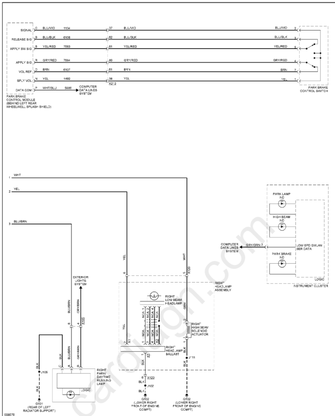
Fig. 59: Headlights Circuit, W/ High Intensity Discharge (2 of 2)
