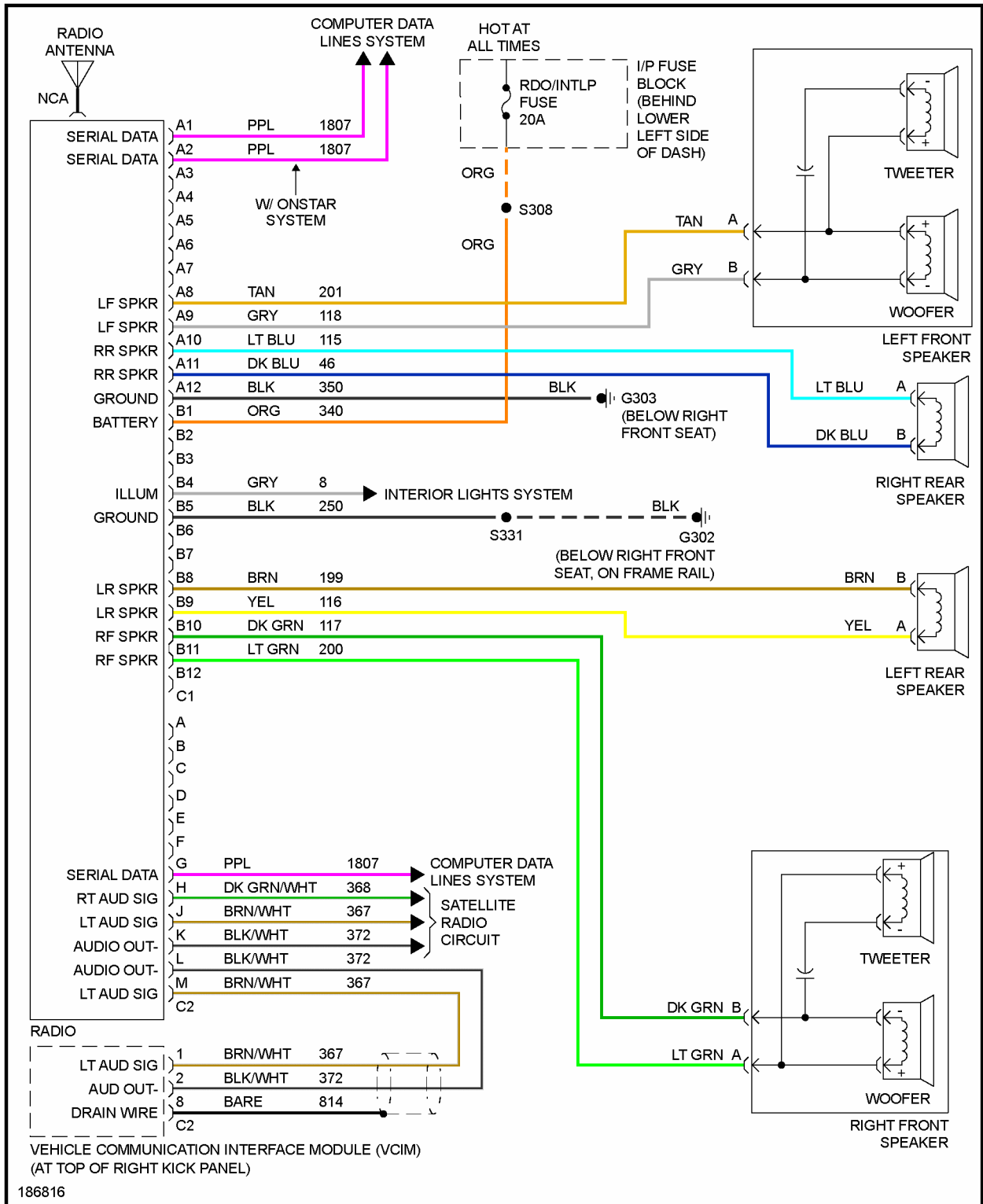
Fig. 30: Radio Circuit, Base
