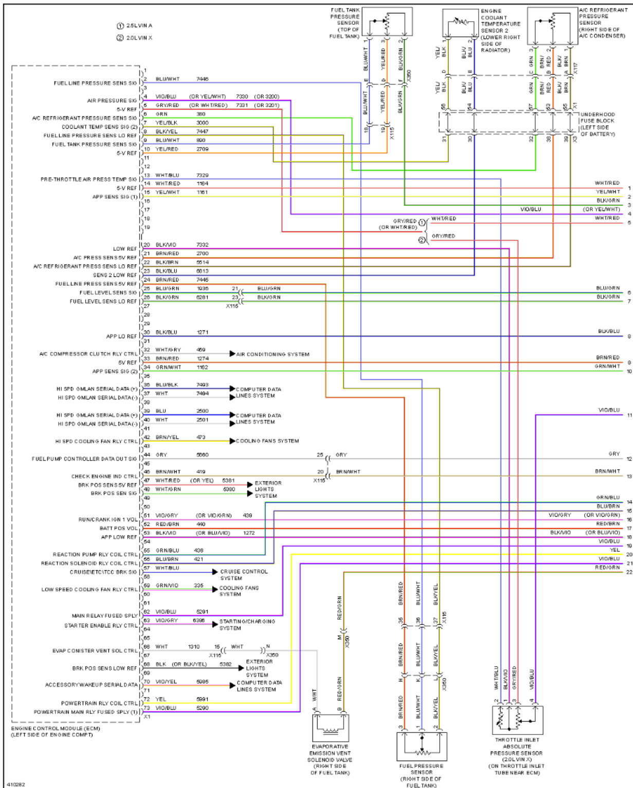
Fig. 45: 2.5L VIN A, Engine Performance Circuit (1 of 6)
