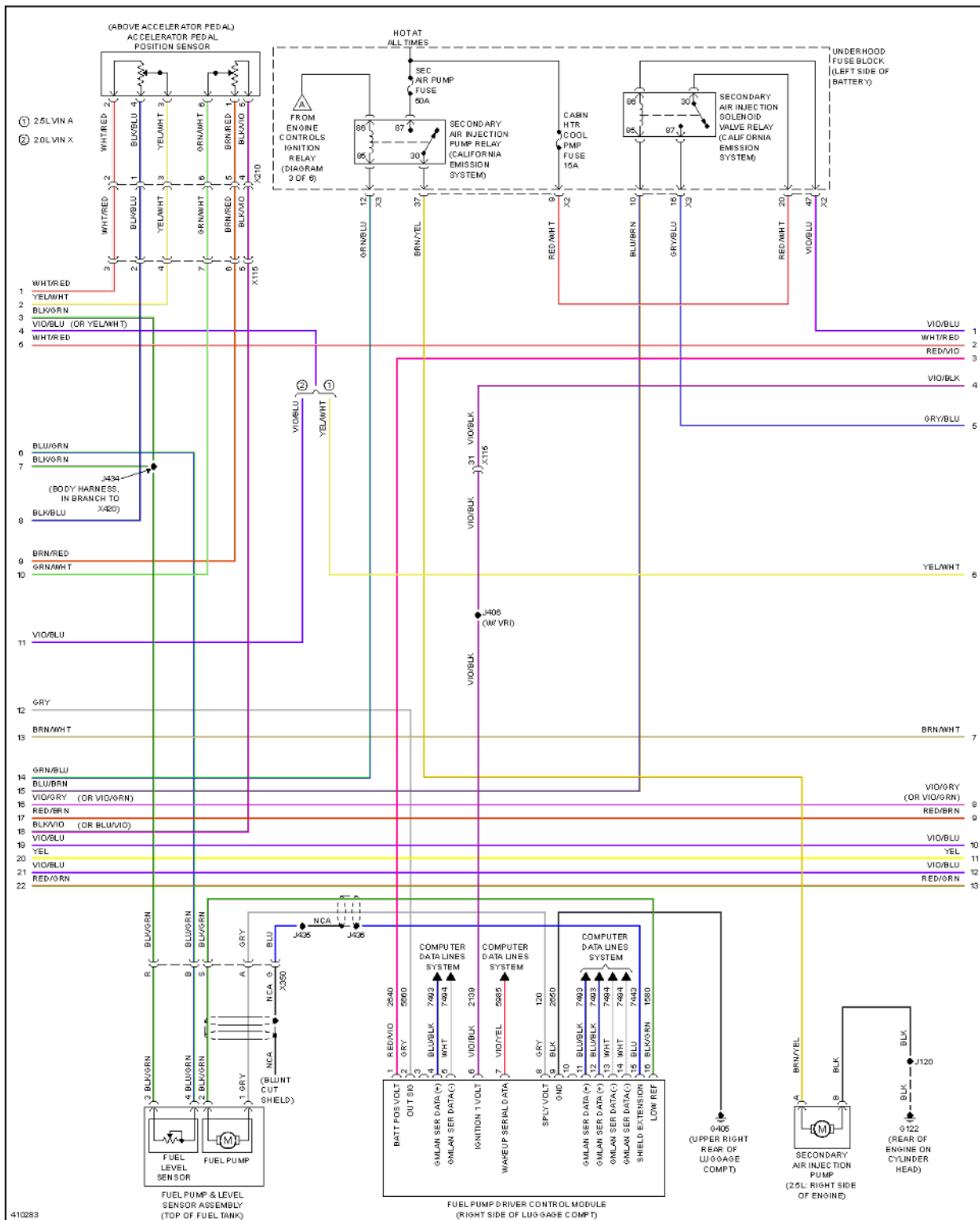
Fig. 46: 2.5L VIN A, Engine Performance Circuit (2 of 6)
