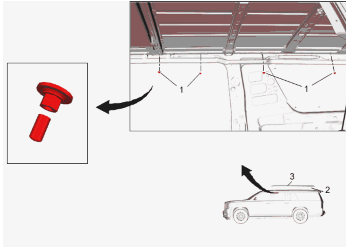
Fig. 2: Luggage Carrier Side Rail (Long Wheelbase, Built Prior to 9/1/2014)
