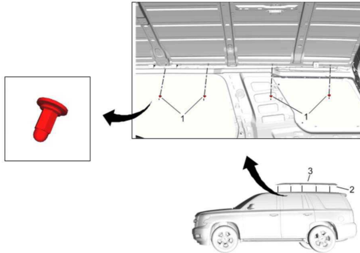
Fig. 3: Luggage Carrier Side Rail (Short Wheelbase, Built After 9/2/2014)
