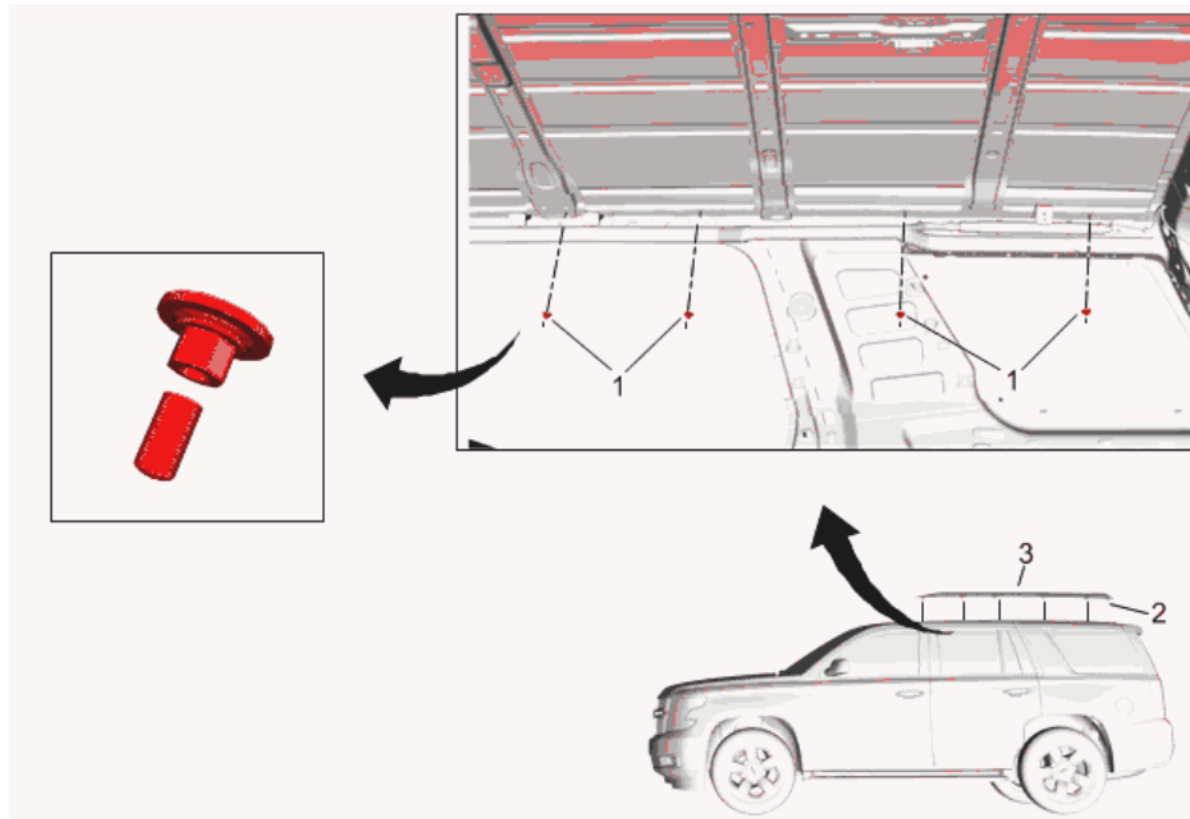
Fig. 1: Luggage Carrier Side Rail (Short Wheelbase, Built Prior to 9/1/2014)
