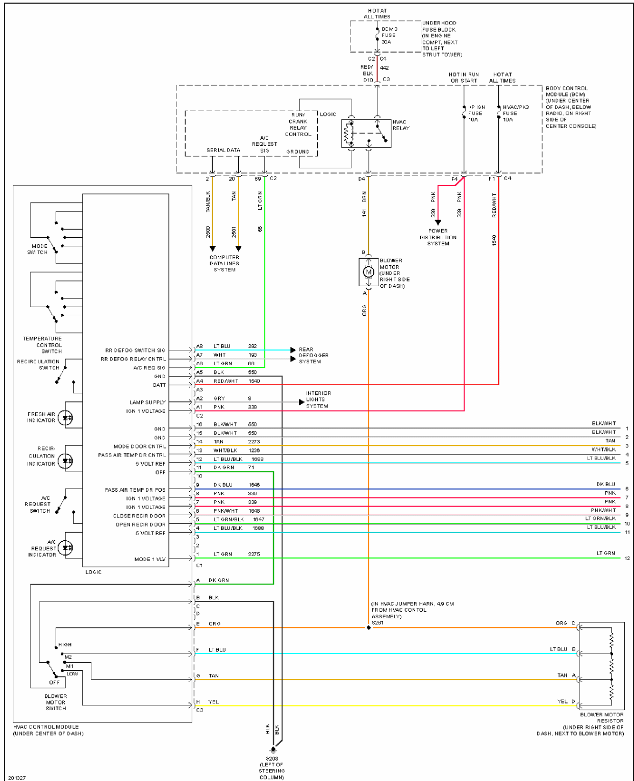
Fig. 5: 2.2L VIN F, Manual A/C Circuit (1 of 2)
