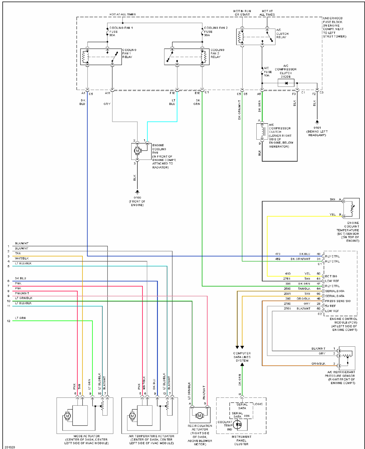
Fig. 6: 2.2L VIN F, Manual A/C Circuit (2 of 2)
