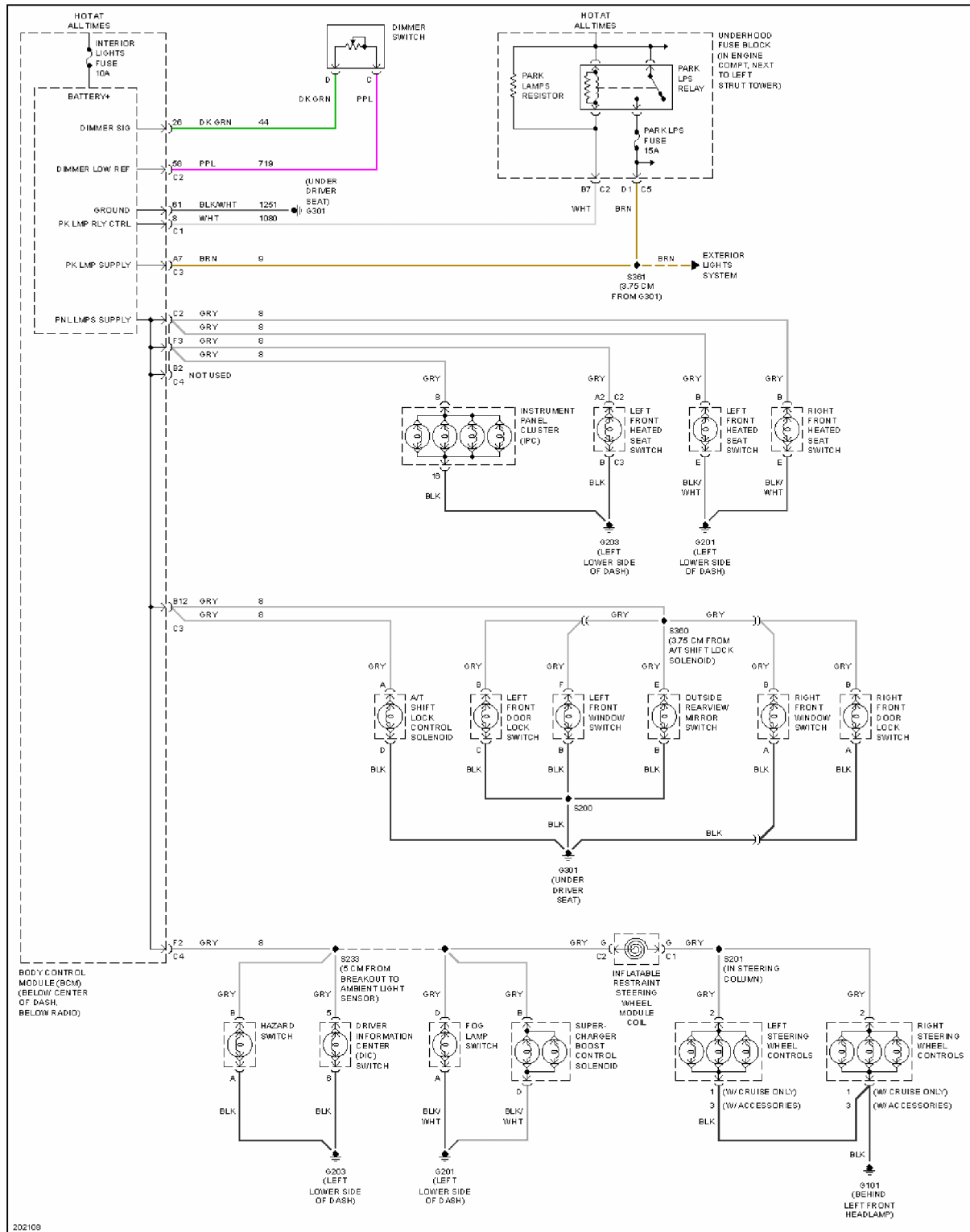
Fig. 39: Instrument Illumination Circuit
