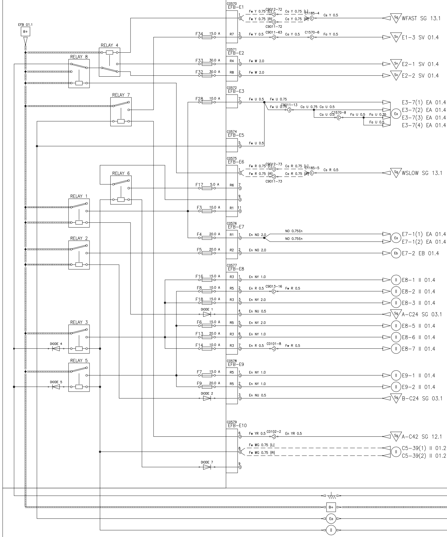
EFB (Engine Bay Fusebox) – Relays 1–8
