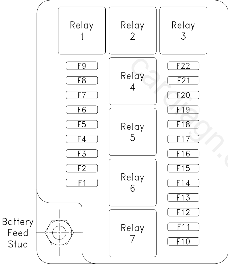
BOOT FUSEBOX AD43-14A073-AA
