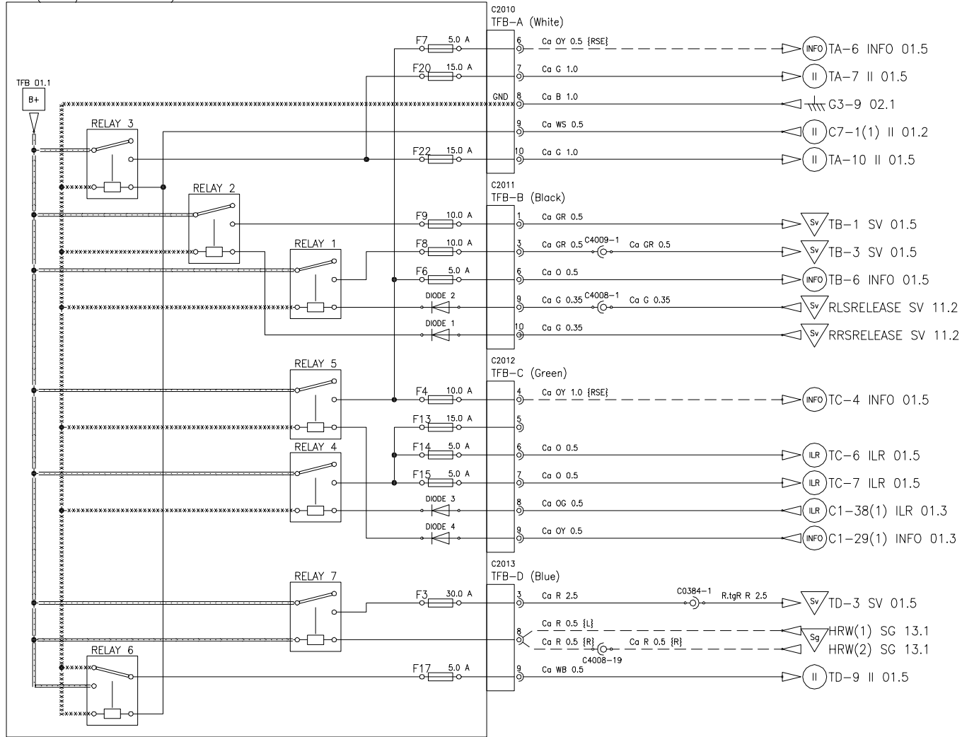
TFB (Trunk/Boot Fusebox)
