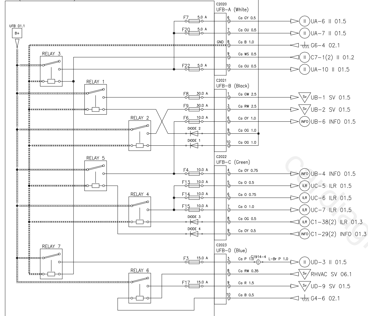
UFB (Underseat Fusebox)
