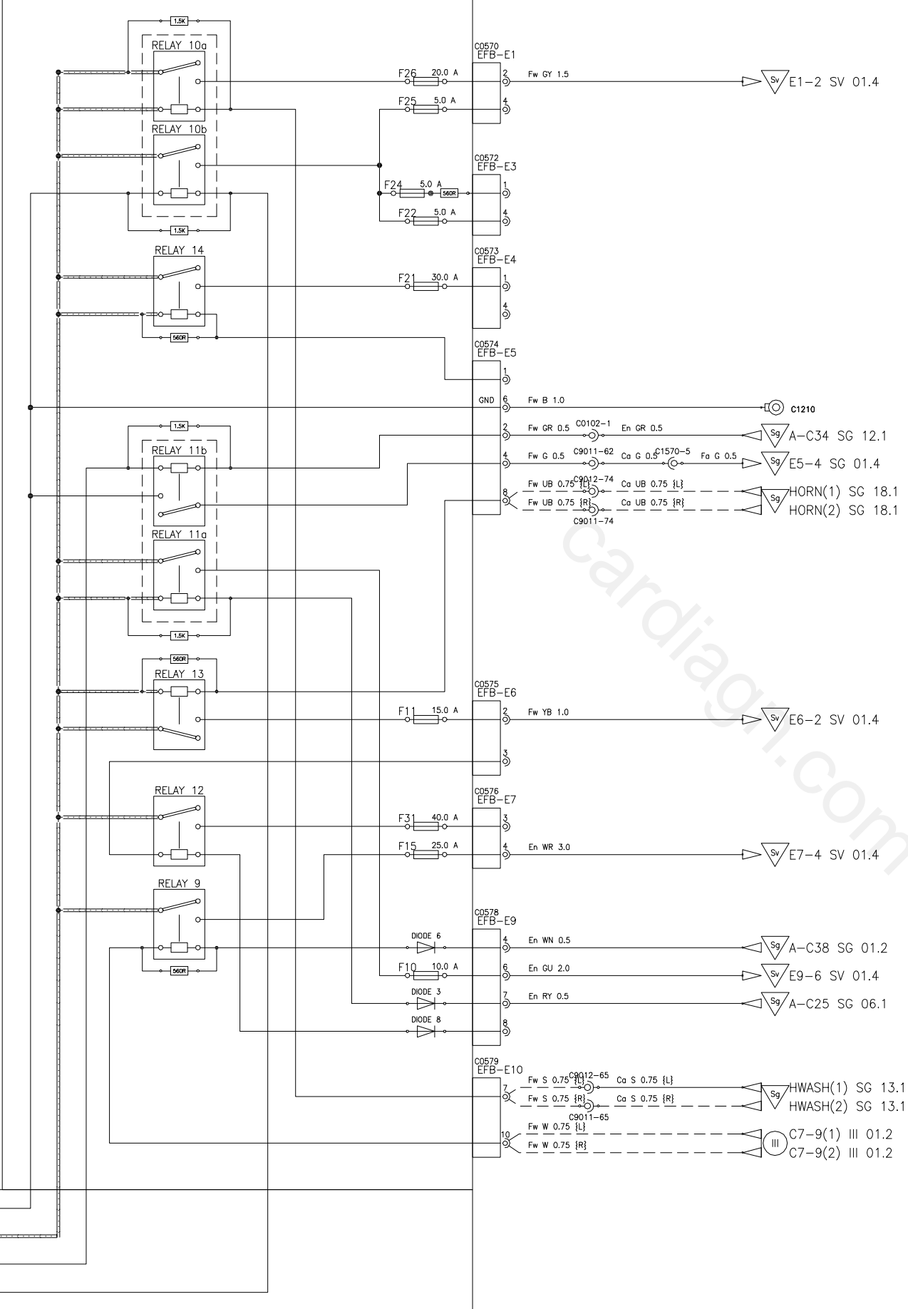
EFB (Engine Bay Fusebox) – Relays 9–14
