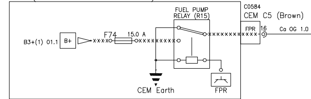
CEM (Central Electronic Module)
