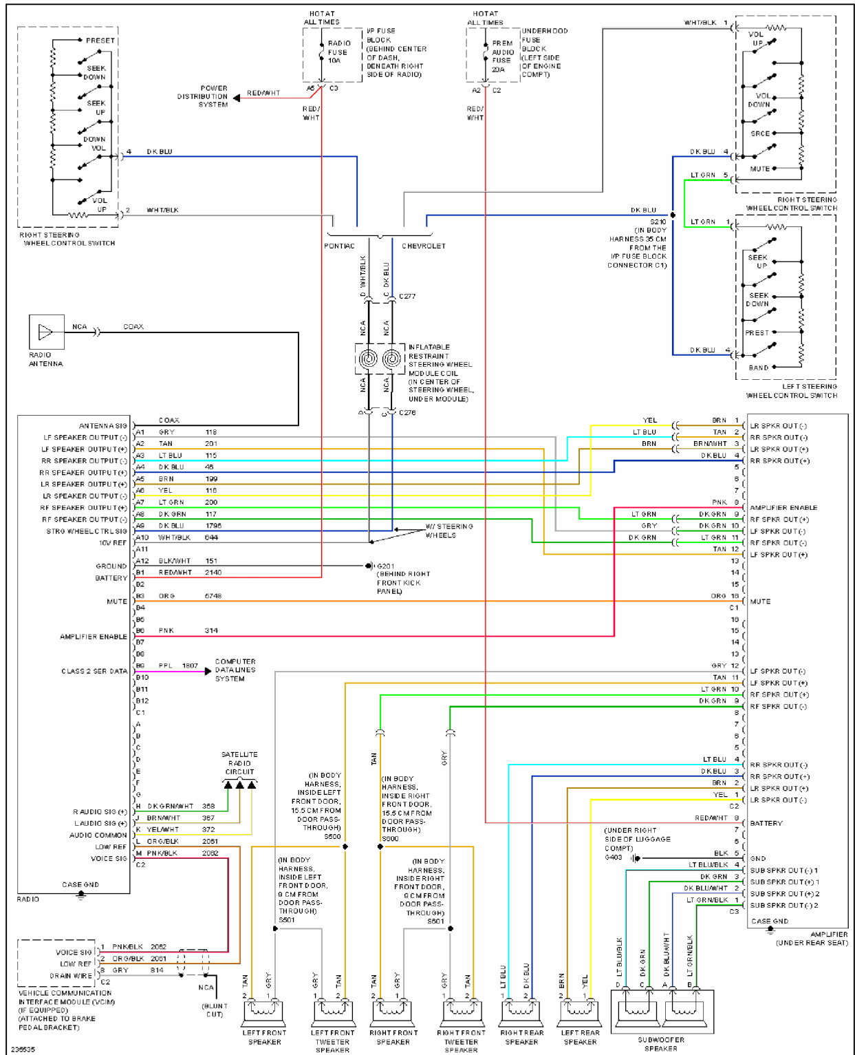
Fig. 39: Premium Sound Radio Circuit
