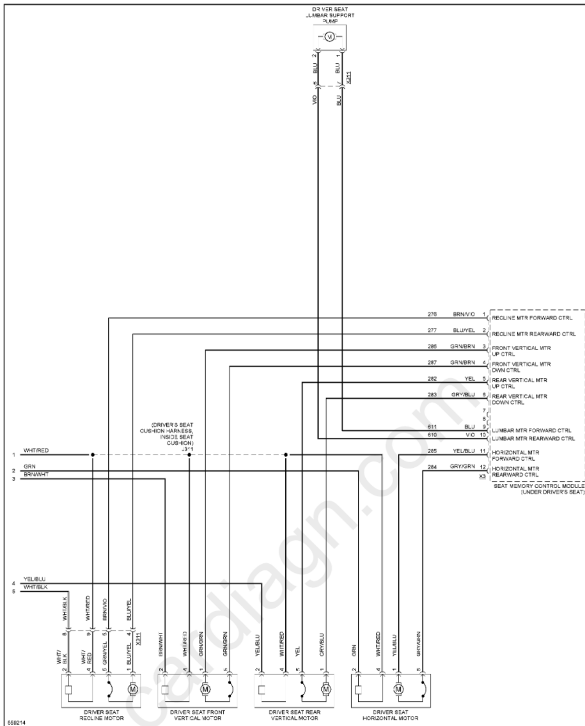
Fig. 71: Driver's Memory Seat Circuit (2 of 2)
