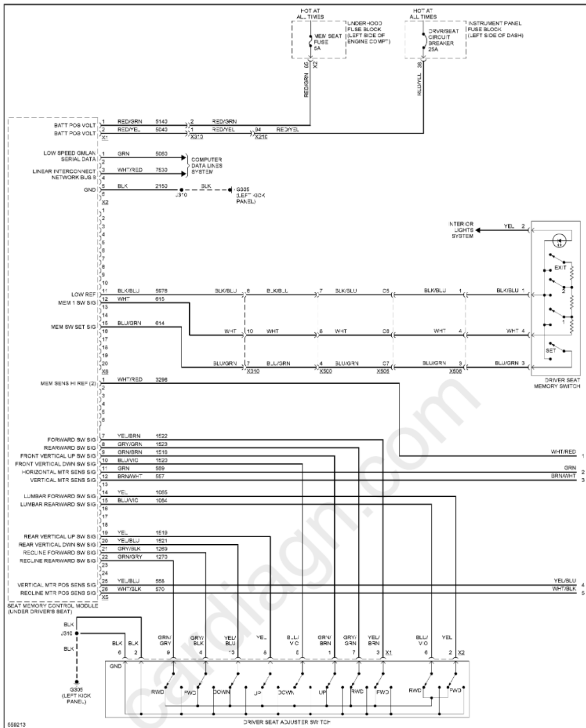
Fig. 70: Driver's Memory Seat Circuit (1 of 2)
