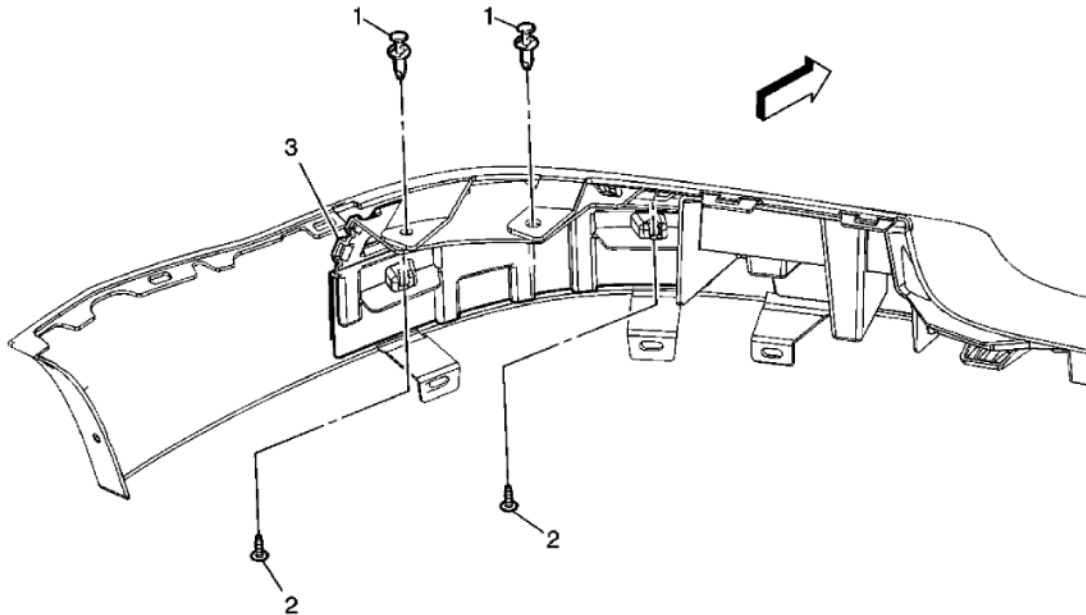
Fig. 16: View Of Front Bumper Fascia Outer Support (GMC) Courtesy of GENERAL MOTORS CORP.
