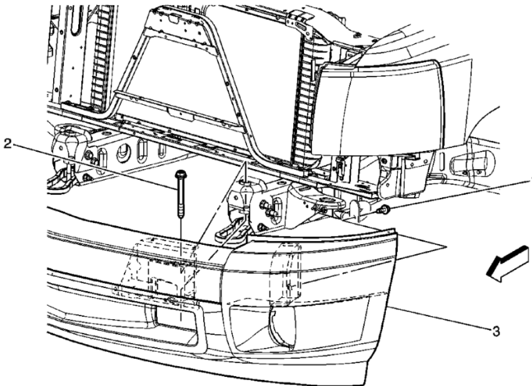
Fig. 2: View Of Front Bumper Impact Bar (Chevrolet) Courtesy of GENERAL MOTORS CORP.
