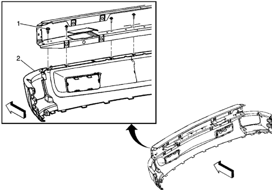
Fig. 18: View Of Front Air Deflector (Chevrolet)
