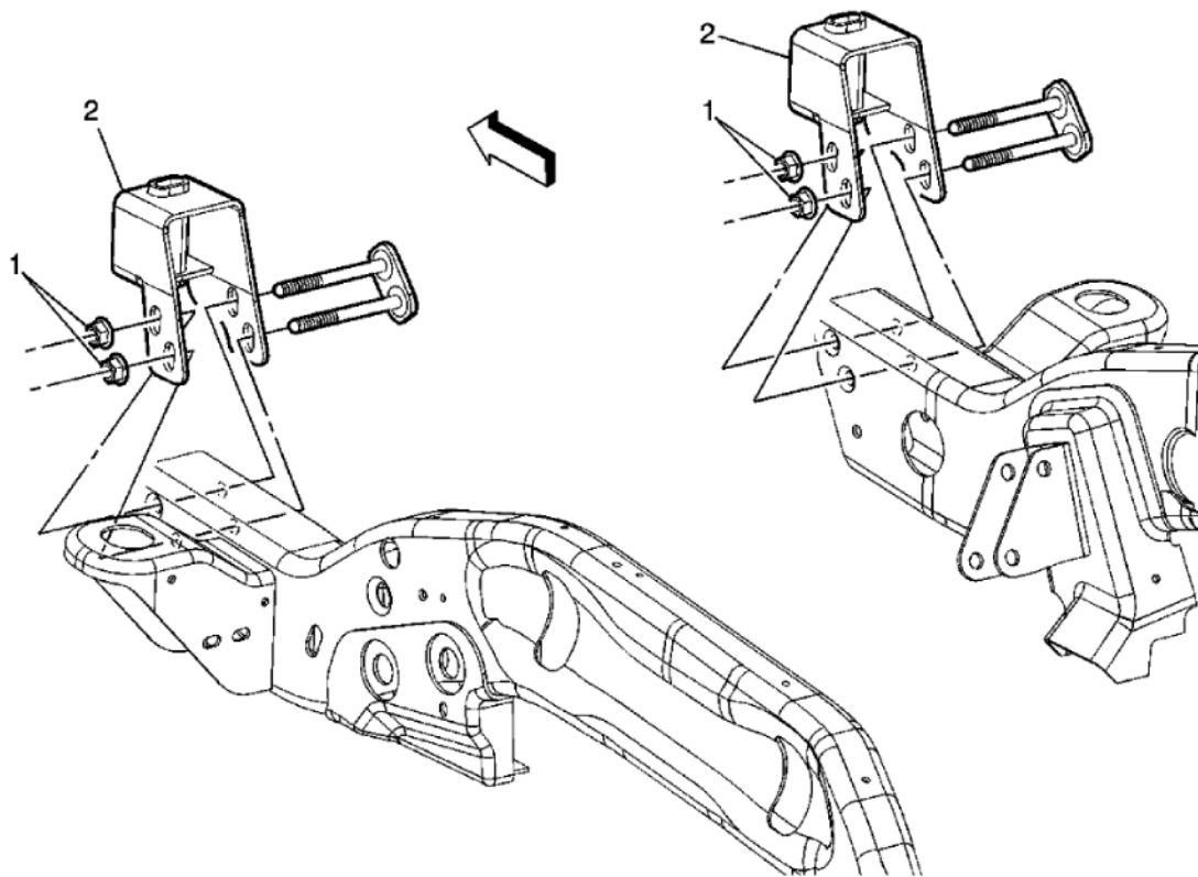
Fig. 9: View Of Front Bumper Impact Bar Extension Courtesy of GENERAL MOTORS CORP.
