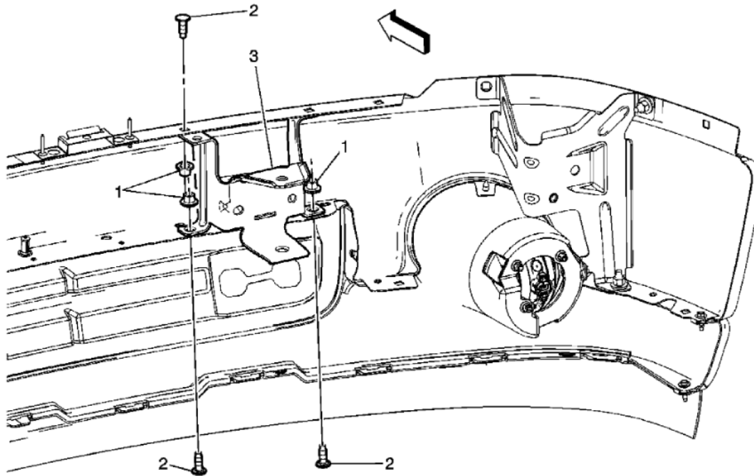
Fig. 4: View Of Front Bumper Impact Bar Inner Bracket (GMC) Courtesy of GENERAL MOTORS CORP.
