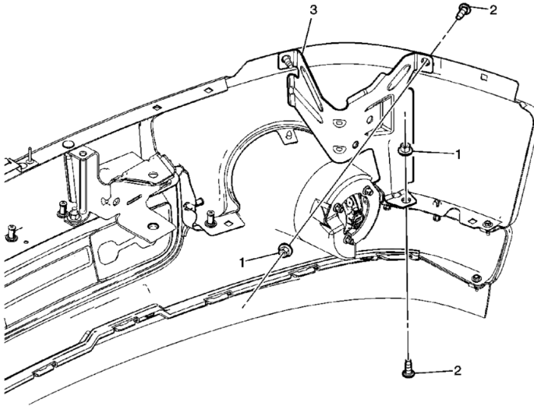
Fig. 6: View Of Front Bumper Impact Bar Outer Bracket (GMC)
