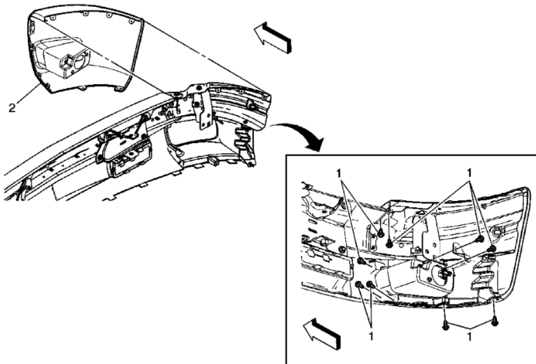
Fig. 10: View Of Front Bumper End Cap (Chevrolet) Courtesy of GENERAL MOTORS CORP.
