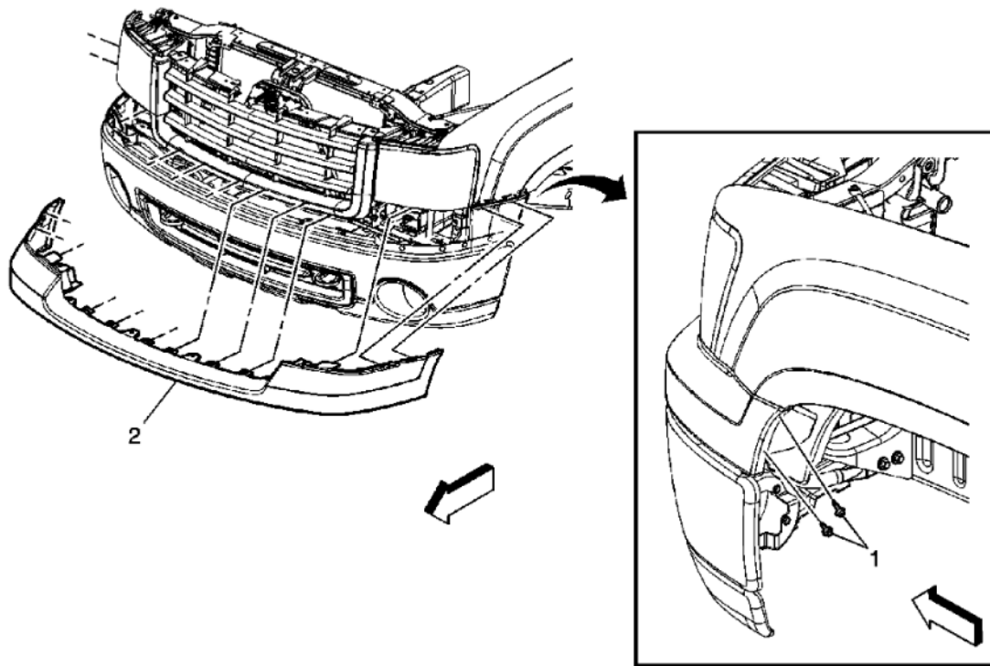
Fig. 13: View Of Front Bumper Fascia Trim Cap (GMC) Courtesy of GENERAL MOTORS CORP.
