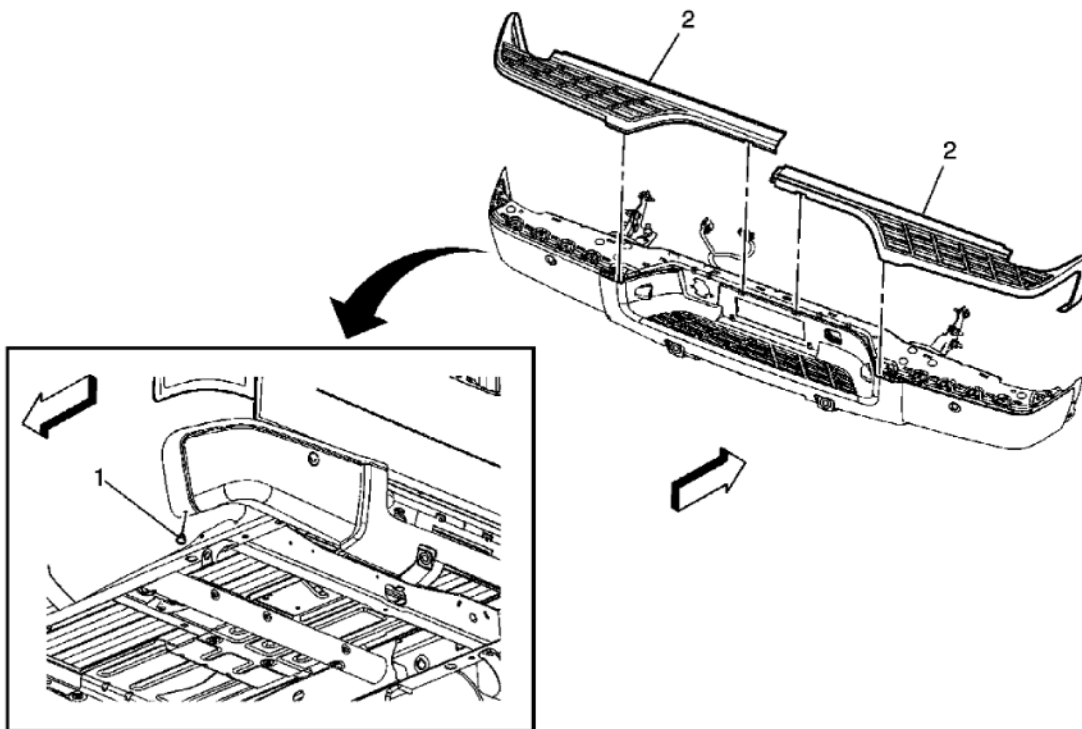
Fig. 24: View Of Rear Bumper Step Outer Pad Courtesy of GENERAL MOTORS CORP.
