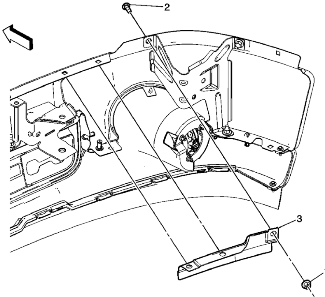
Fig. 7: View Of Front Bumper Impact Bar Outer Reinforcement (GMC) Courtesy of GENERAL MOTORS CORP.
