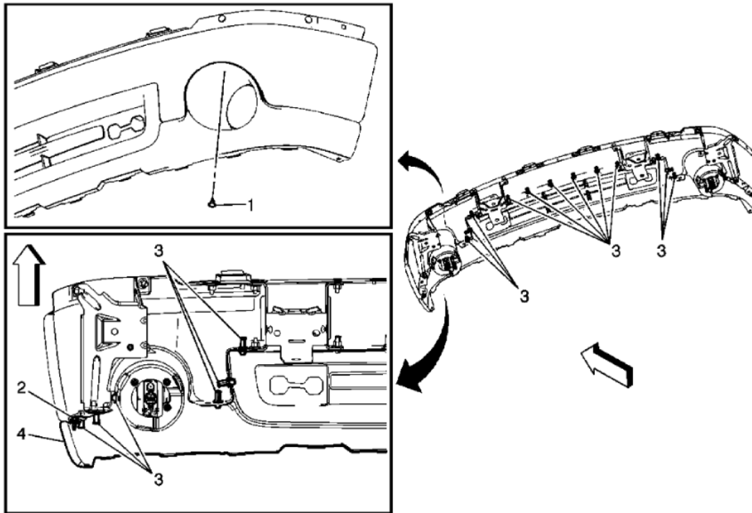
Fig. 17: View Of Front Air Deflector (GMC) Courtesy of GENERAL MOTORS CORP.
