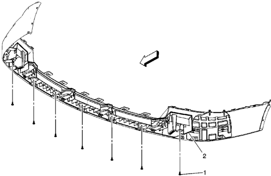
Fig. 14: View Of Front Bumper Fascia Center Support Bracket (GMC) Courtesy of GENERAL MOTORS CORP.
