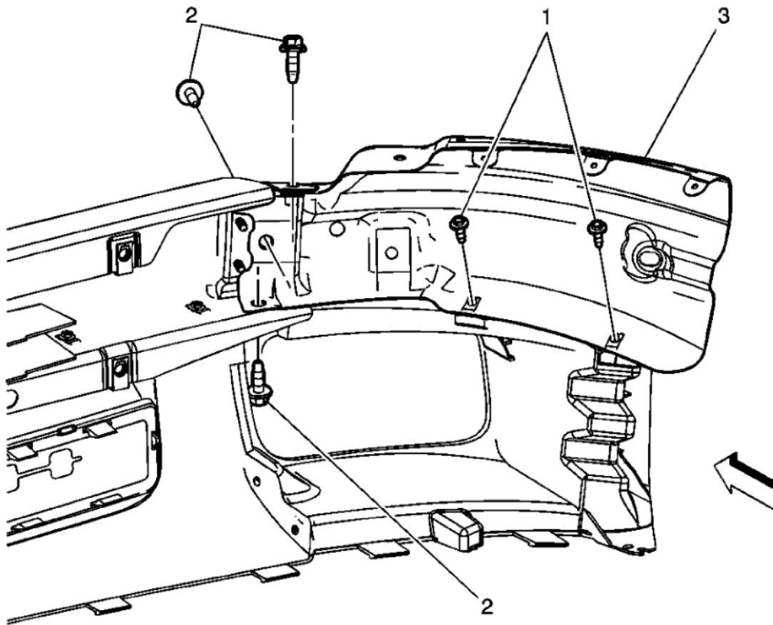
Fig. 8: View Of Front Bumper Impact Bar Extension (Chevrolet) Courtesy of GENERAL MOTORS CORP.
