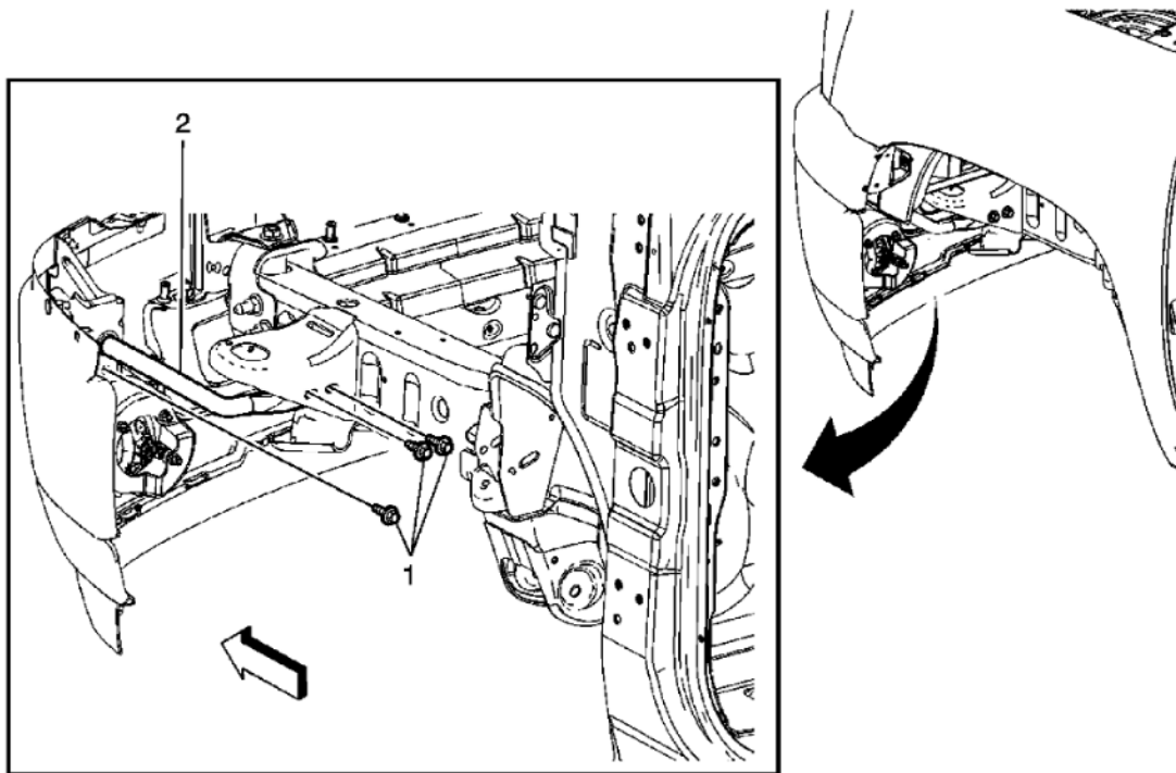
Fig. 12: View Of Front Bumper Impact Bar Brace Courtesy of GENERAL MOTORS CORP.
