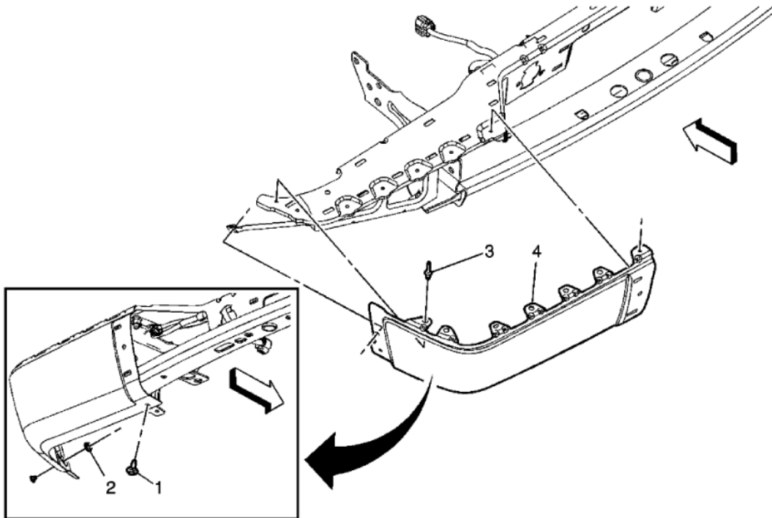
Fig. 21: View Of Rear Bumper Impact Bar End Cap
