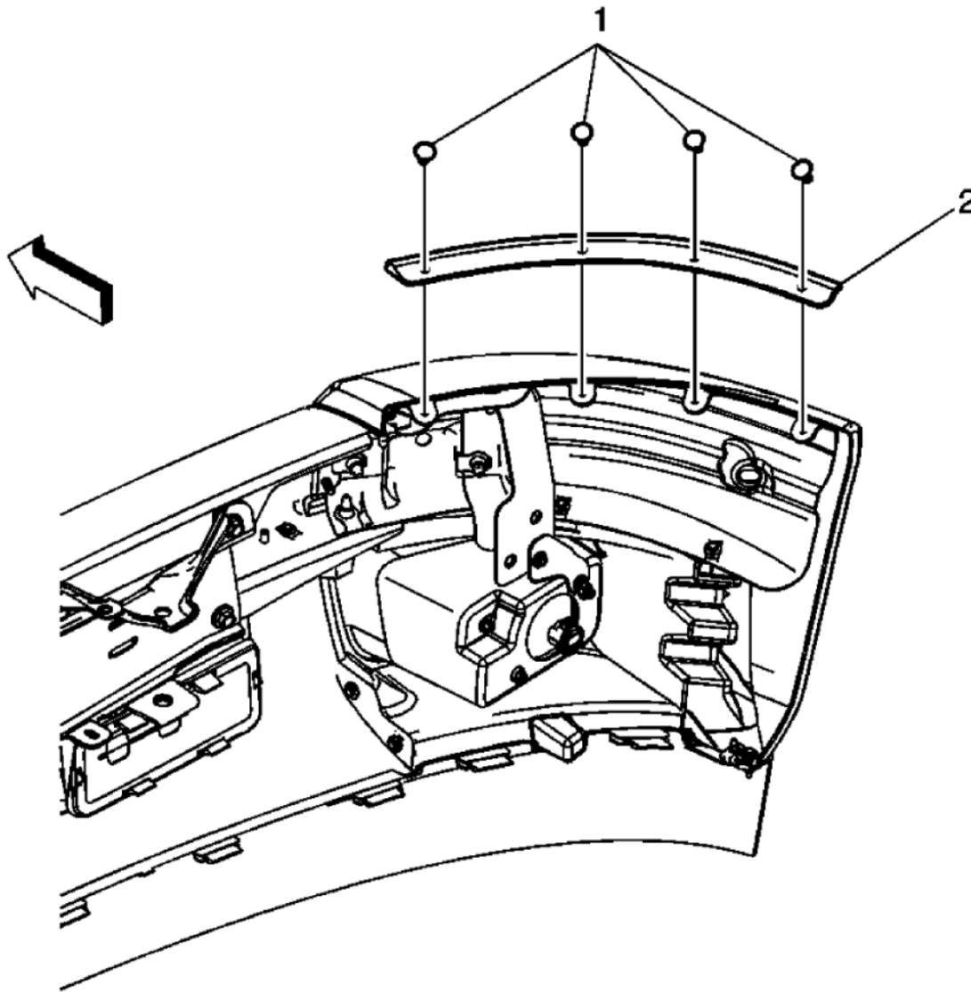
Fig. 11: View Of Front Bumper Filler (Chevrolet) Courtesy of GENERAL MOTORS CORP.
