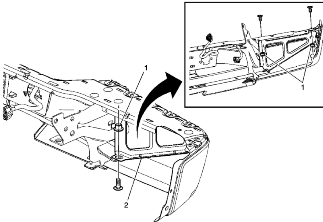
Fig. 22: View Of Rear Bumper Impact Bar Brace Courtesy of GENERAL MOTORS CORP.
