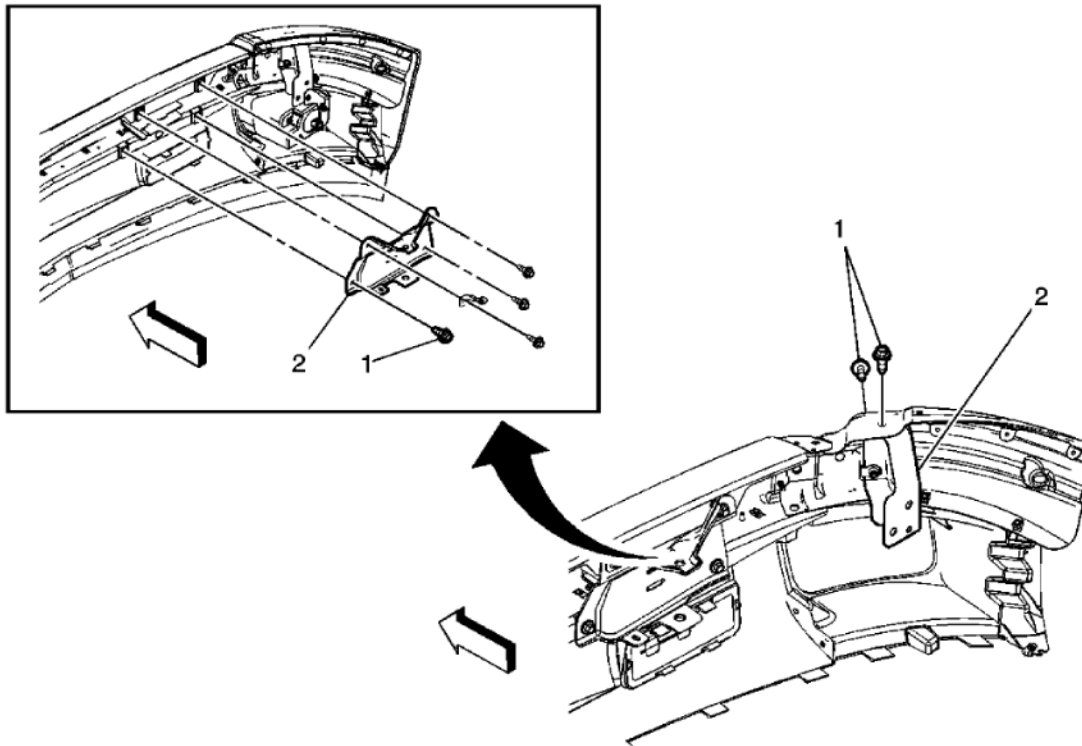
Fig. 5: View Of Front Bumper Impact Bar Outer Bracket (Chevrolet) Courtesy of GENERAL MOTORS CORP.
