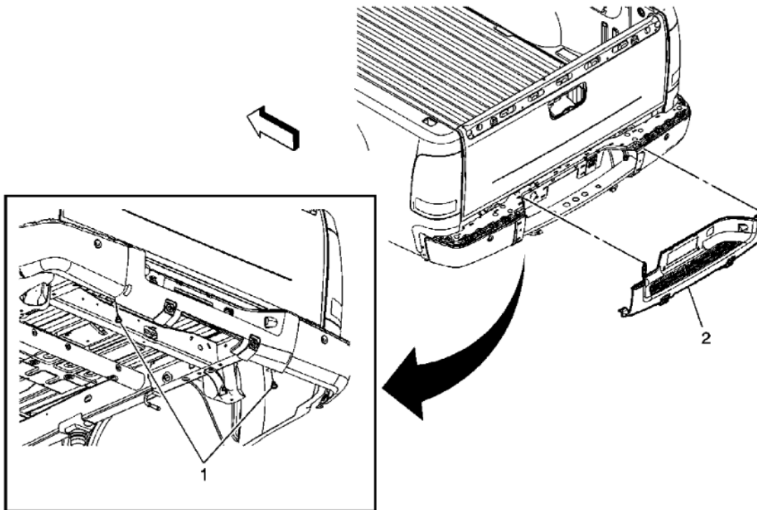
Fig. 23: View Of Rear Bumper Step Center Pad Courtesy of GENERAL MOTORS CORP.
