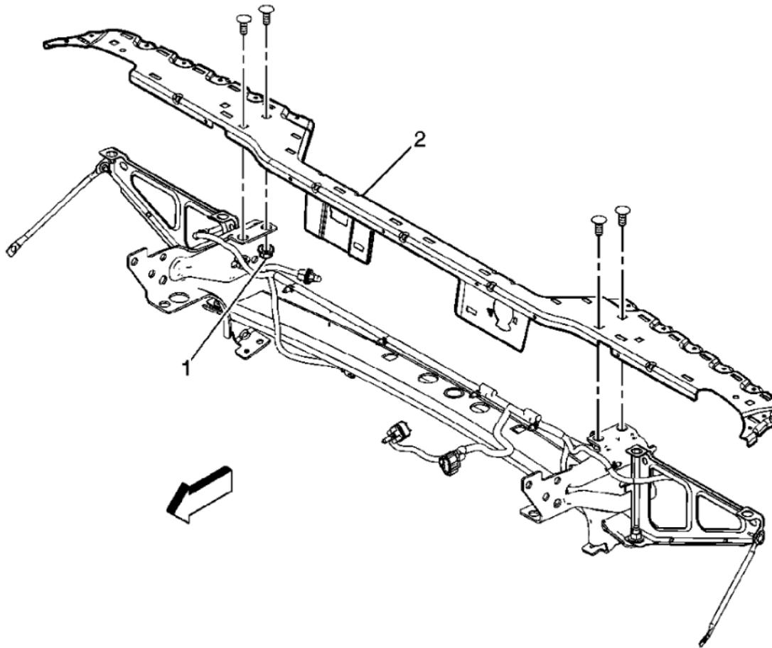
Fig. 20: View Of Rear Bumper Impact Bar Courtesy of GENERAL MOTORS CORP.
