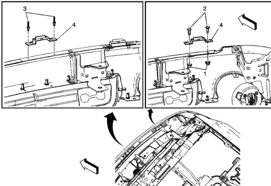
Fig. 3: View Of Front Bumper Impact Bar Bracket (GMC) Courtesy of GENERAL MOTORS CORP.
