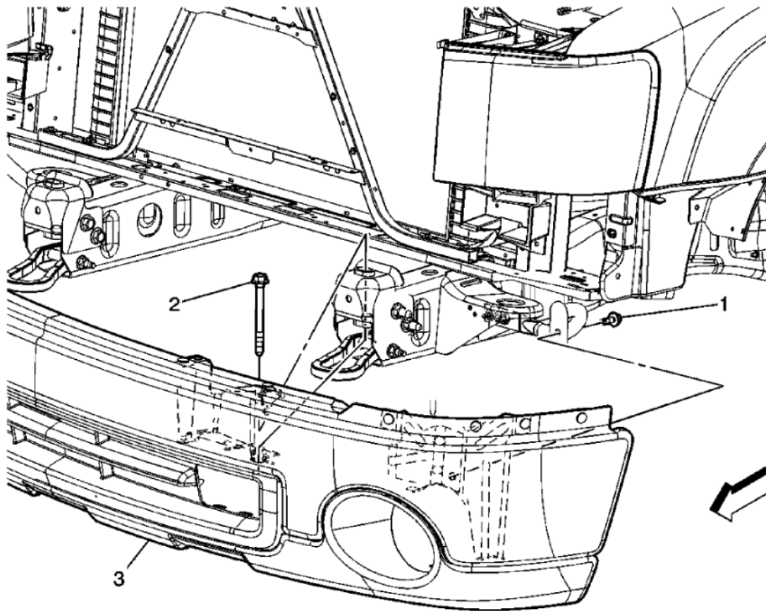
Fig. 1: View Of Front Bumper Impact Bar (GMC) Courtesy of GENERAL MOTORS CORP.
