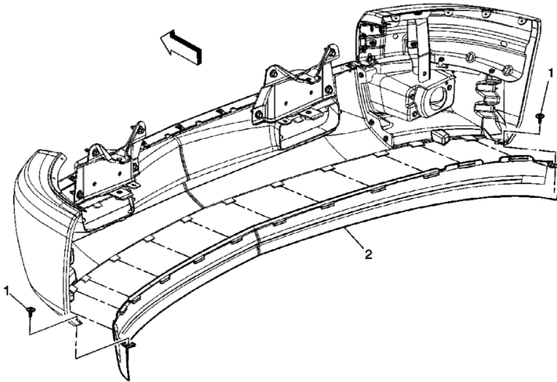
Fig. 19: View Of Front Air Deflector Extension
