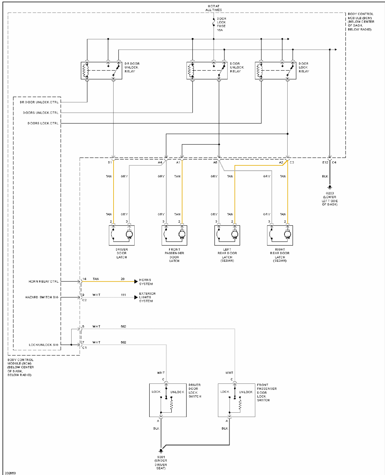
Fig. 44: Power Door Locks Circuit (2 of 2)
