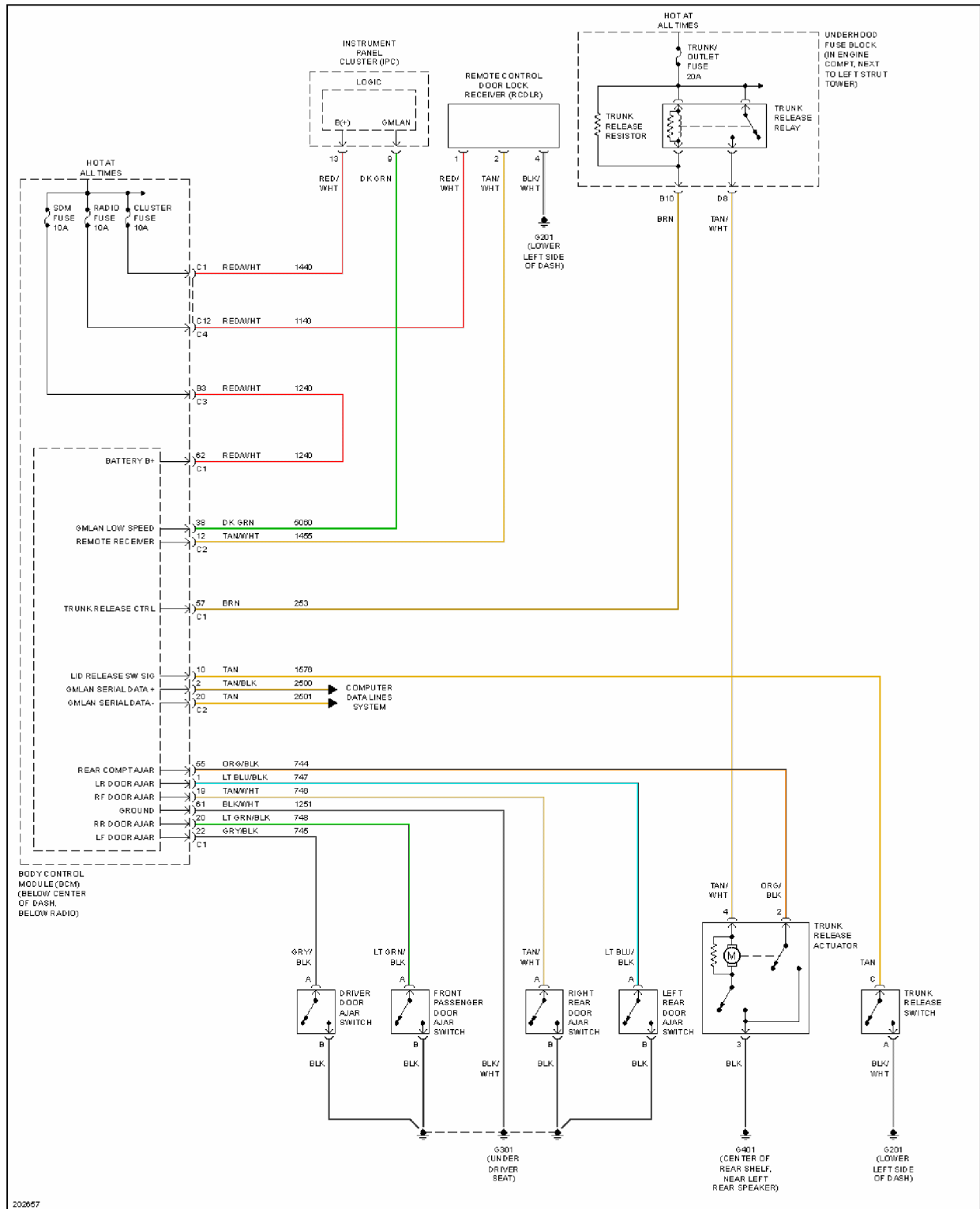
Fig. 43: Power Door Locks Circuit (1 of 2)
