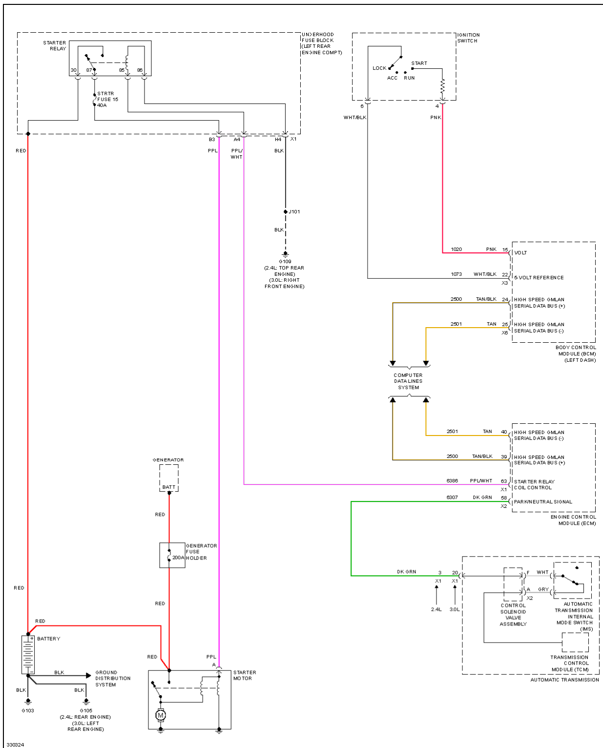
Fig. 72: Starting Circuit
