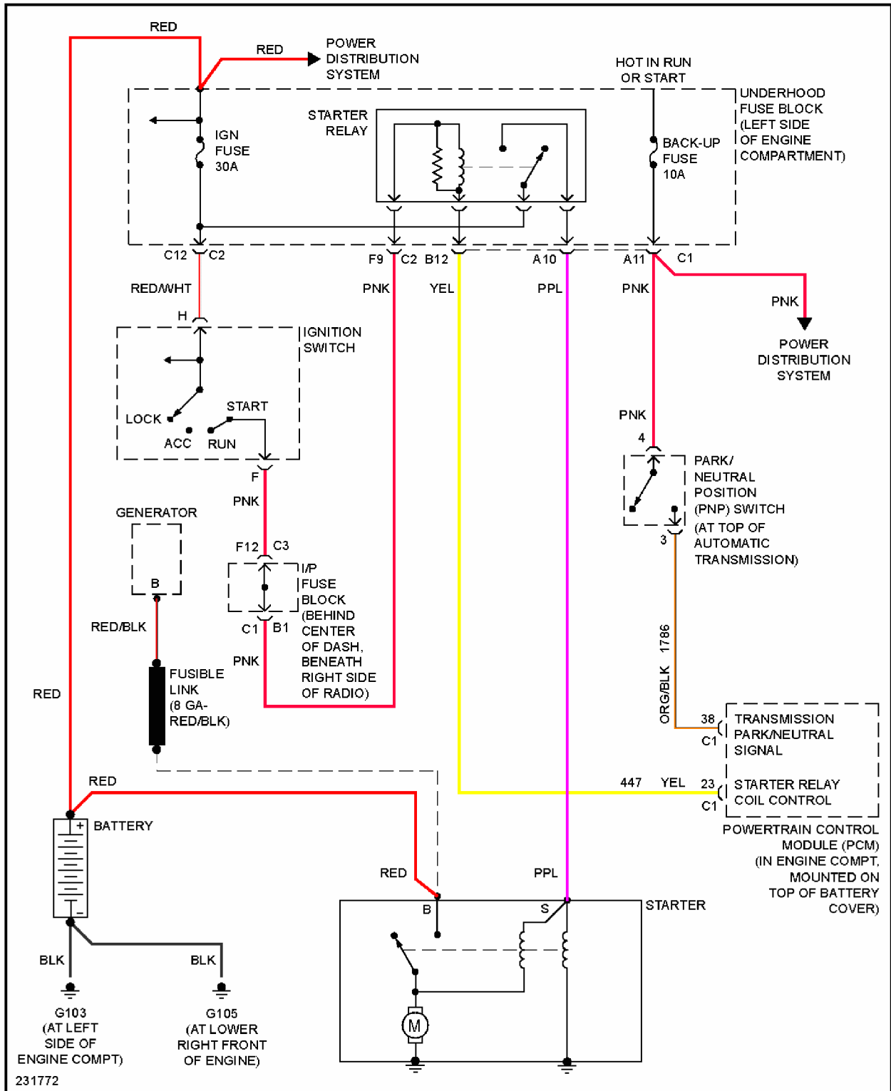
Fig. 43: Starting Circuit
