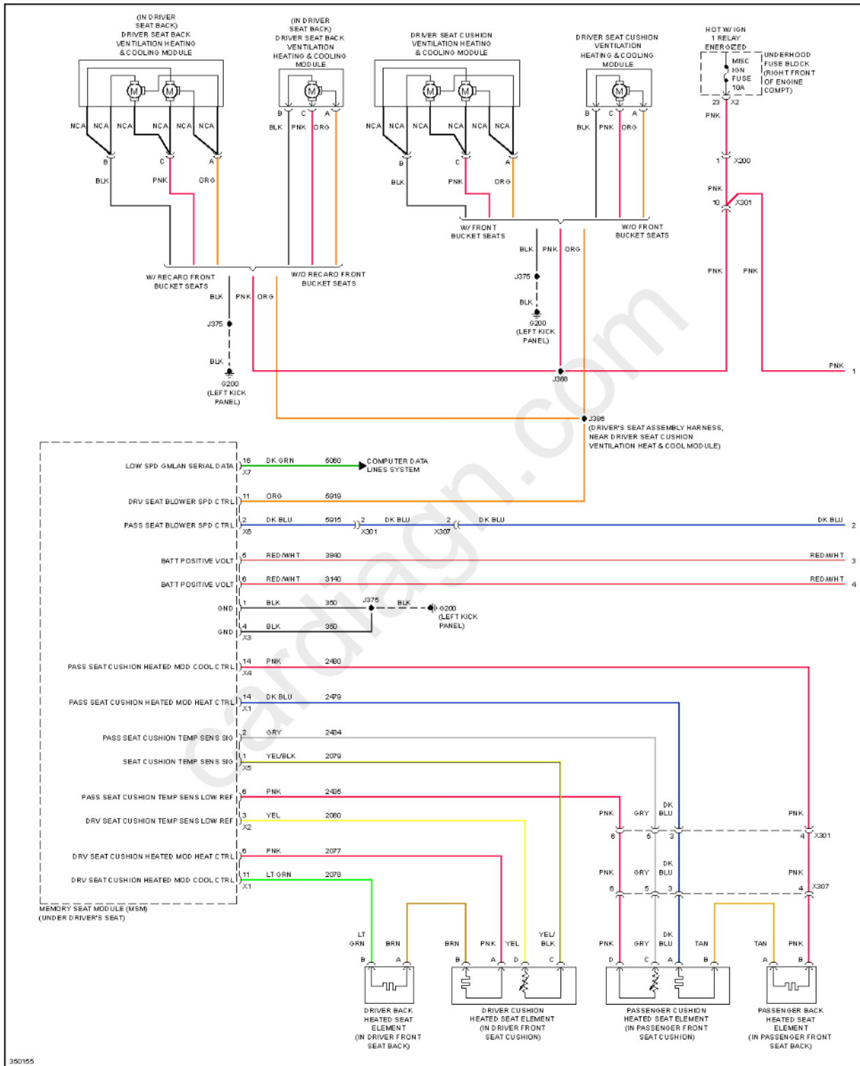
Fig. 90: Heated Seats Circuit (1 of 2)
