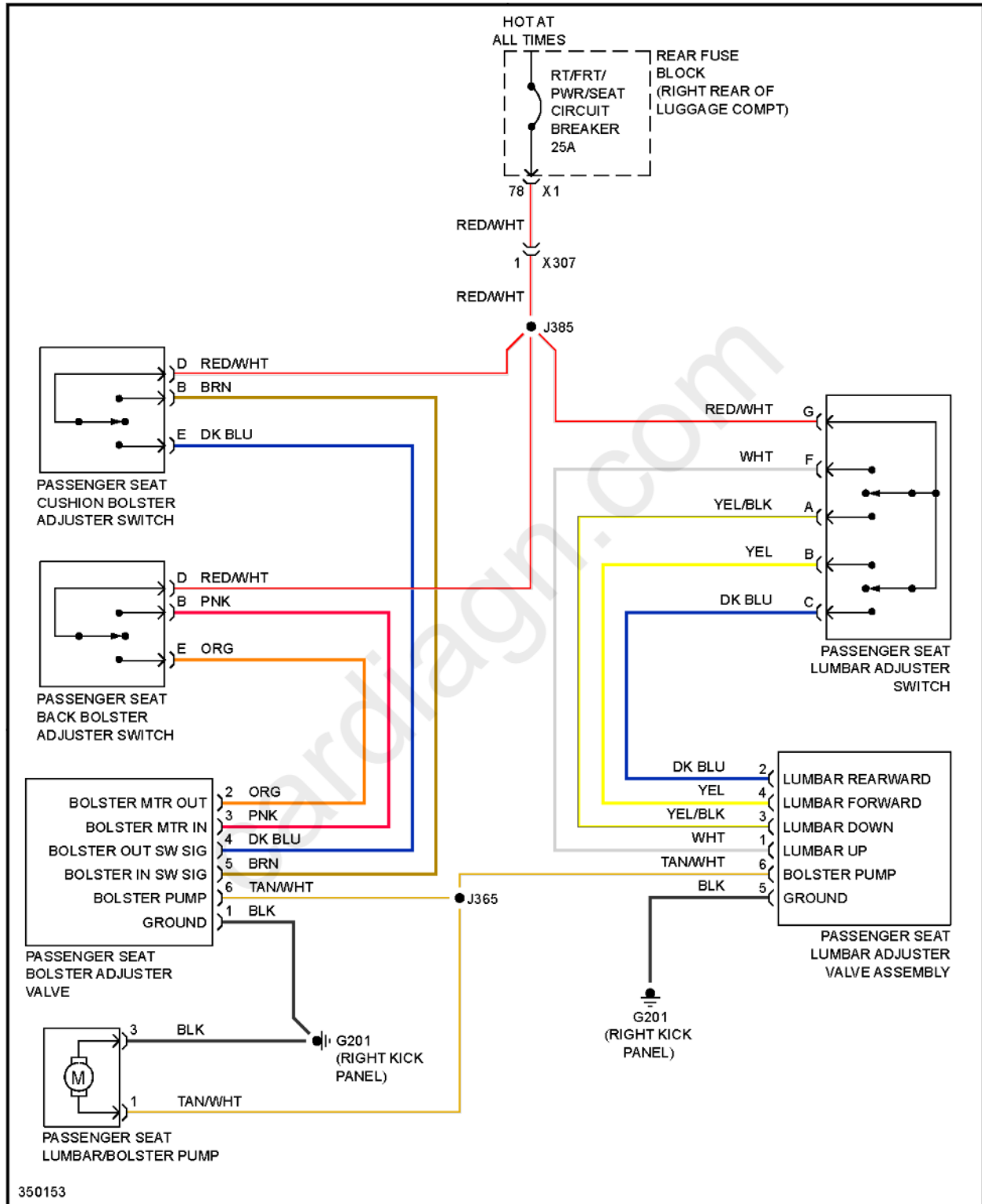
Fig. 94: Passenger's Lumbar Circuit, W/ Recaro Front Bucket Seat
