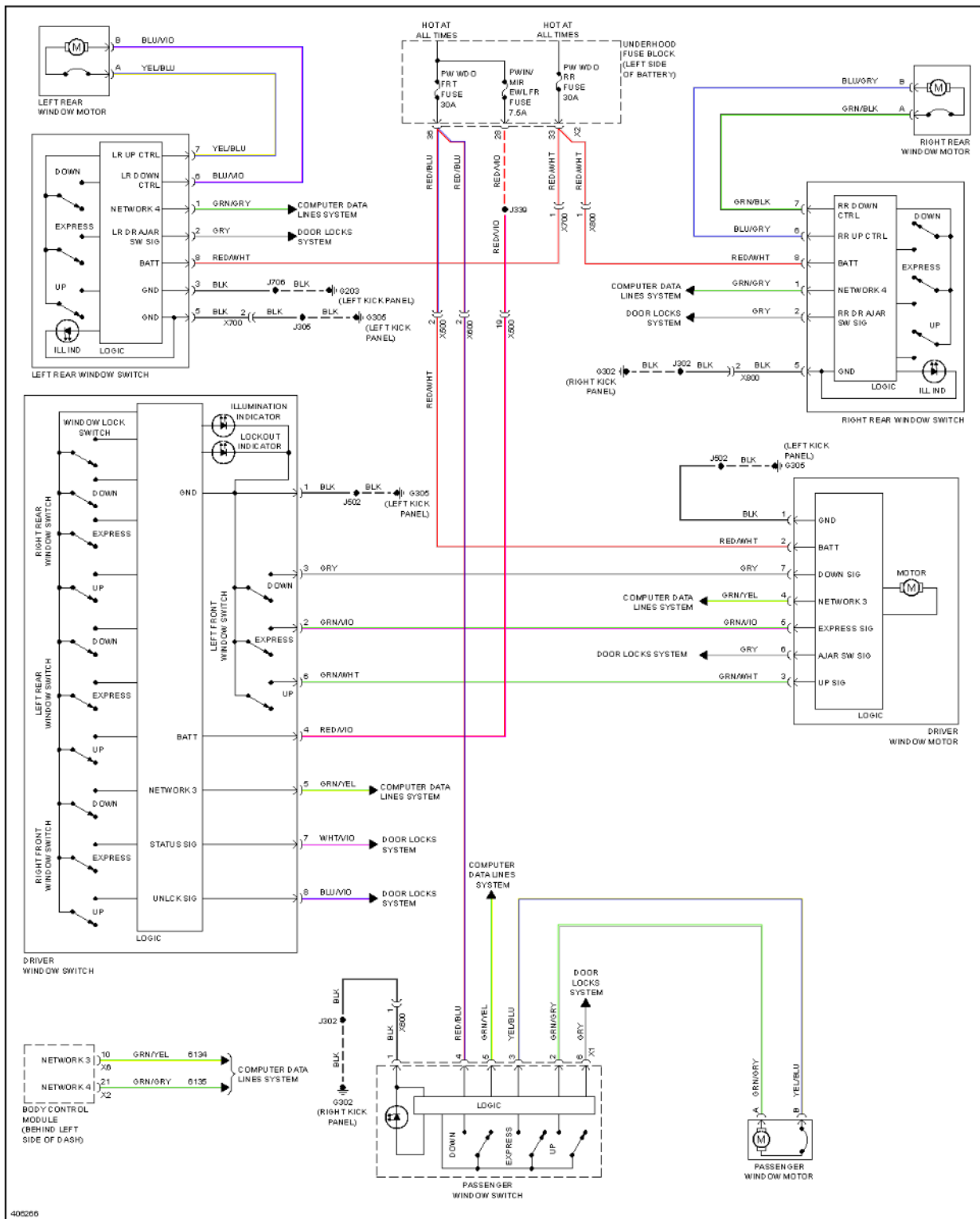
Fig. 111: Power Windows Circuit, W/ Express Up/Down
