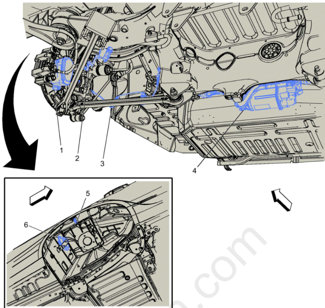
Fig. 4: Right Rear Wheelwell and Rear Axle Components
