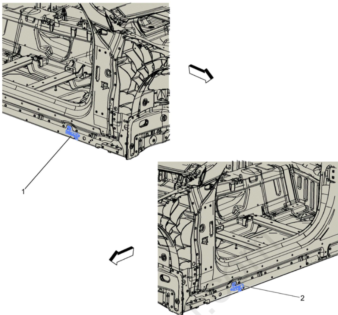
Fig. 2: Rocker Panel Components
