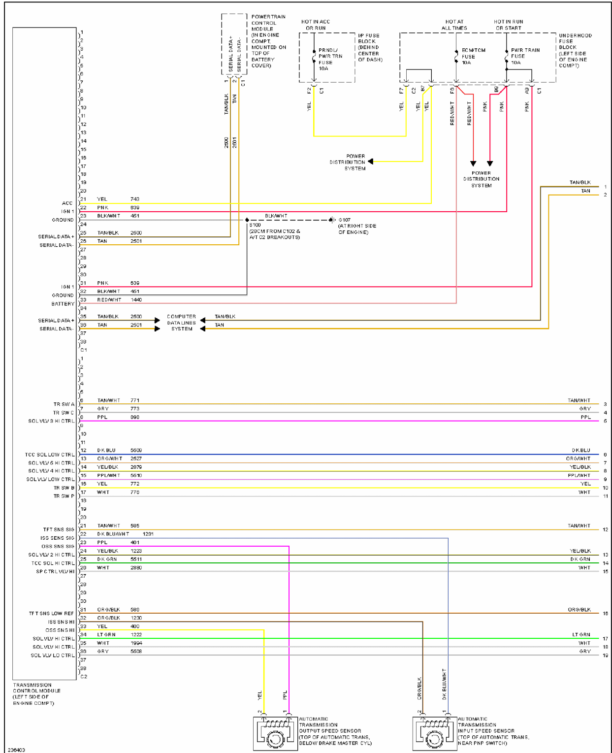
Fig. 45: A/T Circuit (1 of 2)
