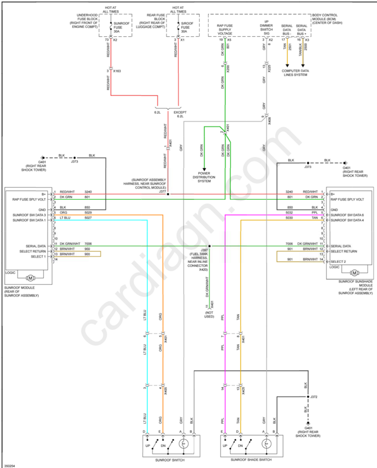
Fig. 96: Power Top/Sunroof Circuit, Coupe
