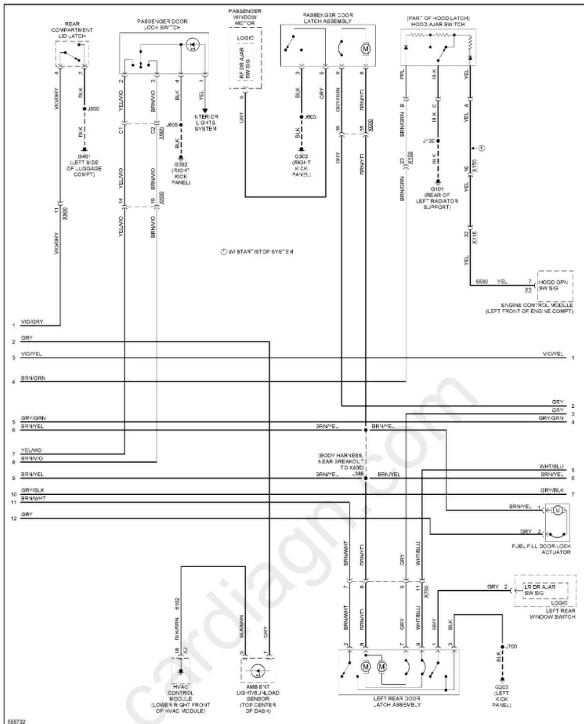
Fig. 16: Forced Entry Circuit, W/O Passive Keyless Entry (2 of 3)
