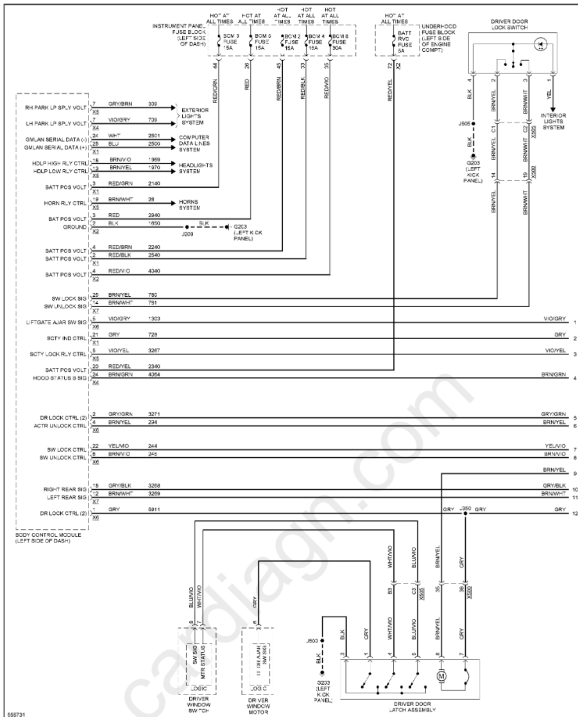
Fig. 15: Forced Entry Circuit, W/O Passive Keyless Entry (1 of 3)
