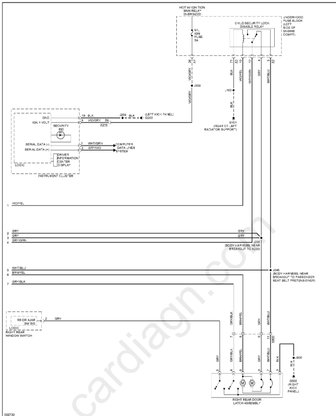
Fig. 17: Forced Entry Circuit, W/O Passive Keyless Entry (3 of 3)
