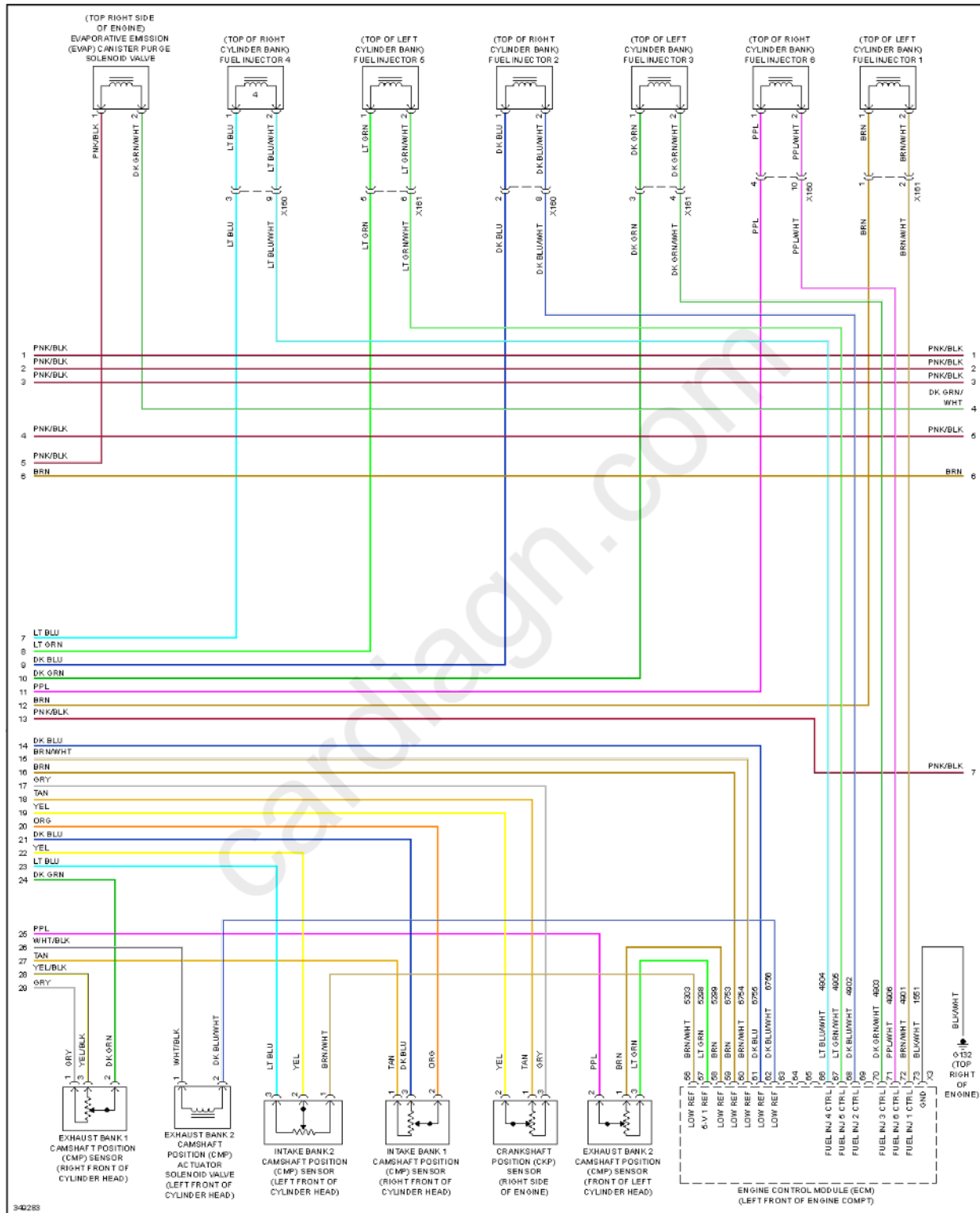
Fig. 29: 3.0L VIN Y, Engine Performance Circuit (4 of 5)
