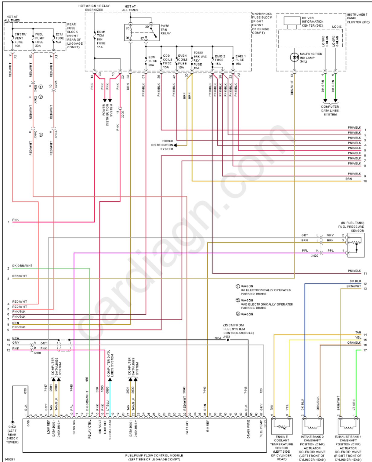
Fig. 27: 3.0L VIN Y, Engine Performance Circuit (2 of 5)
