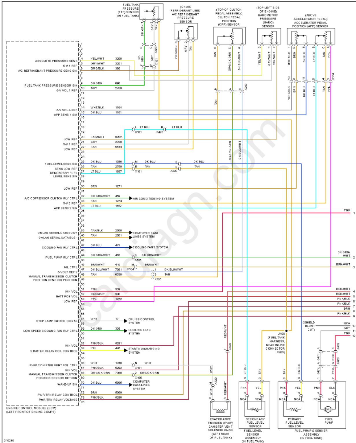
Fig. 26: 3.0L VIN Y, Engine Performance Circuit (1 of 5)
