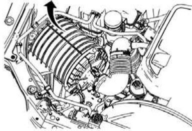
Air Cleaner Element Replacement
