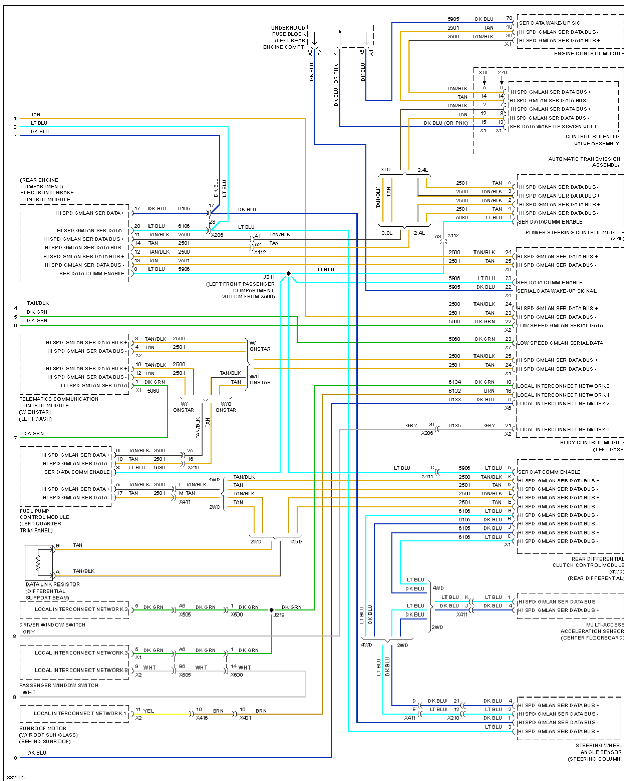
Fig. 13: Computer Data Lines Circuit (2 of 2)
